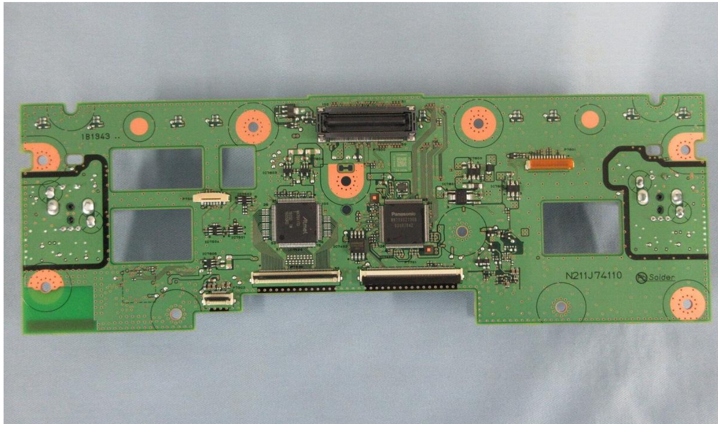
4.PCB-MONI-SW S-side
