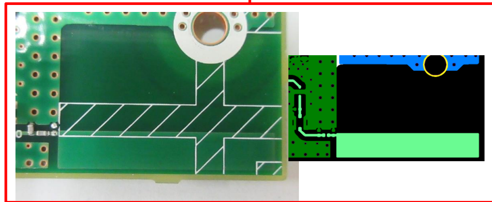
3. PCB-MONI-SW C-side
