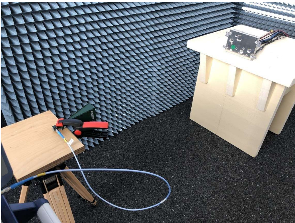
Photograph 21: Radiated emission 18...40 GHz
