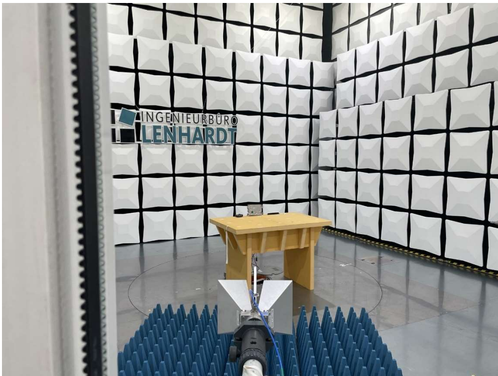
Photograph 20: Radiated emission 1...18 GHz
