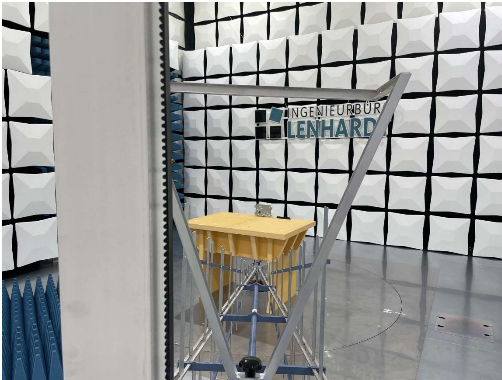
Photograph 17: Radiated emission 30...1000 MHz
