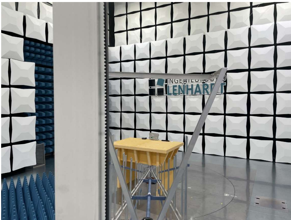
Photograph 18: Radiated emission 30...1000 MHz
