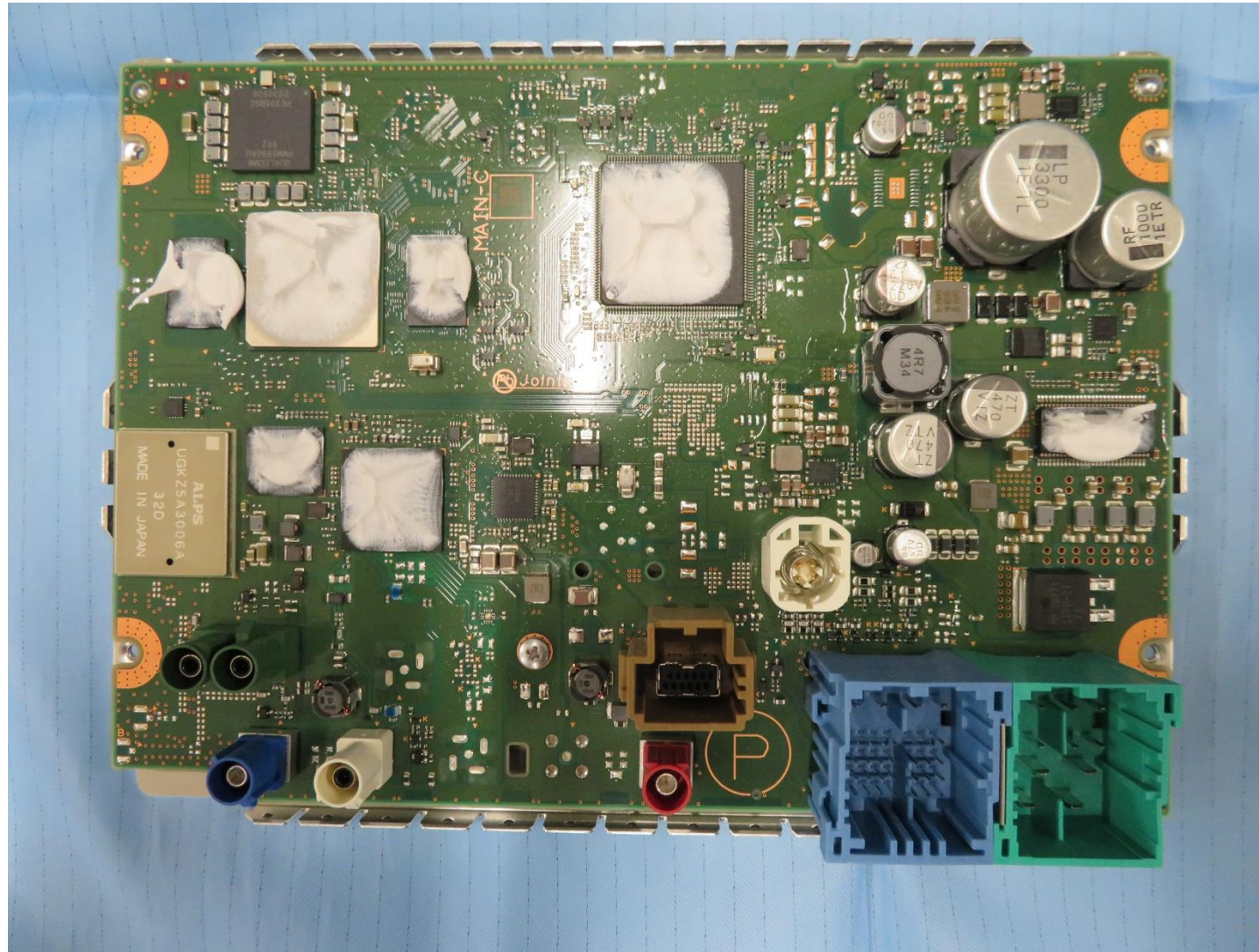
PCB-MAIN C-side
