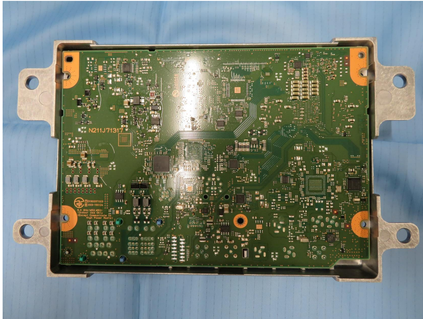
PCB-MAIN S-side
