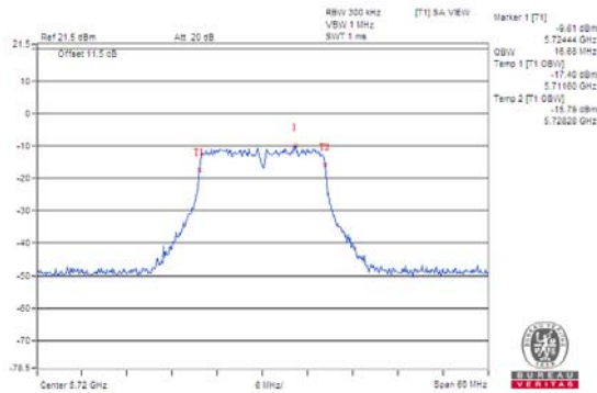
802.11n (HT20) / Chain 0 / CH 144
