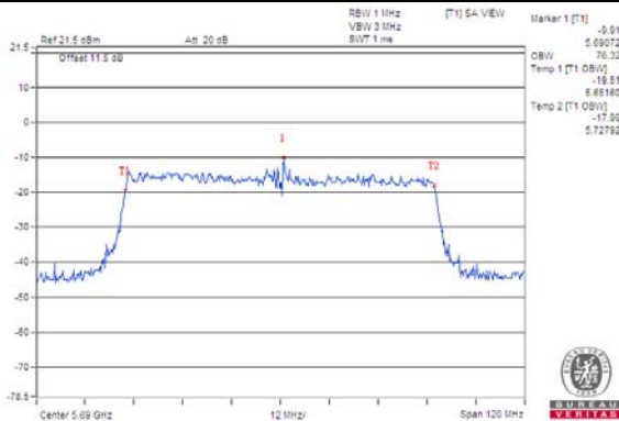
802.11ac (VHT80) / Chain 0 / CH 138
