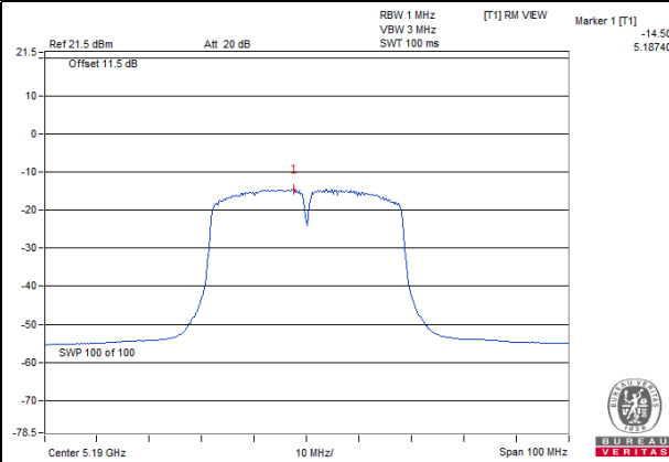
802.11n (HT40) / Chain 0 / CH 38
