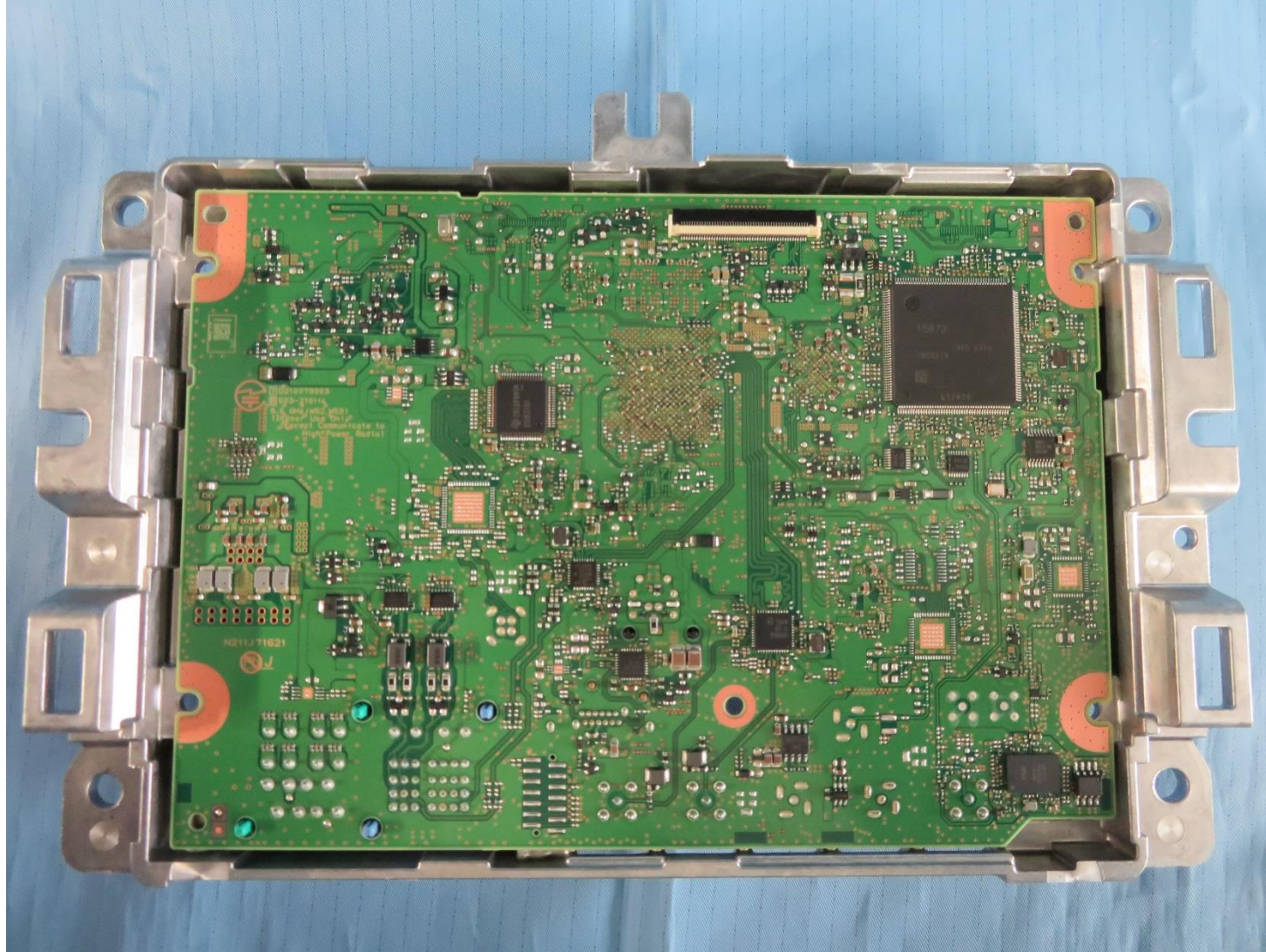
PCB-MAIN S-side
