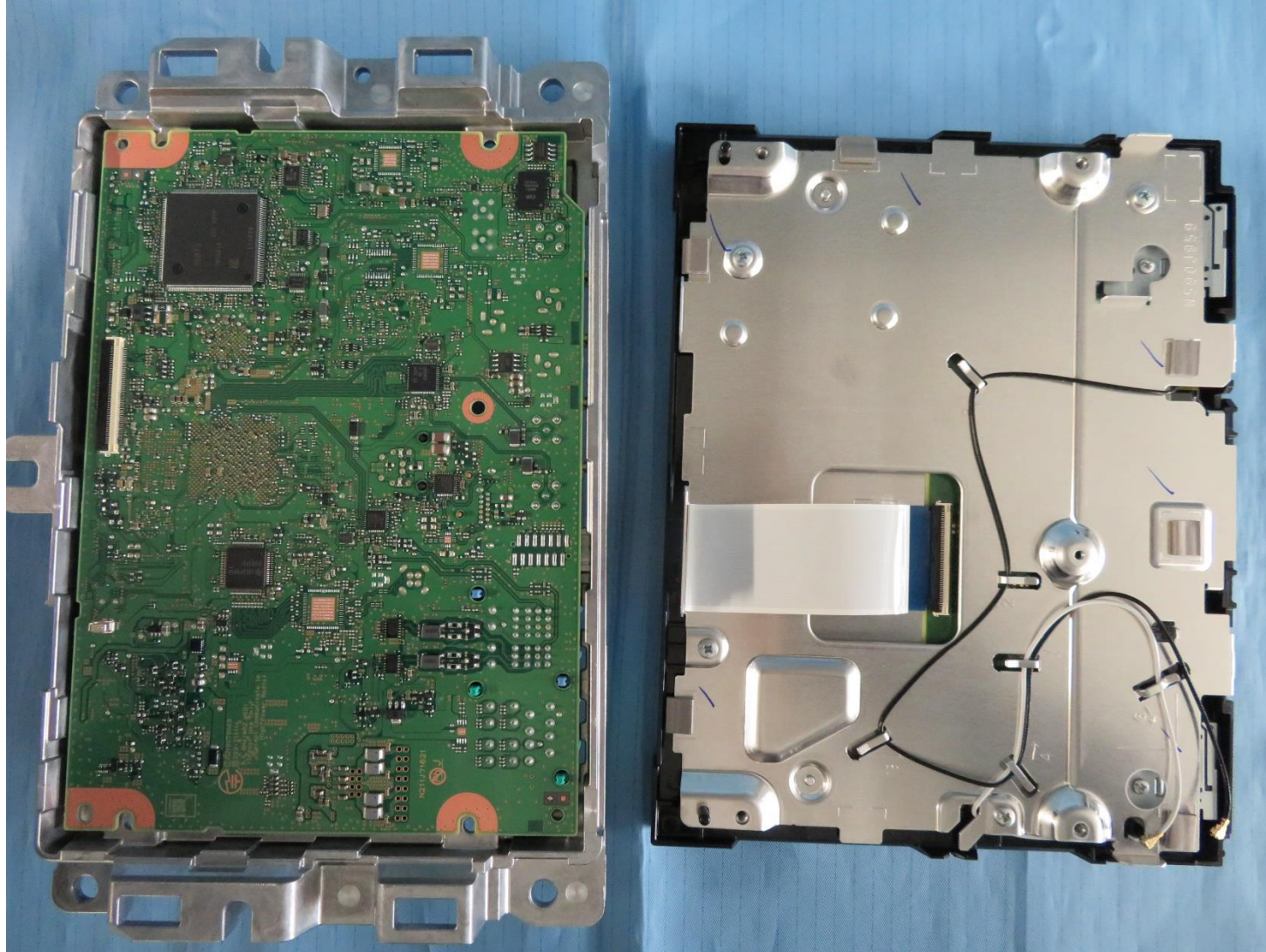
PCB-MAIN S-side
