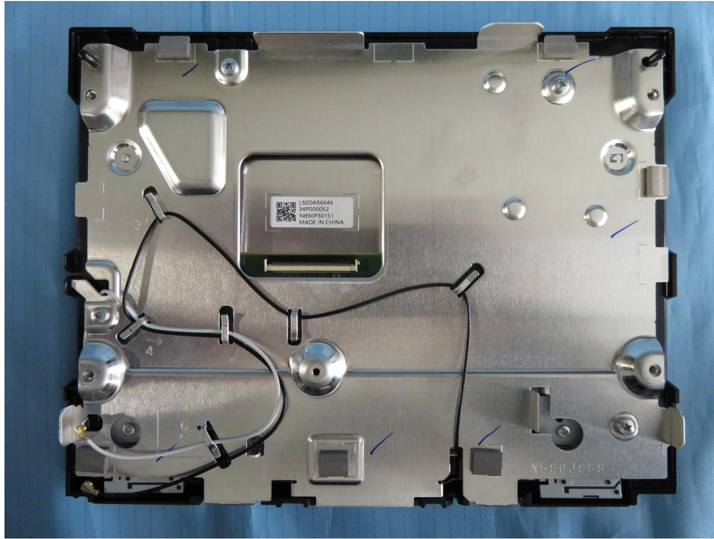
Rear side
