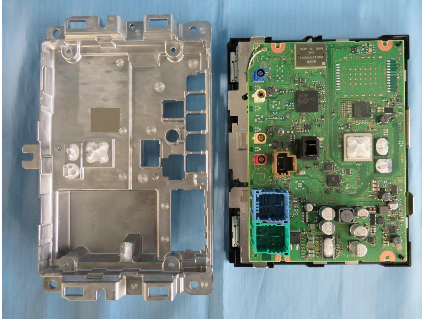
PCB-MAIN C-side
