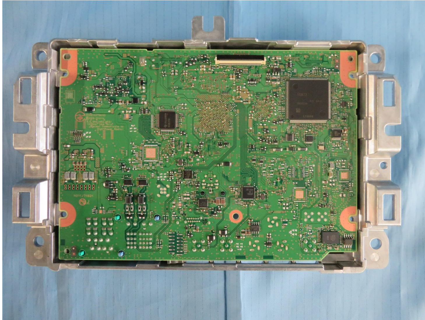
PCB-MAIN S-side
