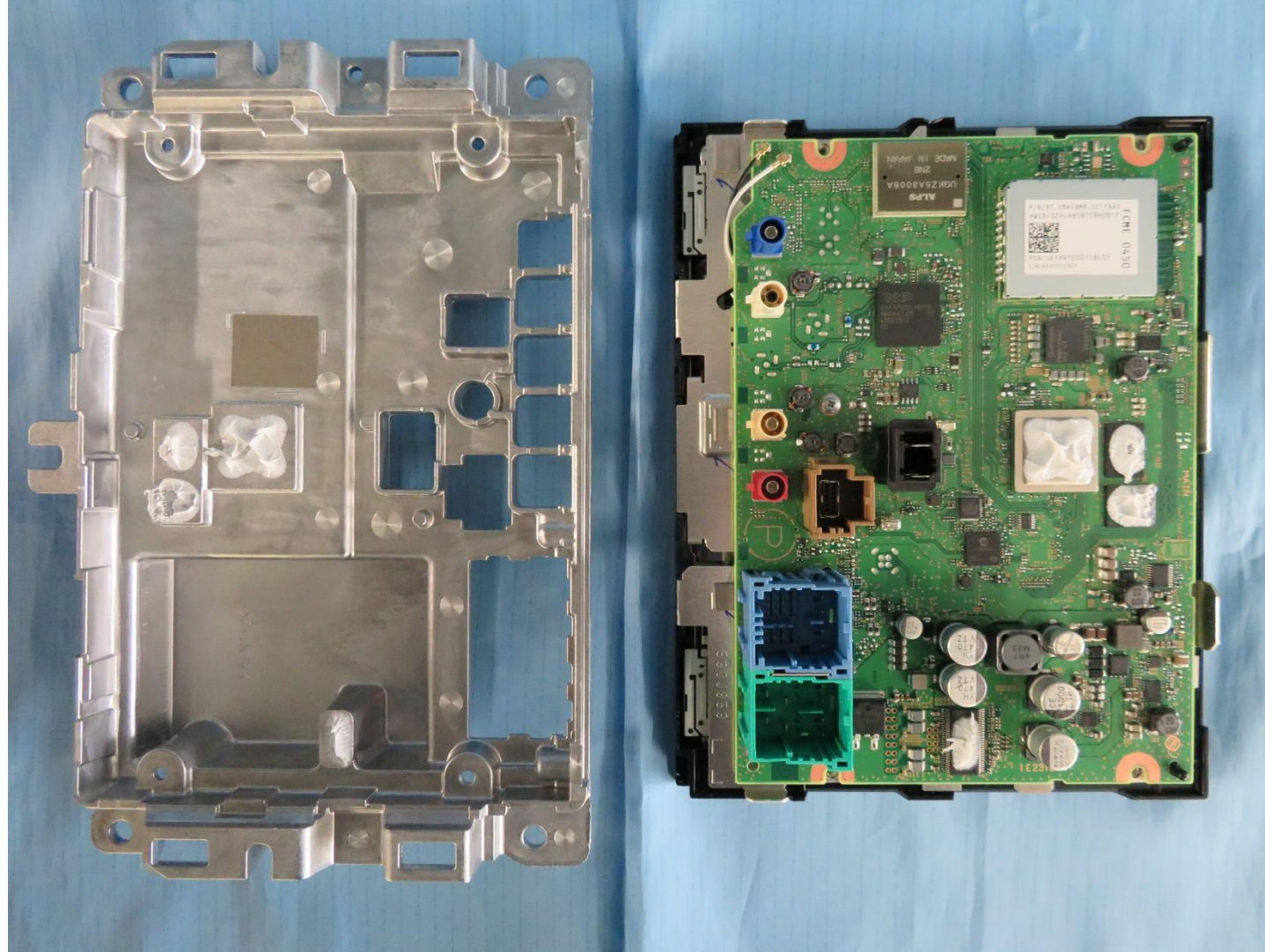
PCB-MAIN C-side
