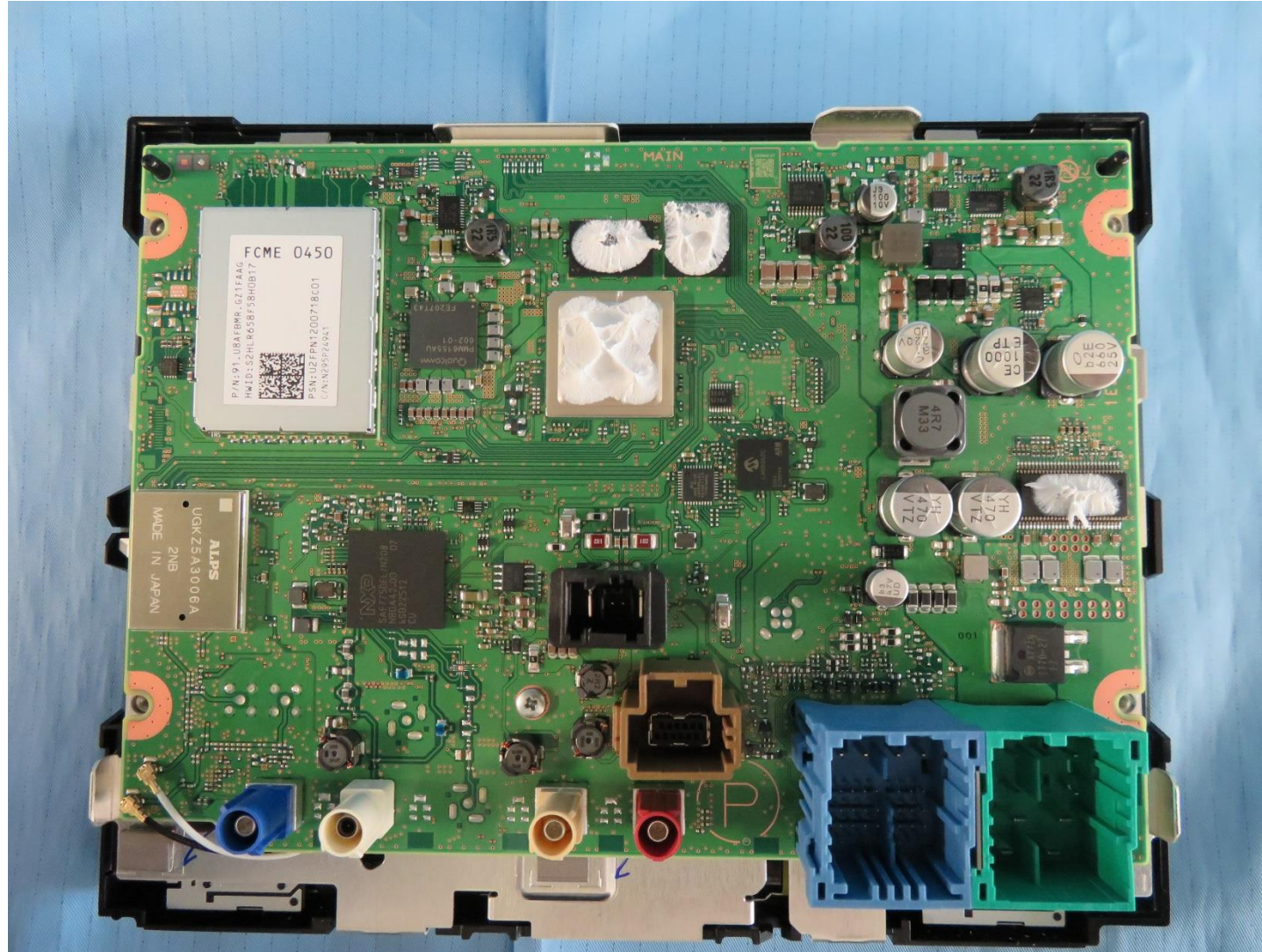
PCB-MAIN C-side
