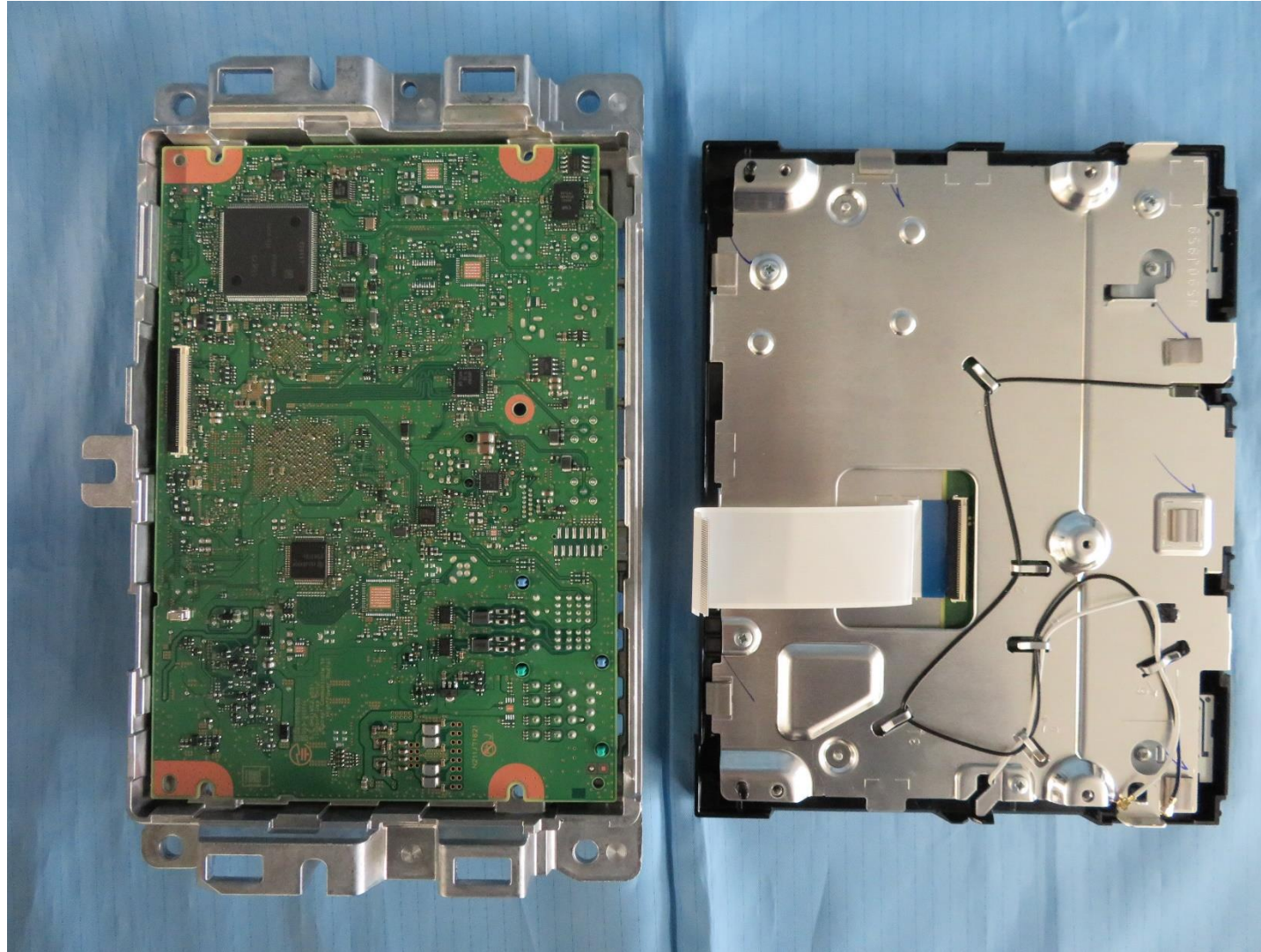
PCB-MAIN S-side
