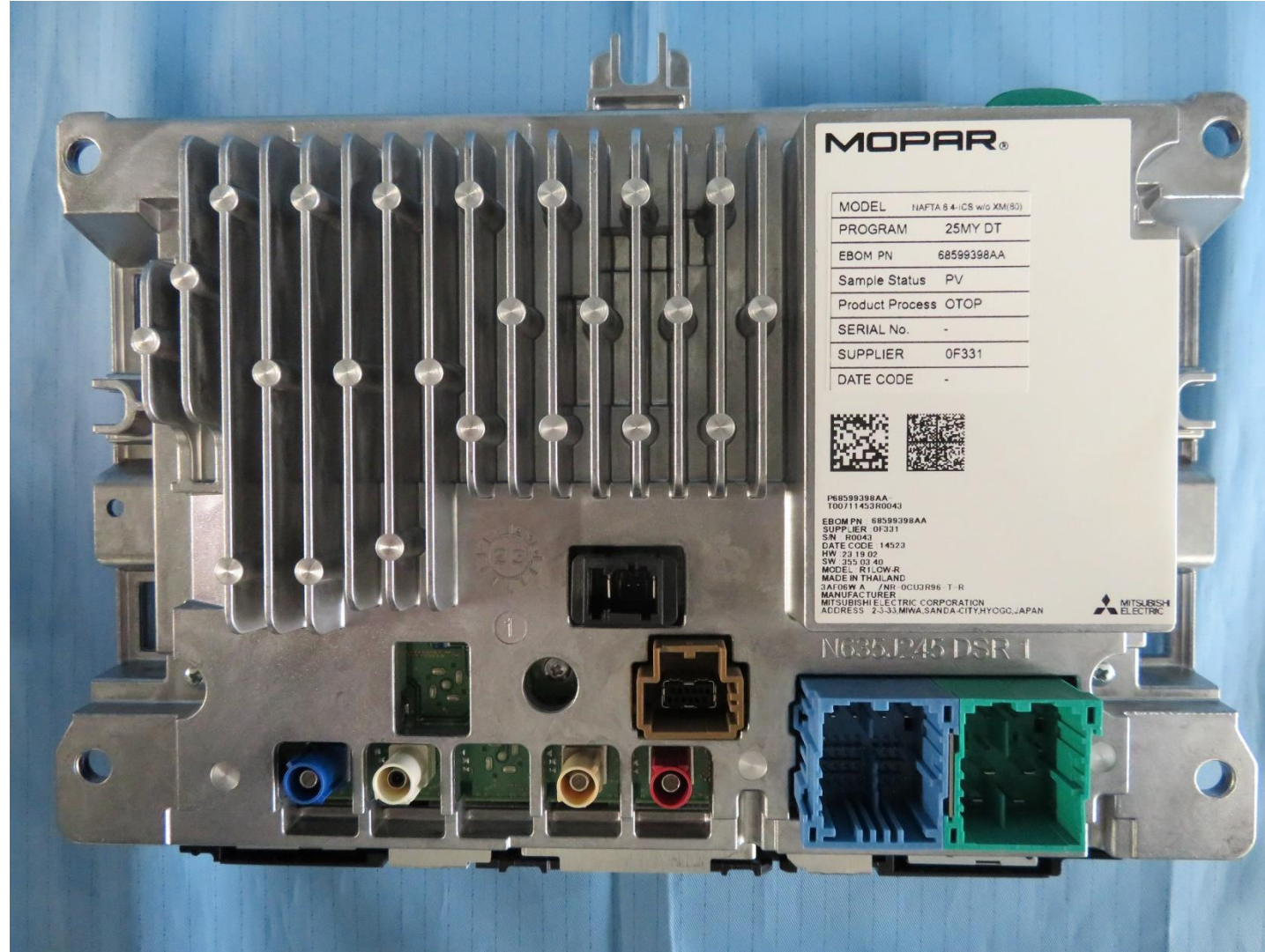
Rear side
