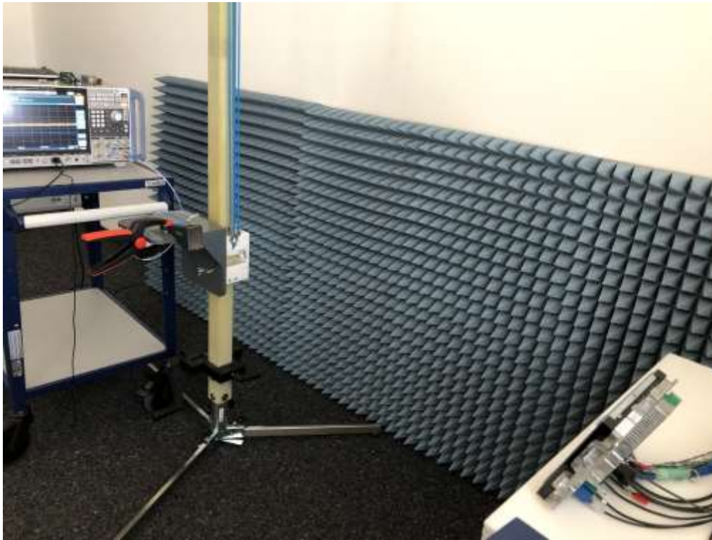
Photograph 33: Radiated emission 18...40 GHz
