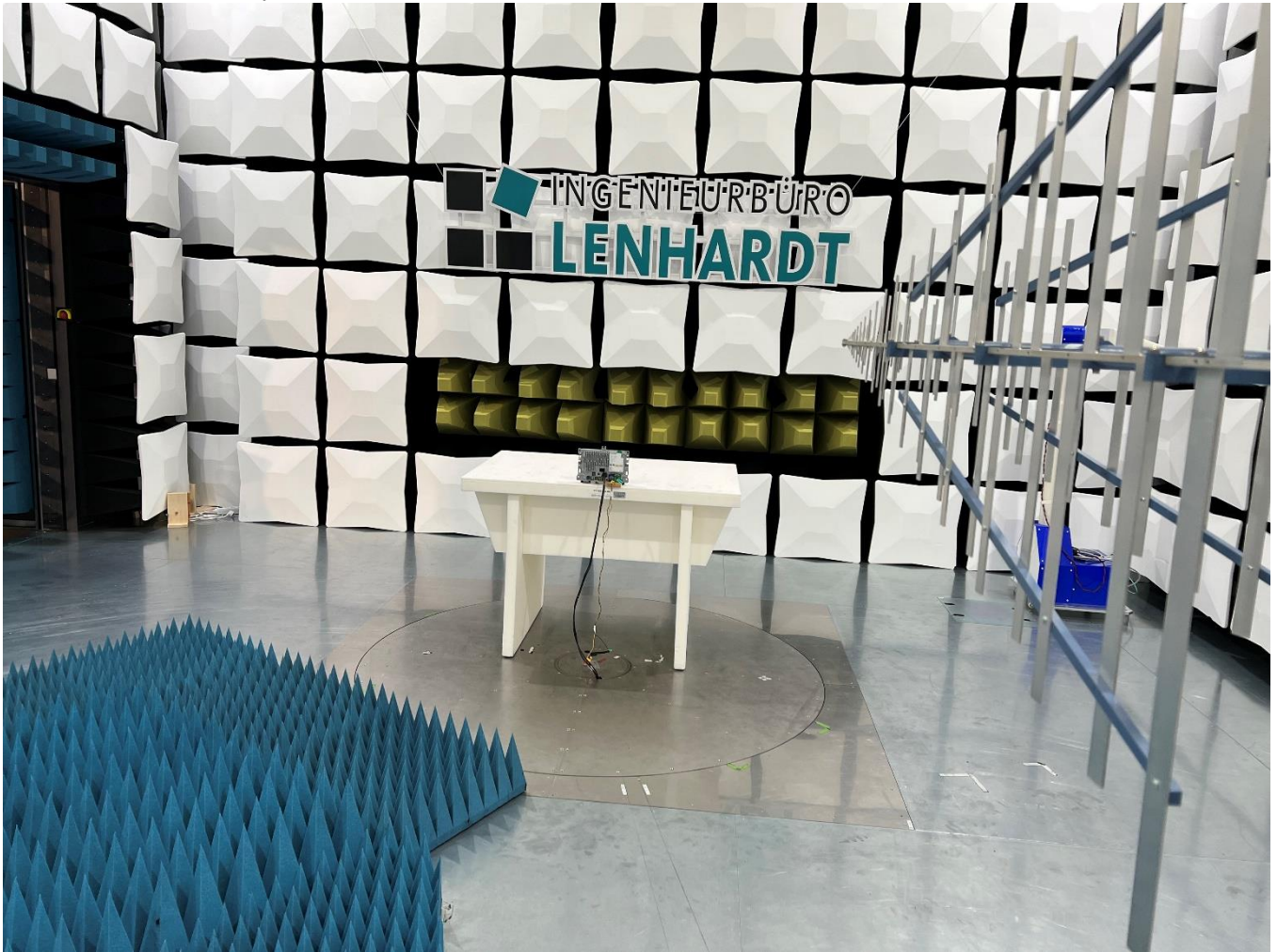
Photo No. 3: Test set-up 8.1, test antenna view
