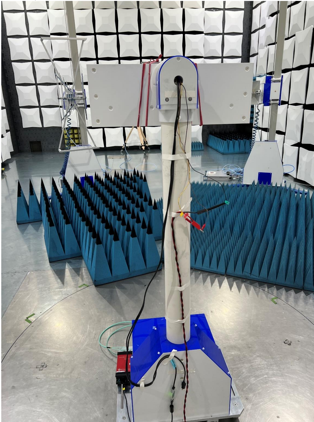
Photo No. 4: Test set-up 8.2, EUT view
