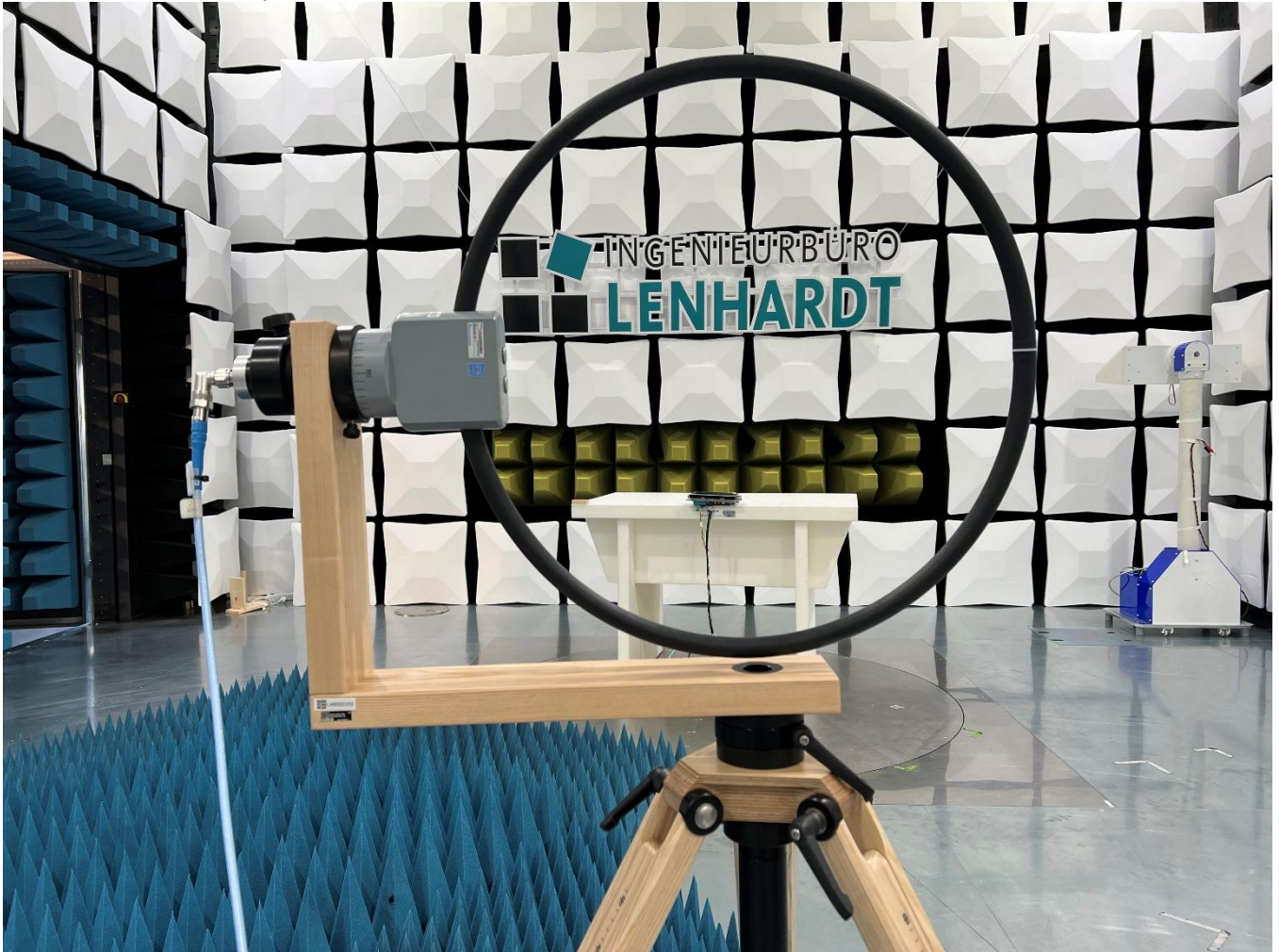
Photo No. 2: Test set-up 8.1, test antenna view
