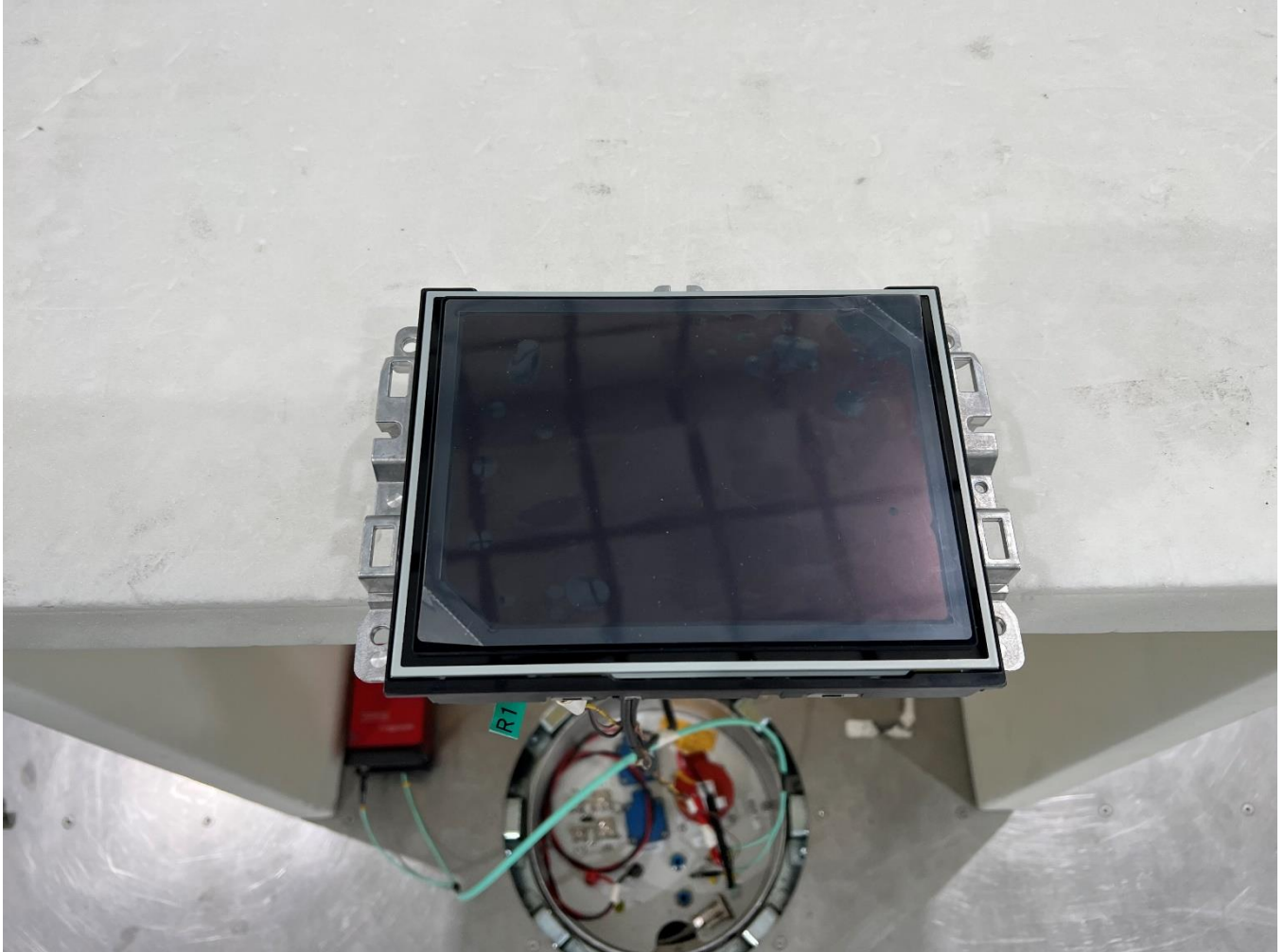
Photo No. 1: Test set-up 8.1, EUT table 0.8 m
