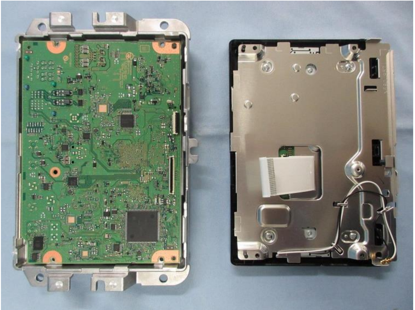
Photo No. 14: PCB-MAIN S-side
