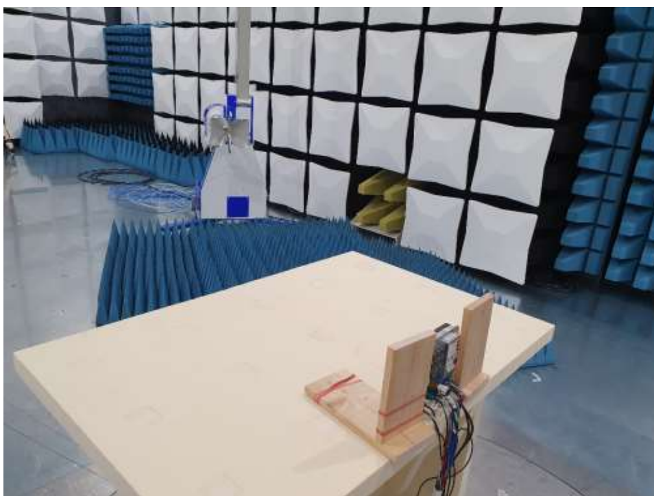
Photograph 23: Radiated emission 1...18 GHz
