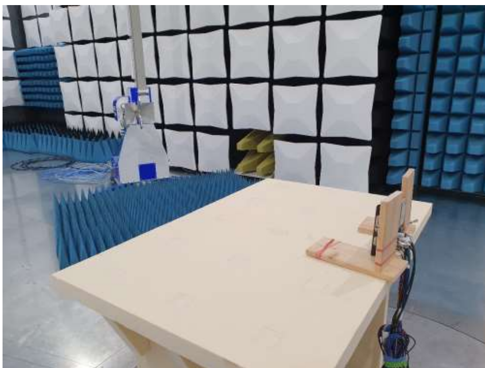
Photograph 14: Radiated emission 1...18 GHz
