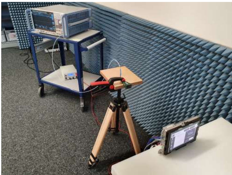
Photograph 27: Radiated emission 18...40 GHz
