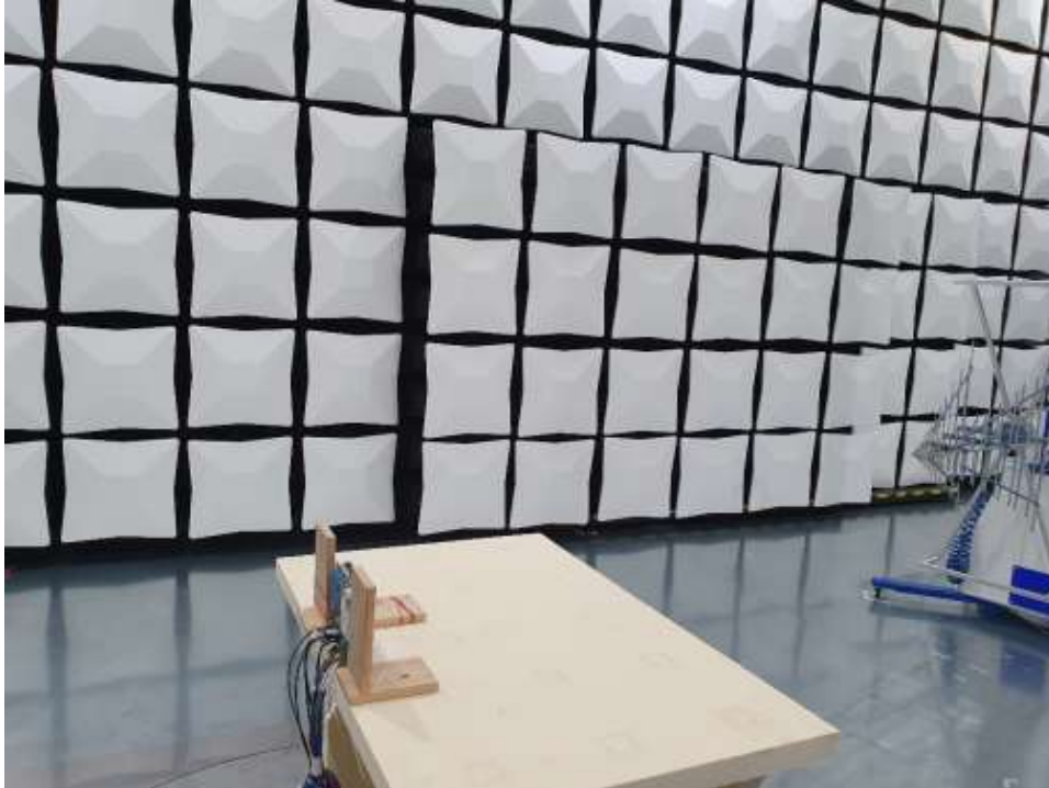
Photograph 16: Radiated emission 30...1000 MHz
