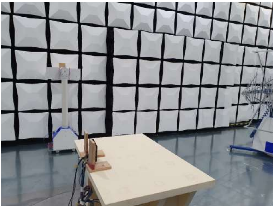
Photograph 25: Radiated emission 30...1000 MHz
