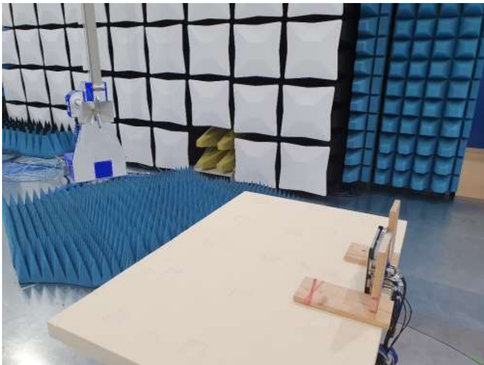
Photograph 17: Radiated emission 1...18 GHz
