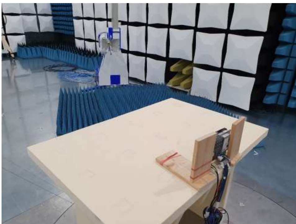
Photograph 11: Radiated emission 1...18 GHz
