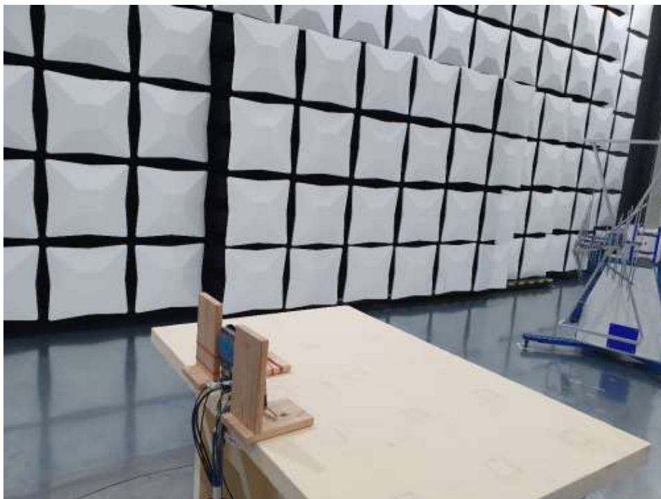
Photograph 28: Radiated emission 30...1000 MHz
