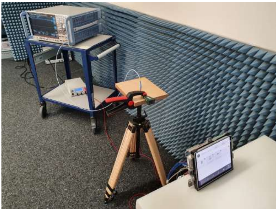
Photograph 15: Radiated emission 18...40 GHz
