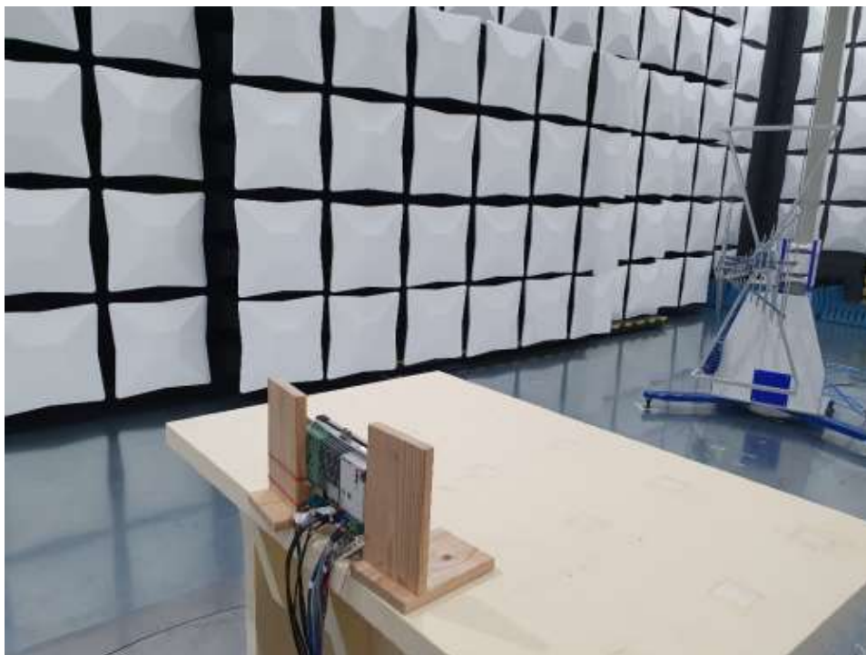
Photograph 13: Radiated emission 30...1000 MHz
