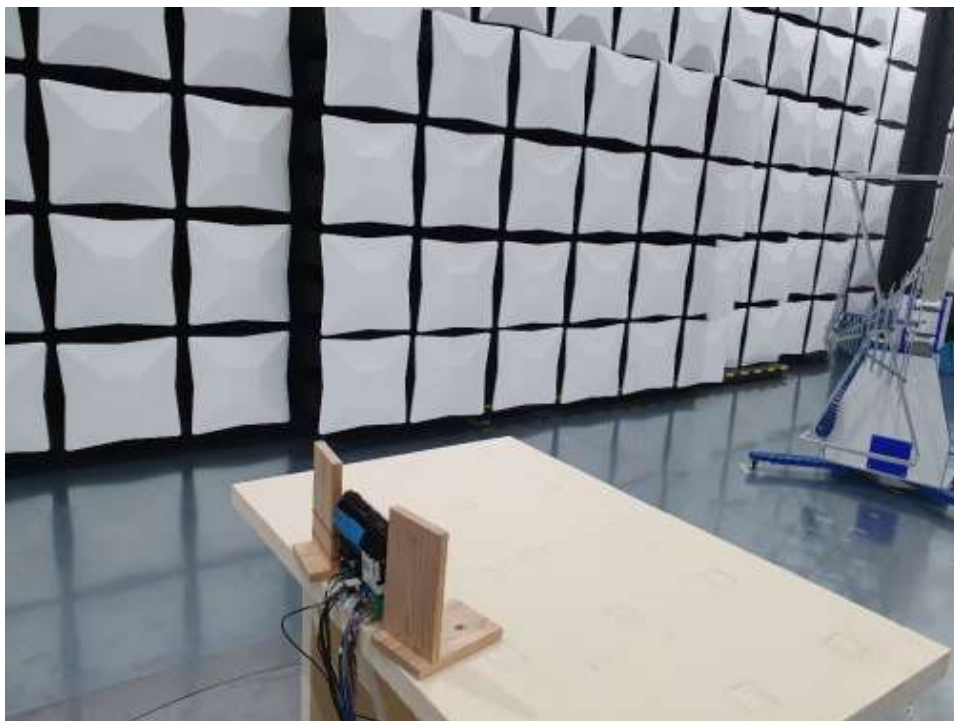
Photograph 1: Radiated emission 30...1000 MHz
