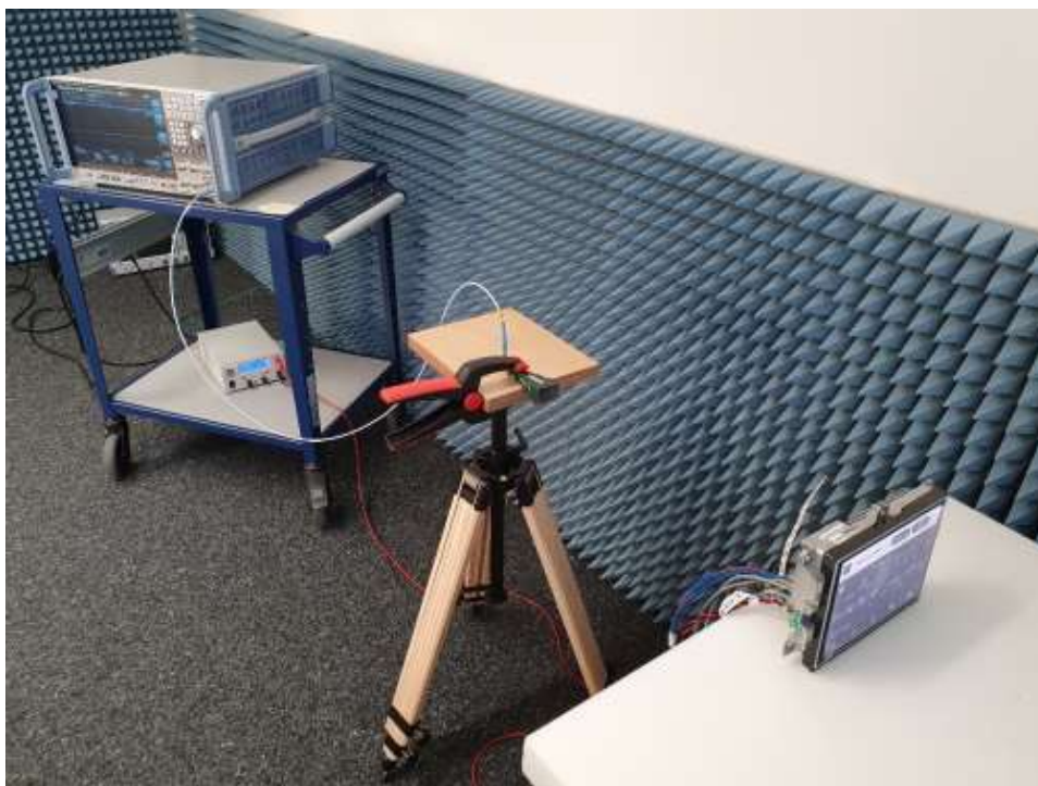
Photograph 12: Radiated emission 18...40 GHz
