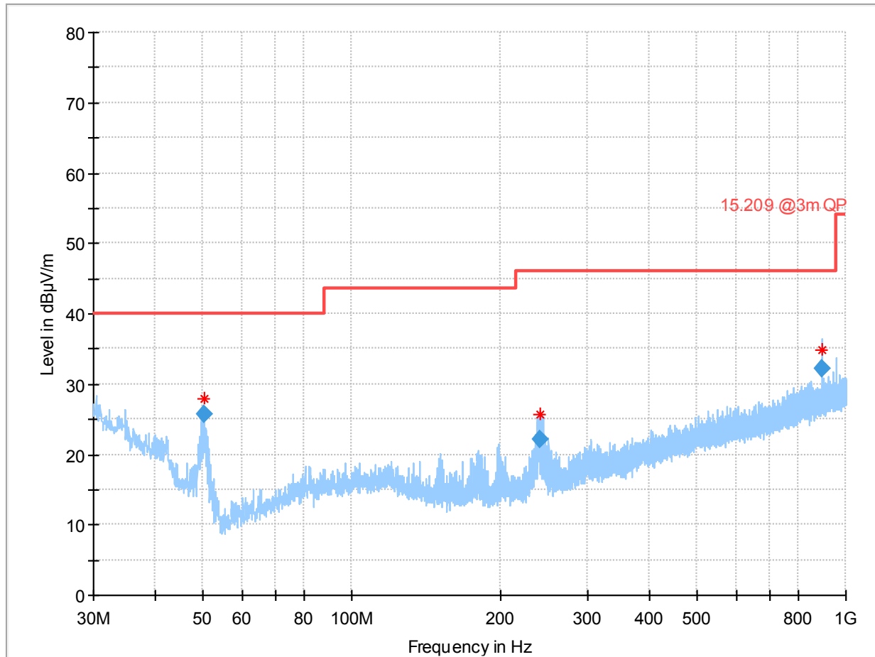
Plot 8: Mode 1, RSE 30 MHz – 1 GHz, channel 165, horizontal / vertical polarisation
