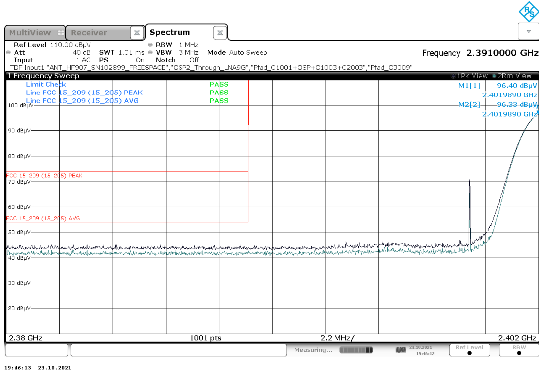
Plot 6: Mode 1, BEC, low channel 37
