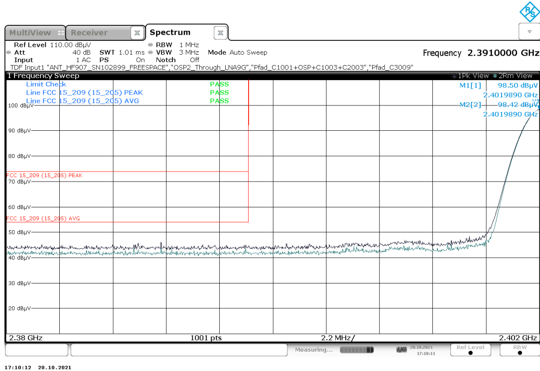
Plot 22: Mode 1, BEC, low channel 37
