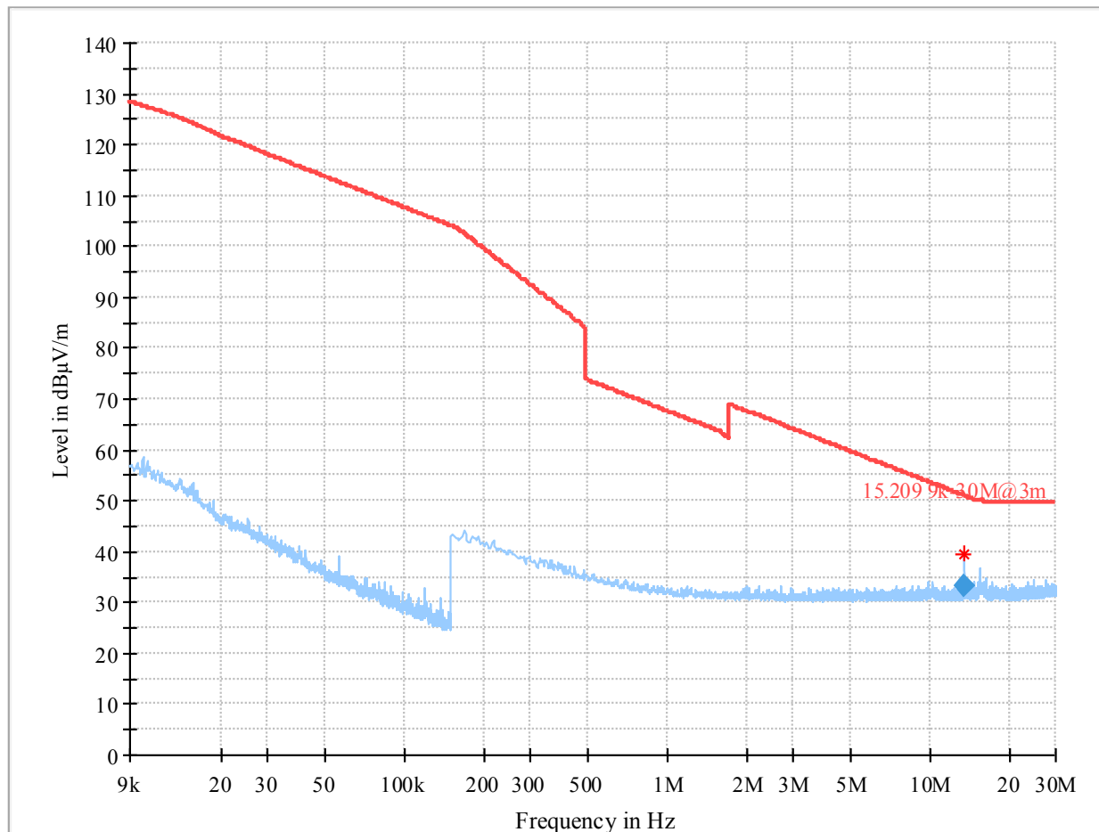
Plot 50: Mode 1, RSE 9 kHz – 30 MHz, high channel, loop antenna
