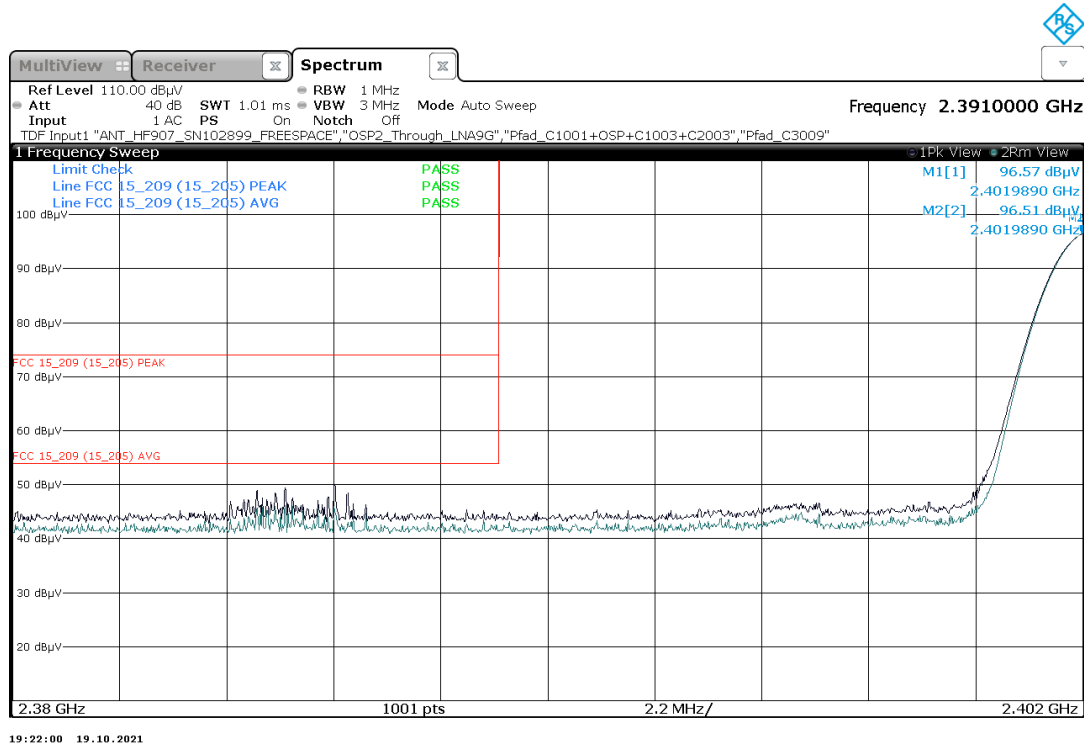
Plot 42: Mode 1, BEC, low channel 37, 2402 MHz
