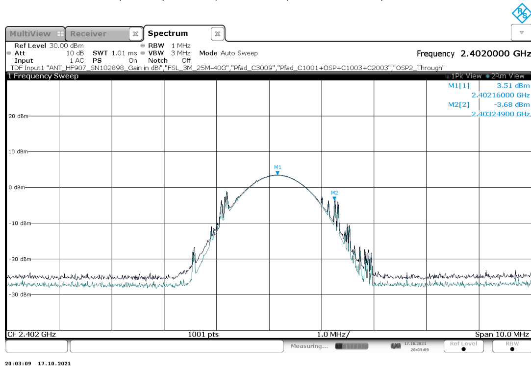
Plot 3: Test Mode 1, GFSK, 1 Mbit/s, Peak EIRP, low channel 37, 2402 MHz
