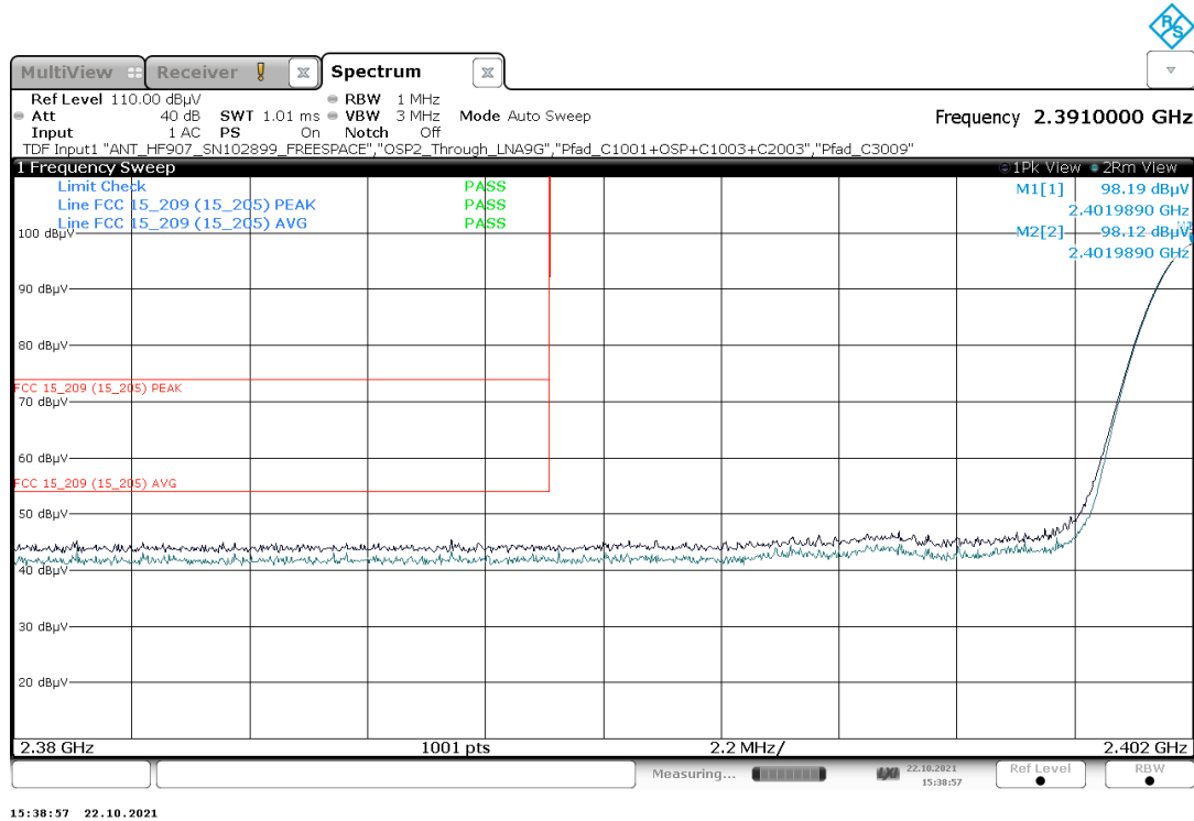
Plot 14: Mode 1, BEC, low channel 37
