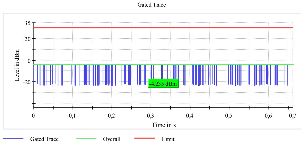
Plot 38: Test Mode 1, GFSK, 1 Mbit/s, RF output power, high channel 39, 2480 MHz
