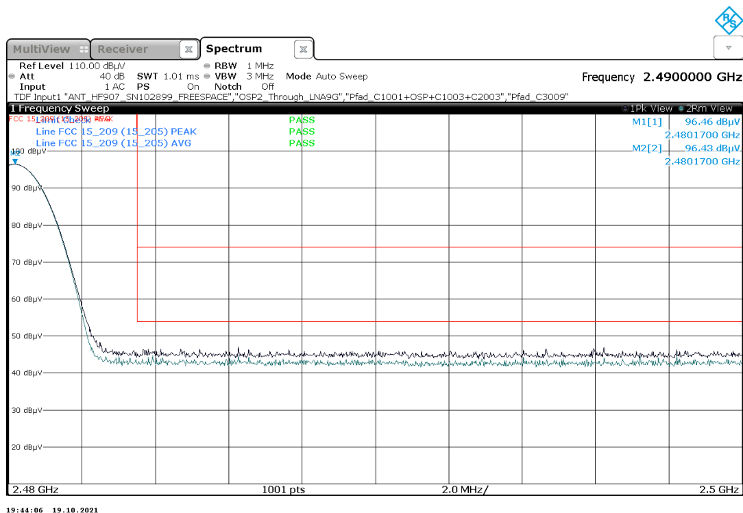
Plot 43: Mode 1, BEC, high channel 39, 2480 MHz
