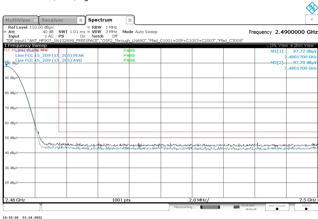
Plot 7: Mode 1, BEC, high channel 39
