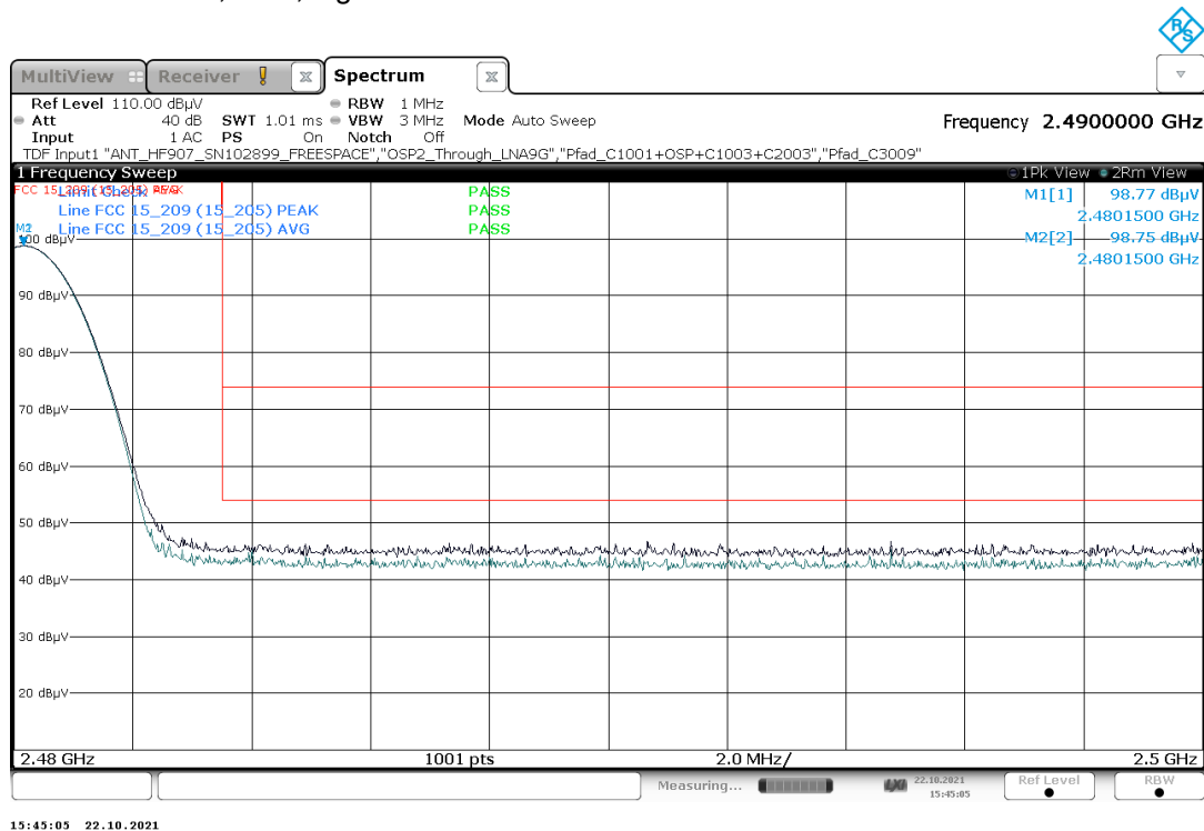
Plot 15: Mode 1, BEC, high channel 39
