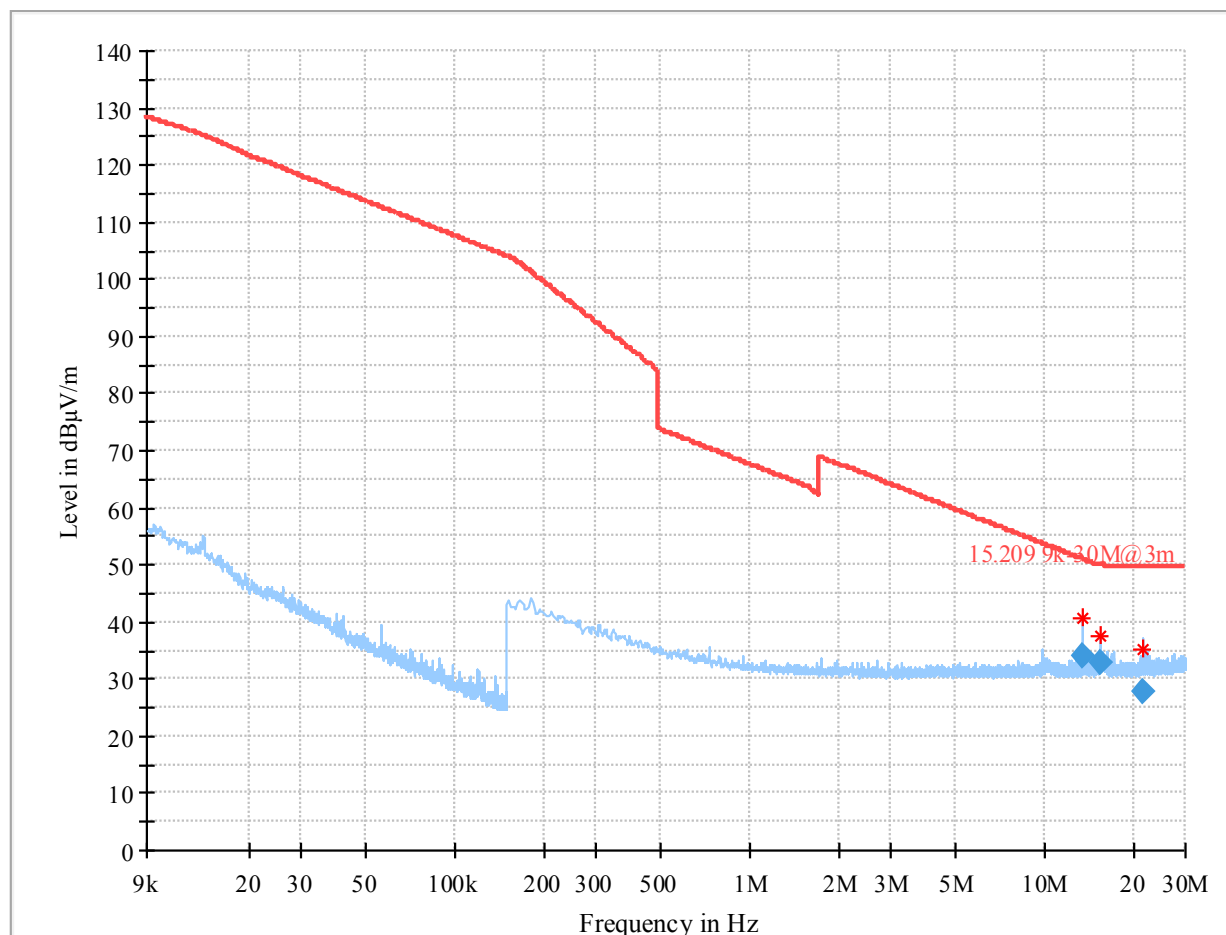
Plot 24: Mode 1, RSE 9 kHz – 30 MHz, low channel, loop antenna
