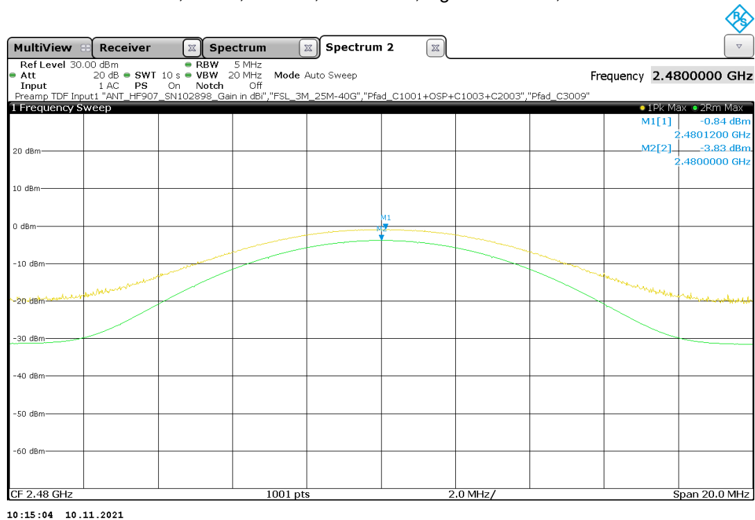
Plot 21: Test Mode 1, GFSK, 1 Mbit/s, Peak EIRP, high channel 39, 2480 MHz
