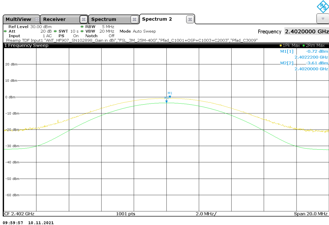
Plot 19: Test Mode 1, GFSK, 1 Mbit/s, Peak EIRP, low channel 37, 2402 MHz
