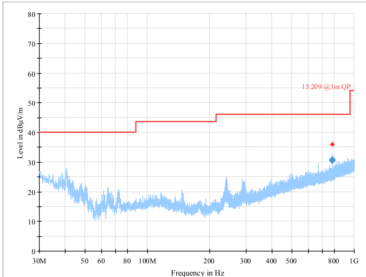
Plot 45: Mode 1, RSE 30 MHz – 1 GHz, low channel, horizontal / vertical polarisation
