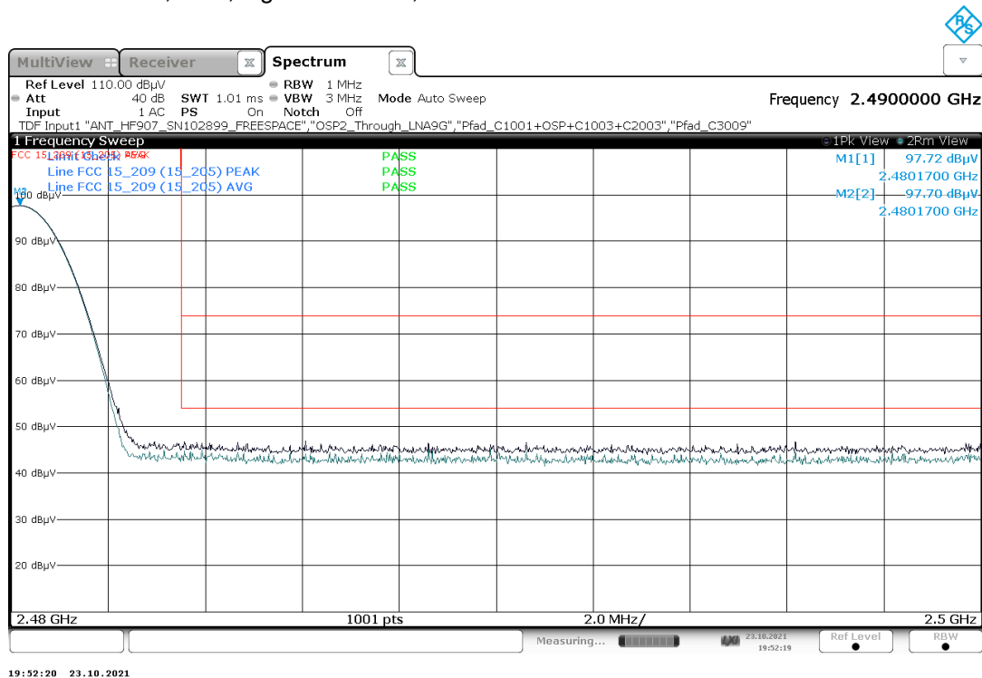
Plot 2: Mode 1, BEC, high channel 39, 2480 MHz
