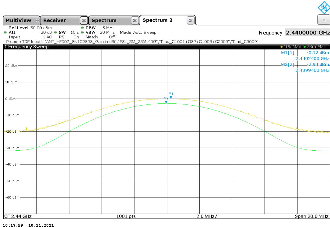
Plot 20: Test Mode 1, GFSK, 1 Mbit/s, Peak EIRP, mid channel 17, 2440 MHz
