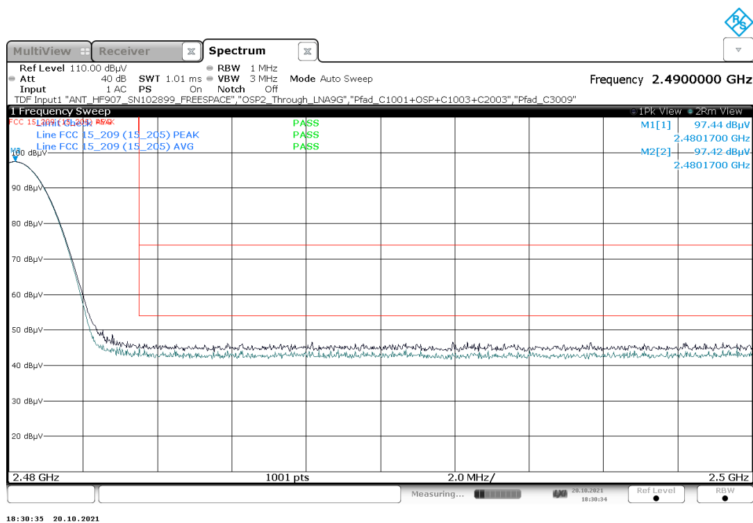
Plot 23: Mode 1, BEC, high channel 39
