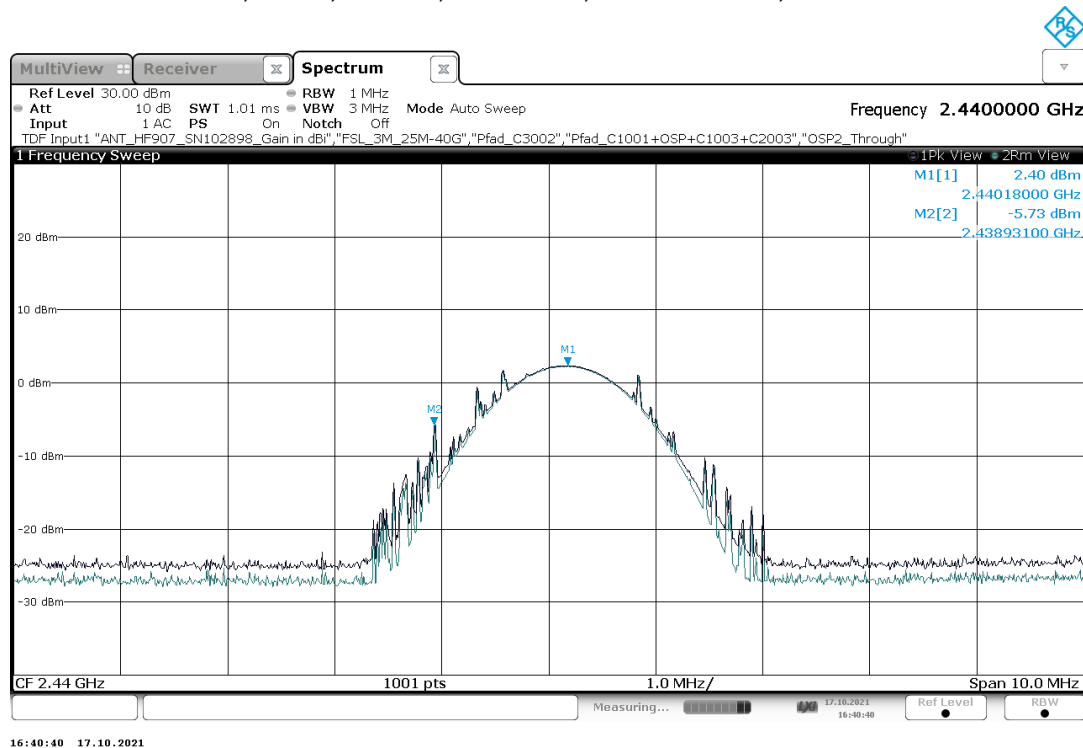
Plot 4: Test Mode 1, GFSK, 1 Mbit/s, Peak EIRP, mid channel 17, 2440 MHz
