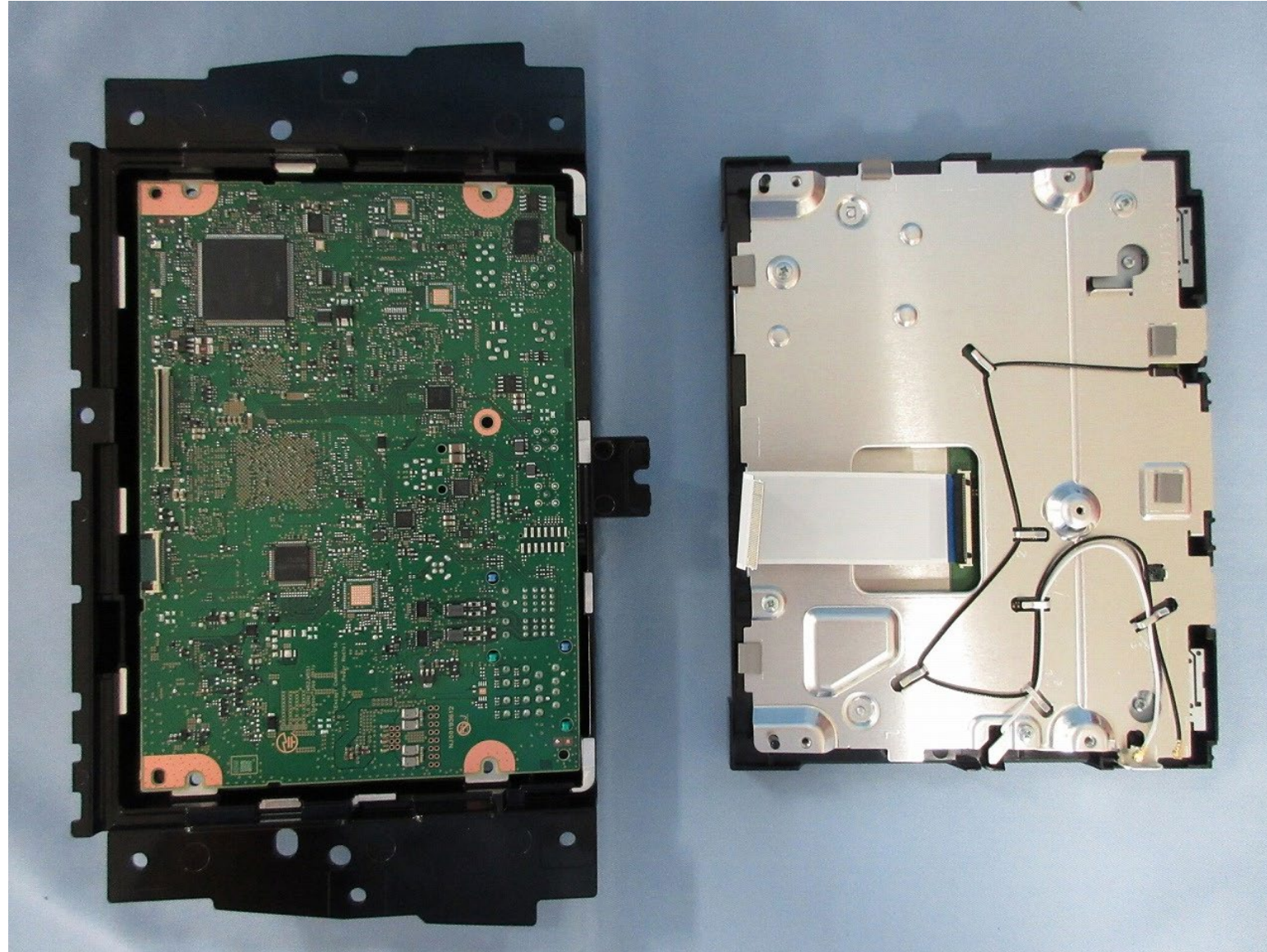
PCB-MAIN S-side
