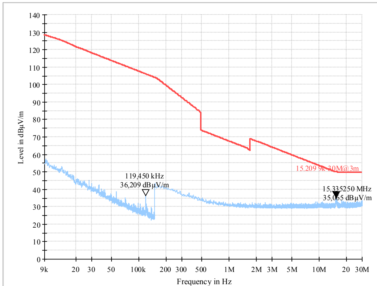
Plot 413: Mode 3, RSE 9 kHz – 30 MHz, channel 54, loop antenna (EUT standing)
