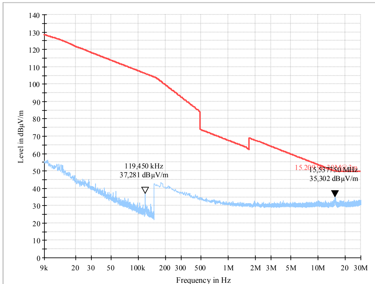
Plot 419: Mode 3, RSE 9 kHz – 30 MHz, channel 126, loop antenna (EUT standing)
