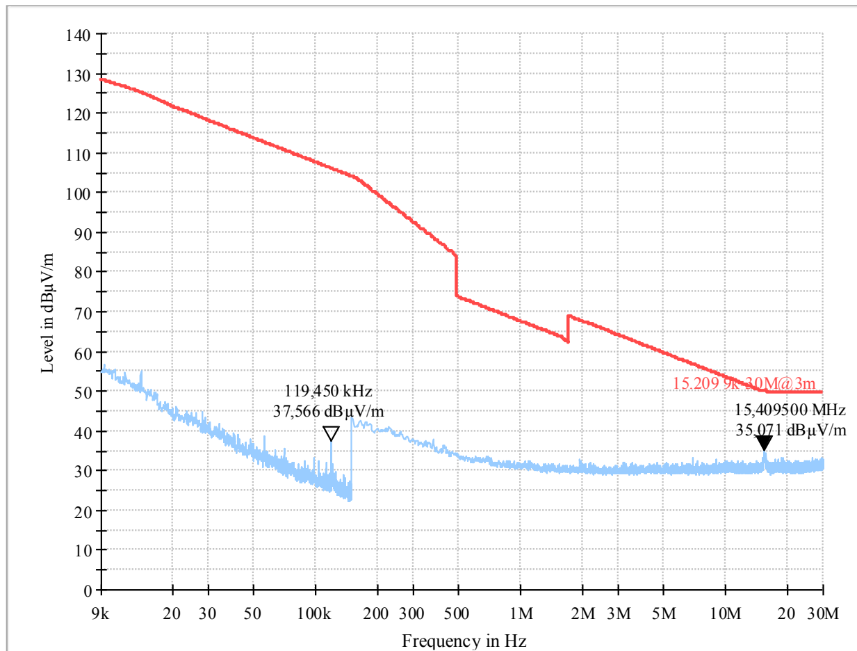
Plot 416: Mode 3, RSE 9 kHz – 30 MHz, channel 102, loop antenna (EUT laying)
