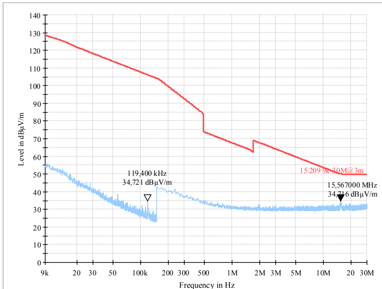
Plot 341: Mode 1, RSE 9 kHz – 30 MHz, channel 165, loop antenna (EUT standing)
