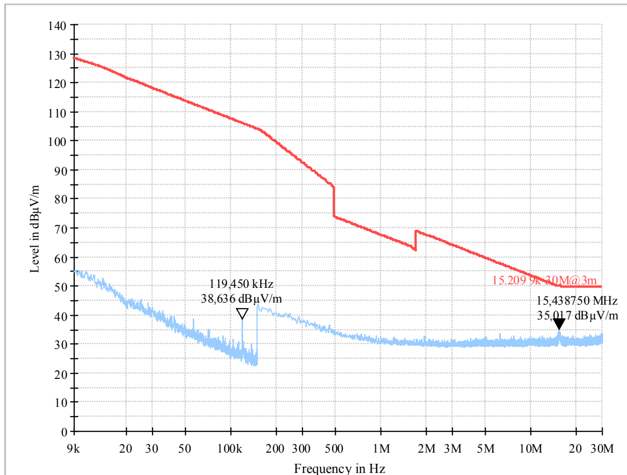
Plot 338: Mode 1, RSE 9 kHz – 30 MHz, channel 157, loop antenna (EUT laying)
