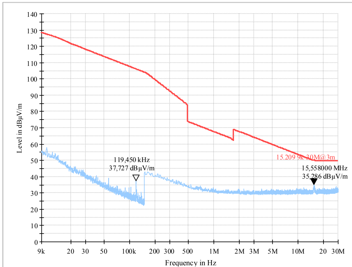
Plot 124: Mode 3, RSE 9 kHz – 30 MHz, low channel, loop antenna (EUT laying)
