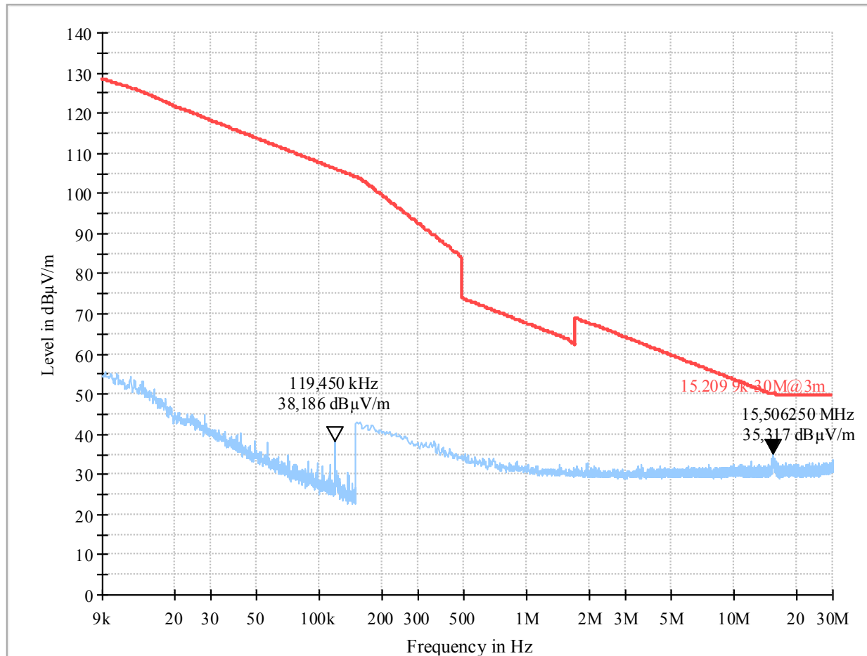
Plot 127: Mode 3, RSE 9 kHz – 30 MHz, high channel, loop antenna (EUT standing)
