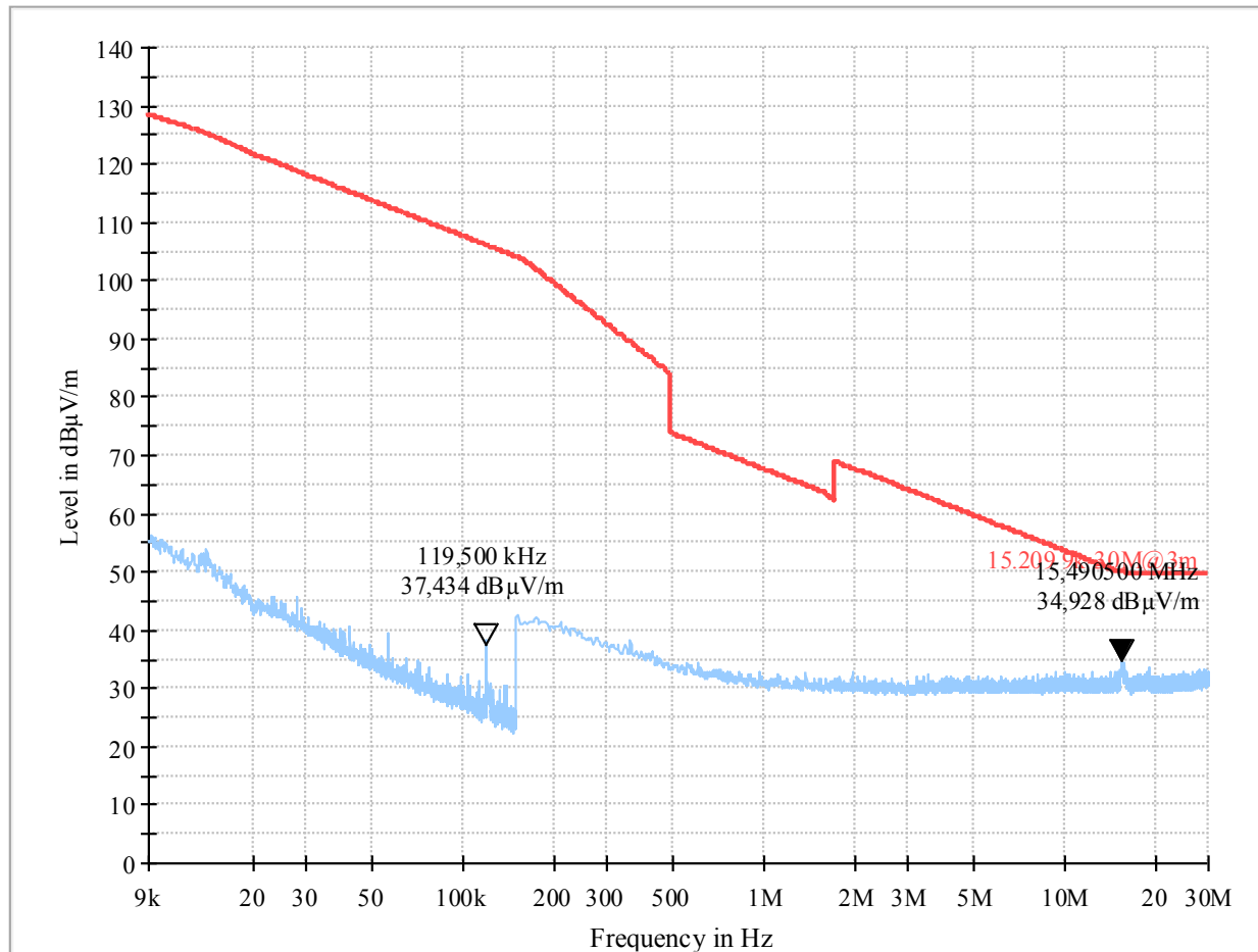
Plot 125: Mode 3, RSE 9 kHz – 30 MHz, low channel, loop antenna (EUT standing)
