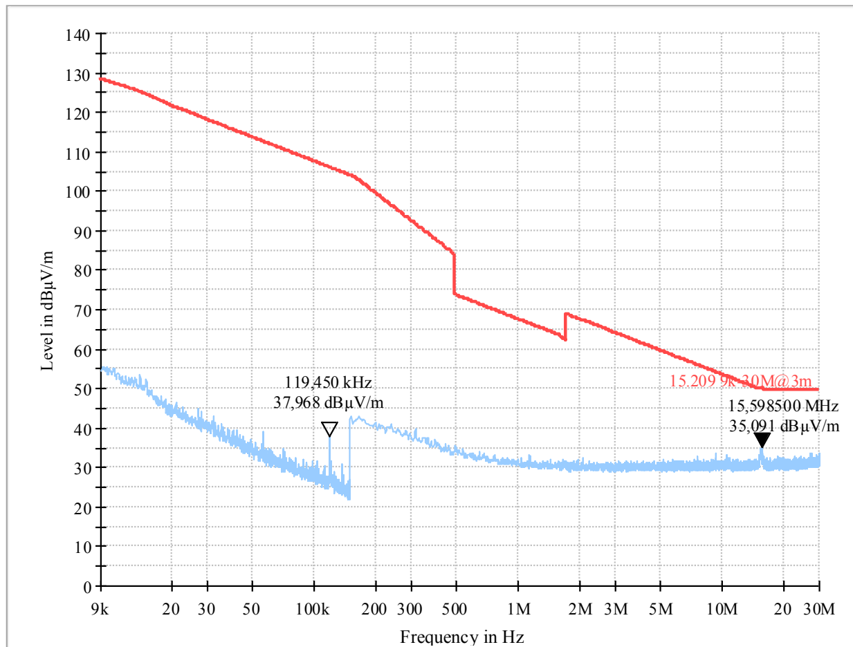
Plot 126: Mode 3, RSE 9 kHz – 30 MHz, high channel, loop antenna (EUT laying)
