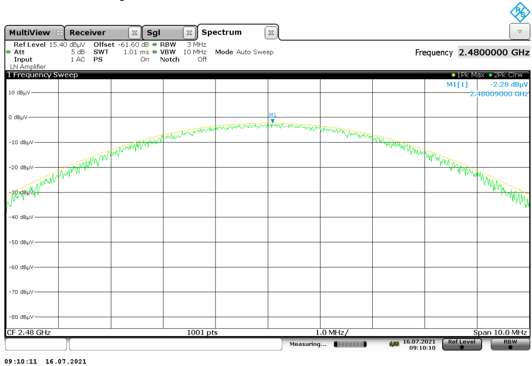
Plot 66: Mode 3, Peak EIRP, high channel
