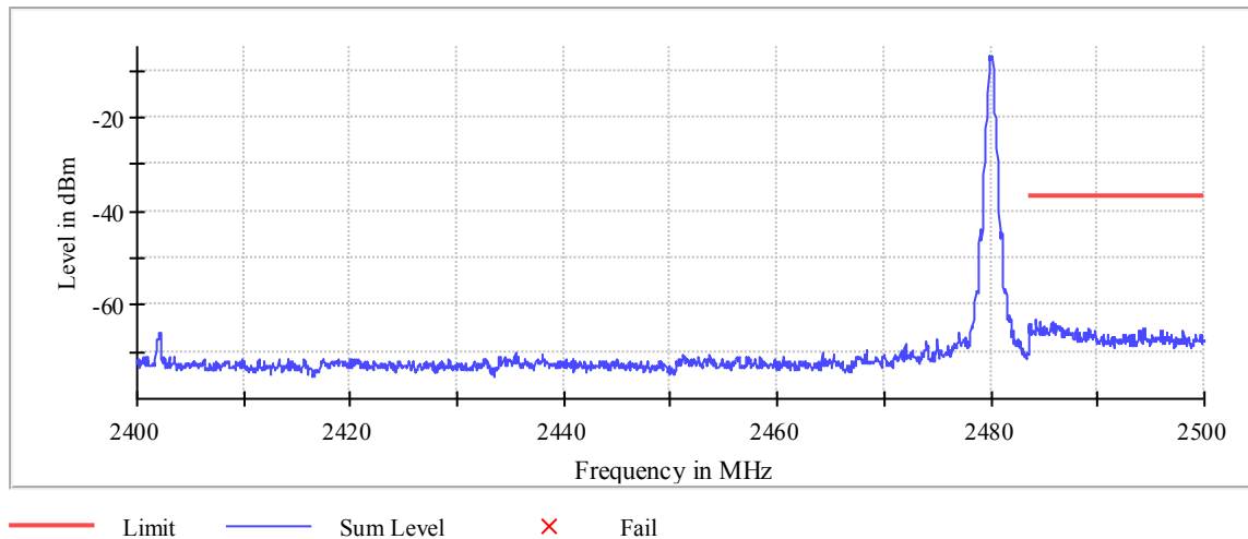
Plot 68: Mode 1, BEC, high channel
