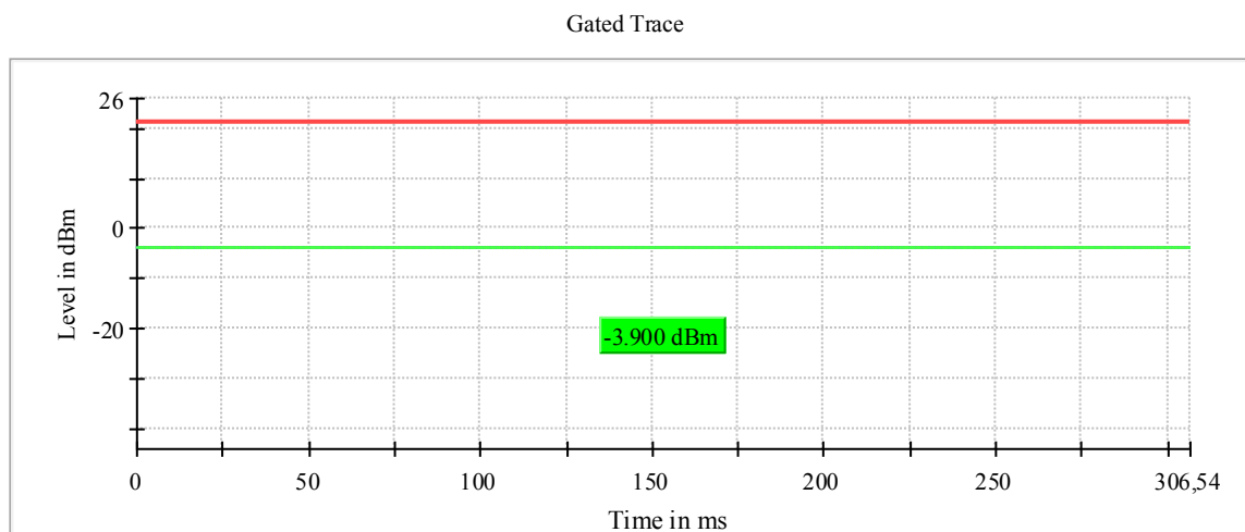
Plot 52: Mode 2, AVGPM-G Gated Average Power Measurement, low channel
