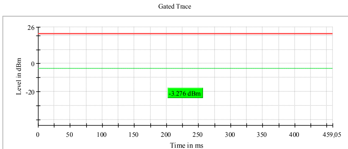
Plot 51: Mode 1, Peak Power, high channel
