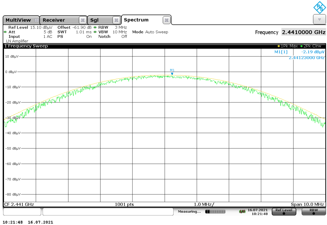
Plot 62: Mode 2, Peak EIRP, mid channel
