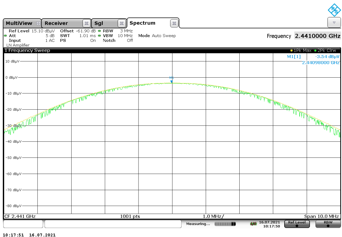
Plot 59: Mode 1, Peak EIRP, mid channel
