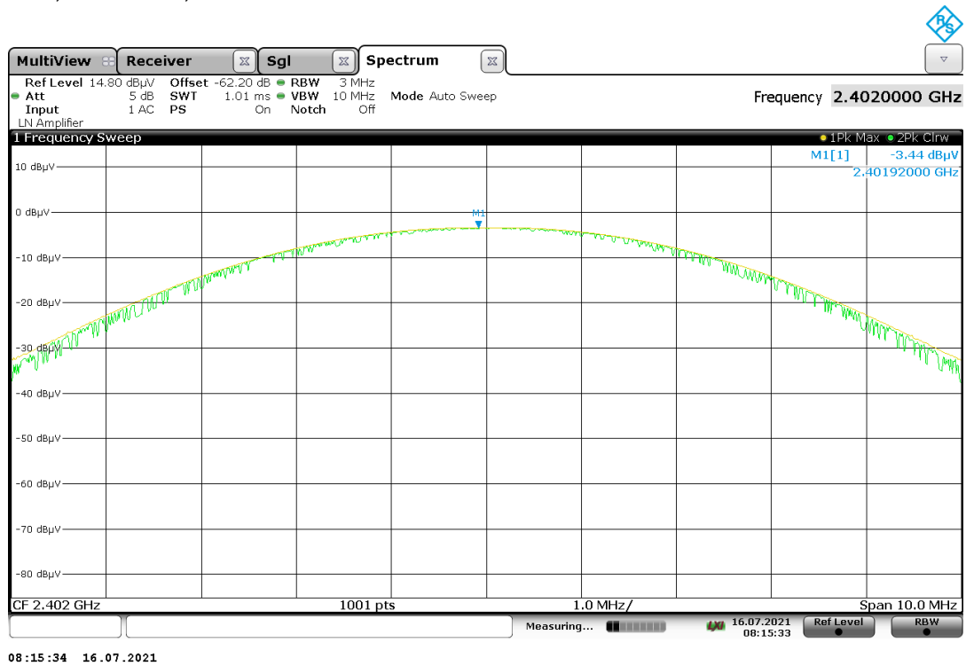
Plot 58: Mode 1, Peak EIRP, low channel
