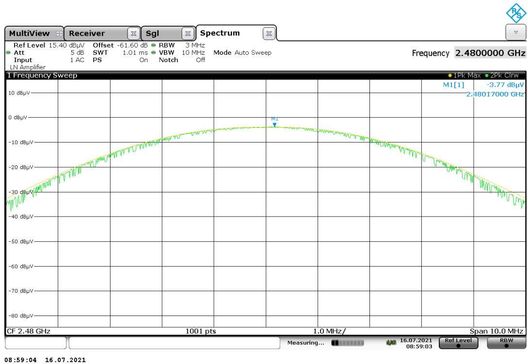
Plot 60: Mode 1, Peak EIRP, high channel
