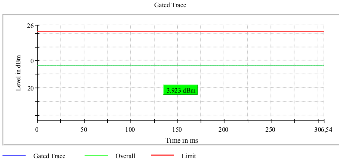
Plot 55: Mode 3, AVGPM-G Gated Average Power Measurement, low channel
