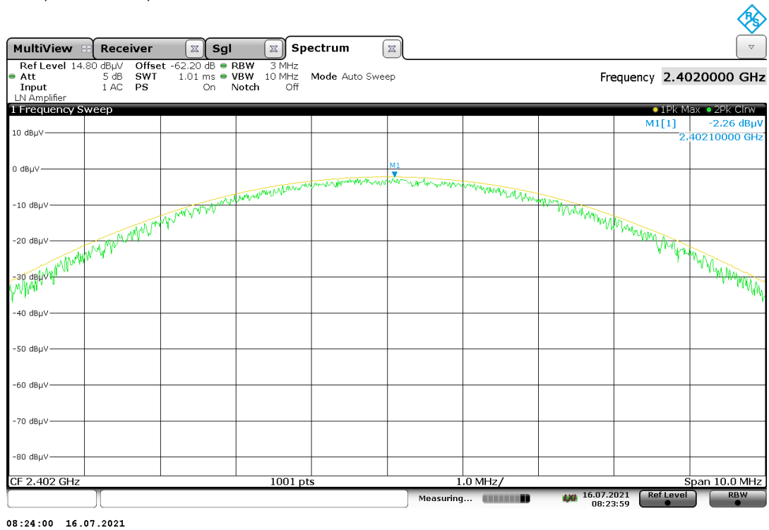
Plot 64: Mode 3, Peak EIRP, low channel
