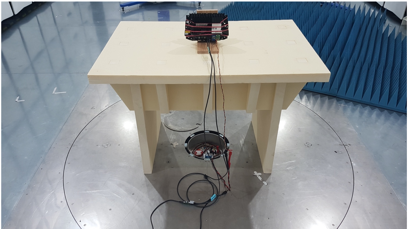
Photo No. 24: Test set-up 8.1 EUT view
