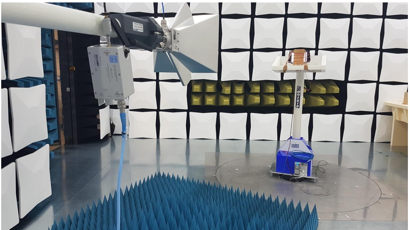
Photo No. 22: Test set-up 8.2 test antenna view
