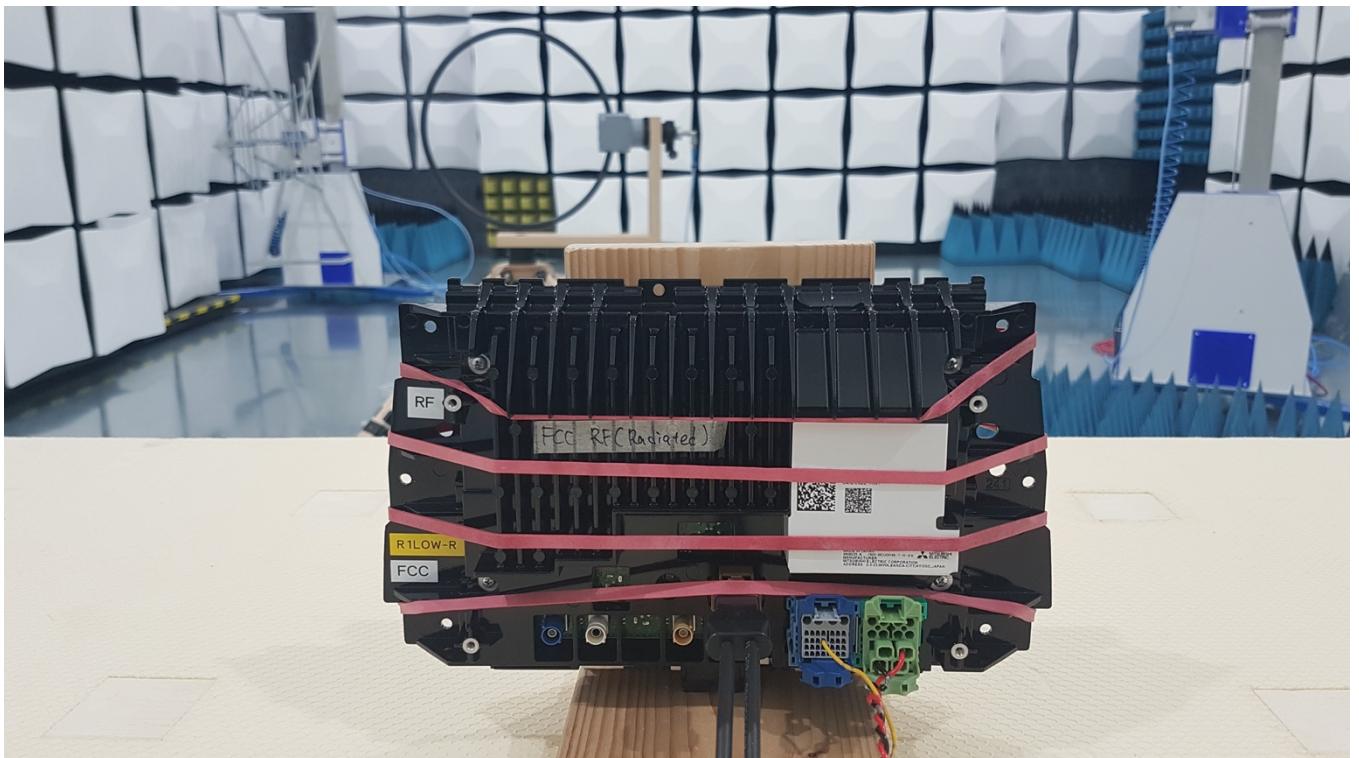
Photo No. 26: Test set-up 8.1 EUT view
