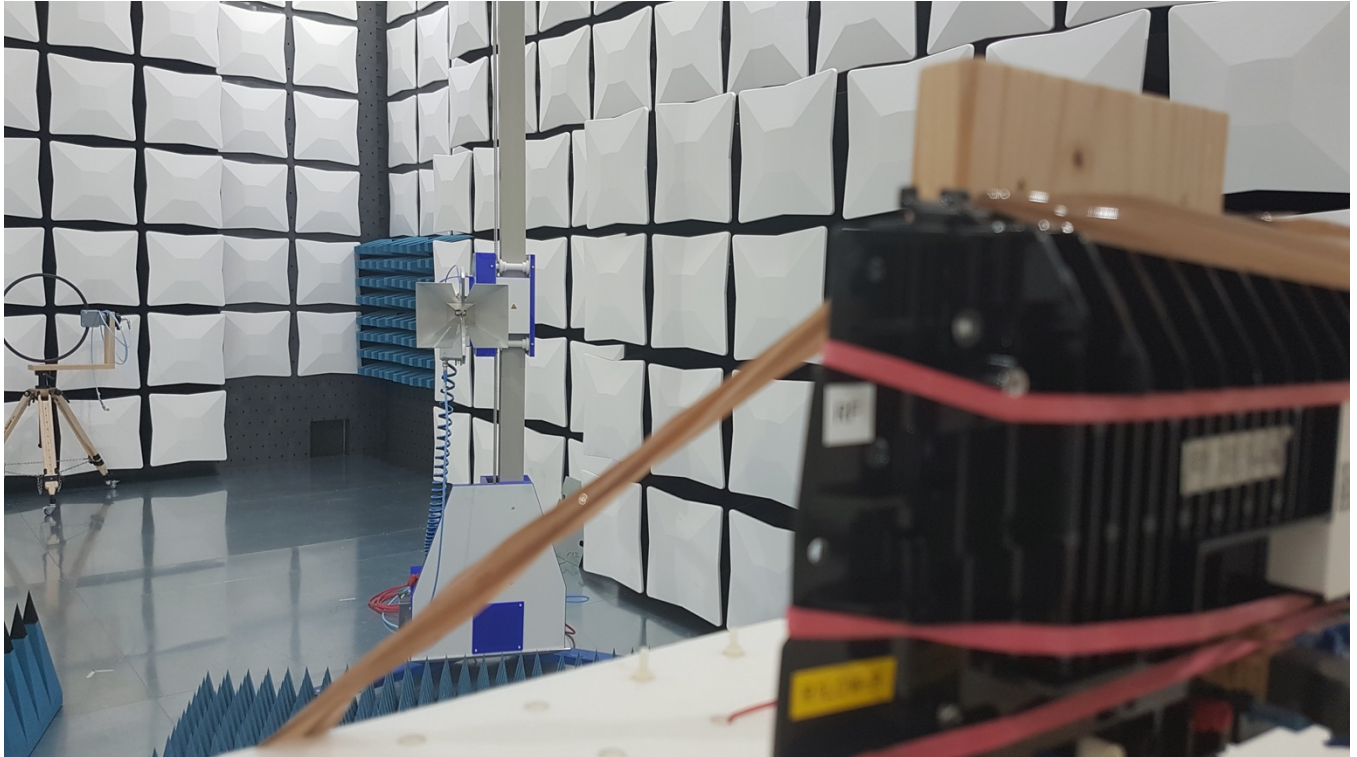
Photo No. 22: Test set-up 8.2 test antenna view
