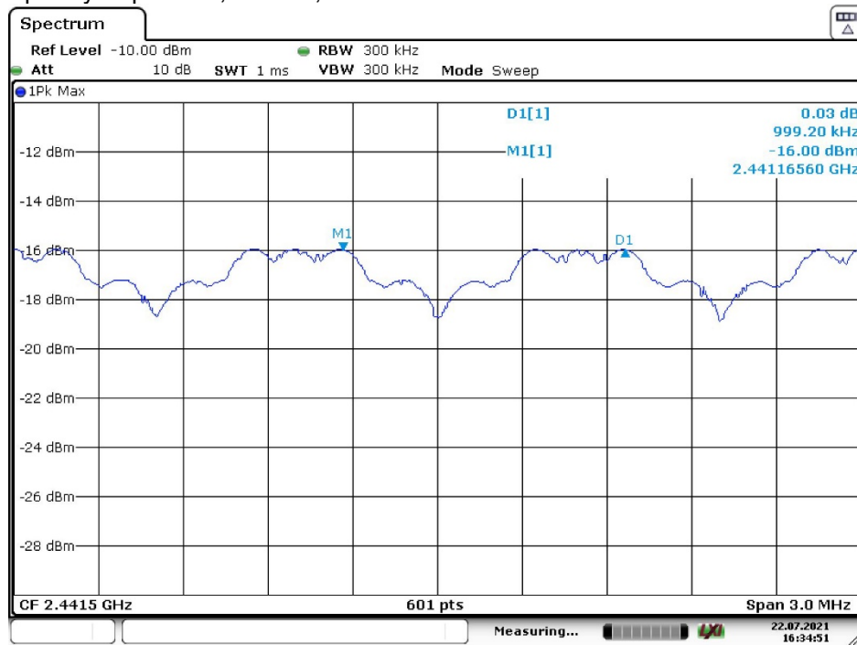
Plot 5: Carrier Frequency Separation, Mode 2, mid channel*
