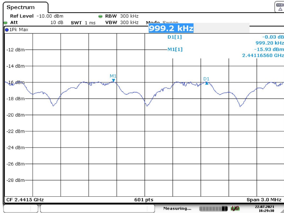
Plot 8: Carrier Frequency Separation, Mode 3, mid channel*
