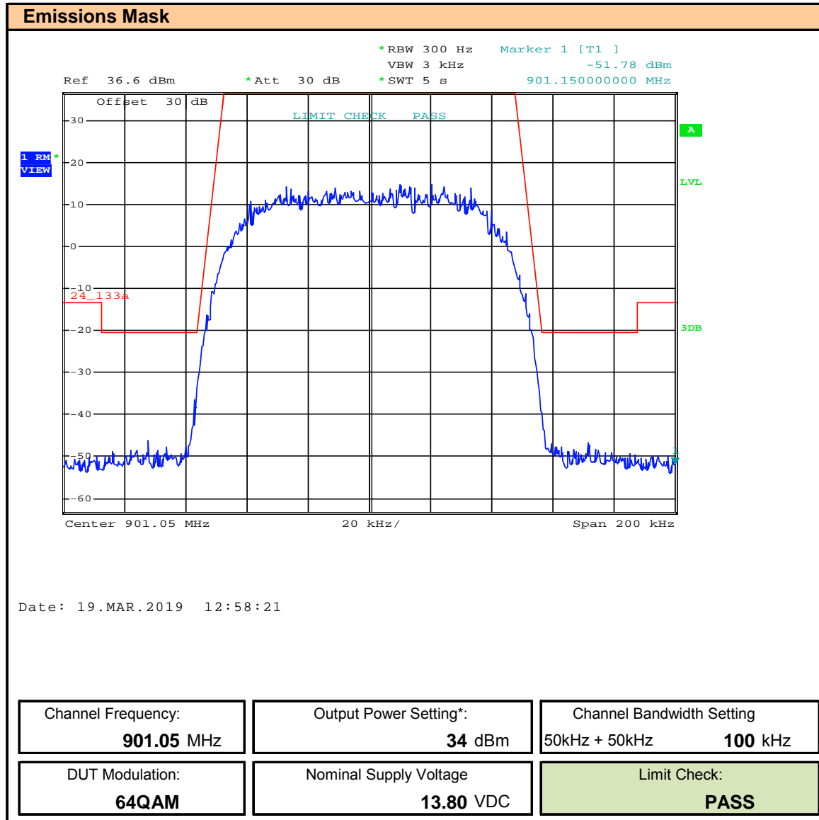
Plot 9.3 – Emissions Mask – 901.05, 100kHz BW, 64QAM
