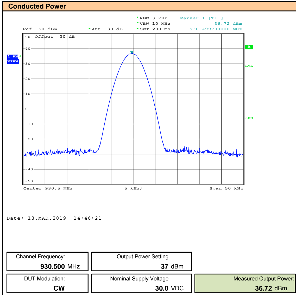
Plot 7.6 – Conducted Power – 930.5MHz, 30VDC
