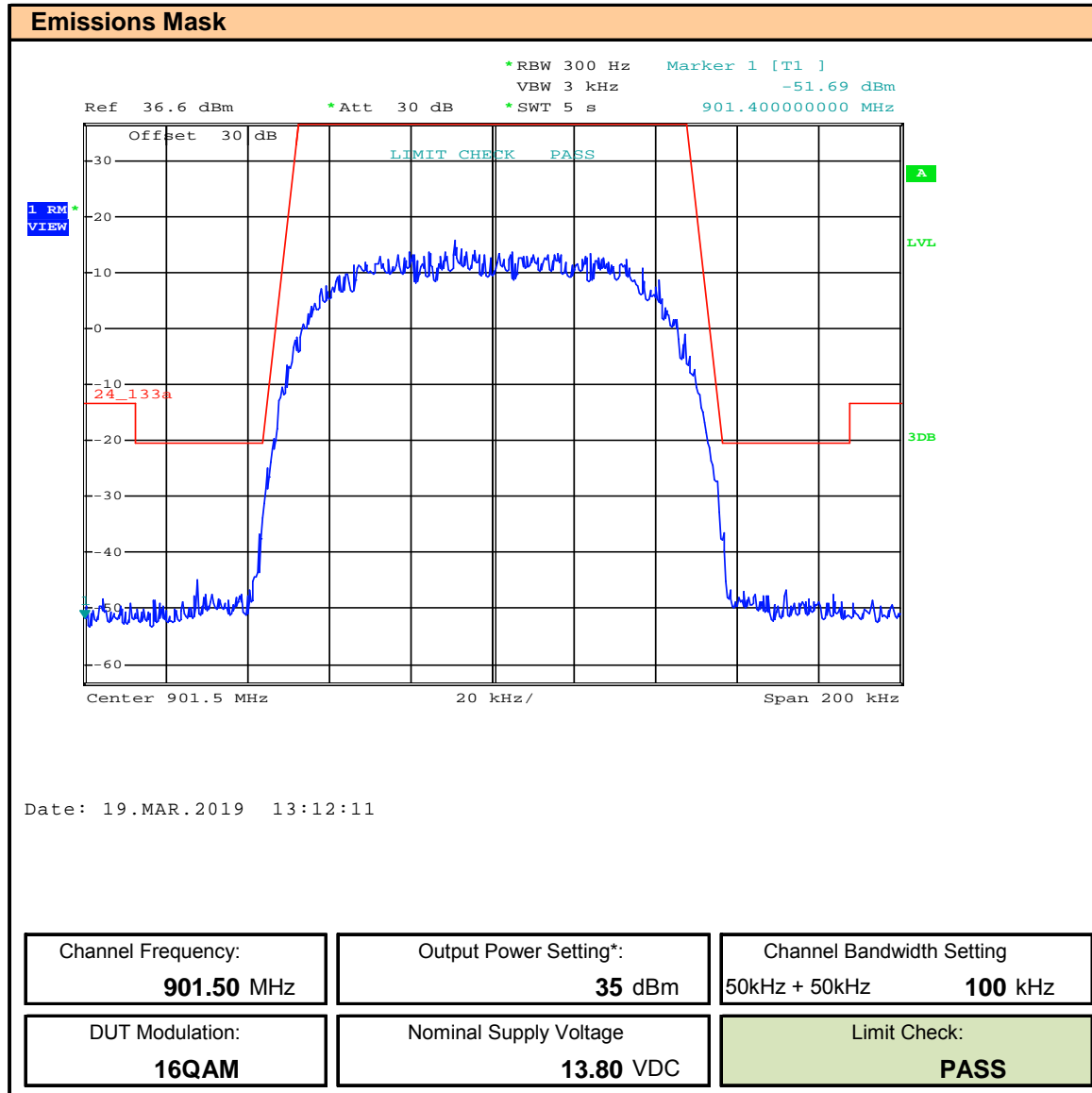
Plot 9.5 – Emissions Mask – 901.5, 100kHz BW, 16QAM
