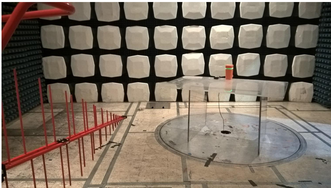
Photograph 1. Undesirable Emissions, Below 1 GHz, Test Setup
