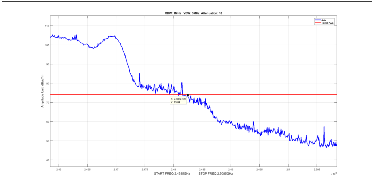
Plot 77. Radiated Emissions, Peak, 2483.5M radiated band edge, 802.11n, BW 20, CF 2462
