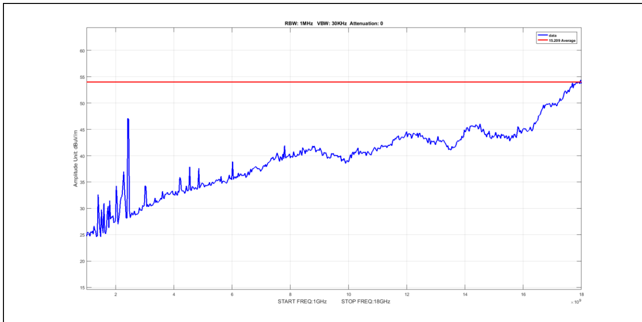
Plot 48. Radiated Emissions, Average, radiated spurious emissions, 802.11n, BW 40M, CF 2422M, 1-18GHz
