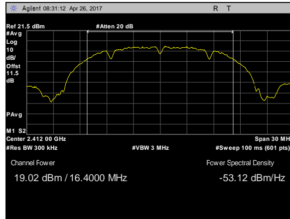
Plot 27. Peak Power Output, 802.11b, BW 20M, CF 2412M, c0
