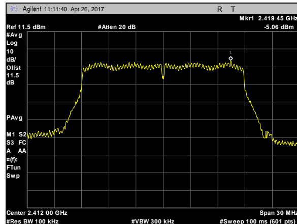
Plot 105. Power Spectral Density, 802.11n, BW 20M, CF 2412M, c0
