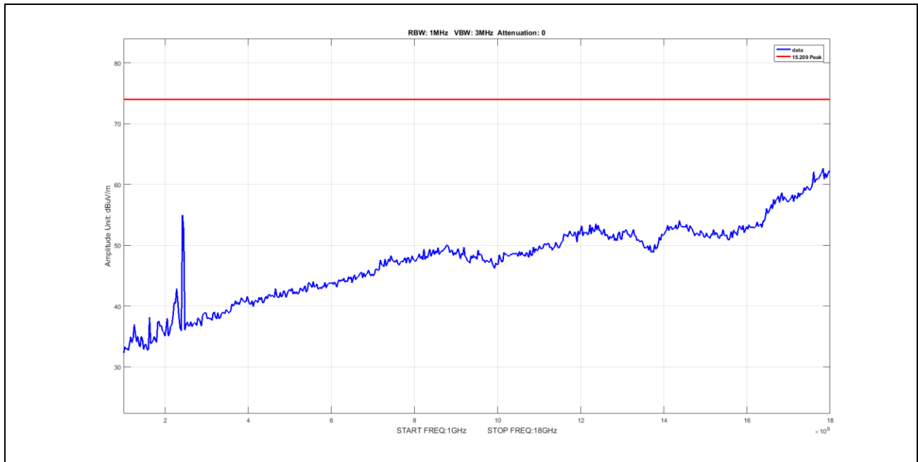
Plot 51. Radiated Emissions, Peak, radiated spurious emissions, 802.11b, BW 20M, CF 2412M, 1-18GHz
