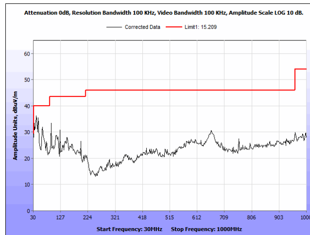
Radiated Emissions, Peak, radiated spurious emissions, 802.11n, BW 20M, CF 2462M, 30-1000MHz
