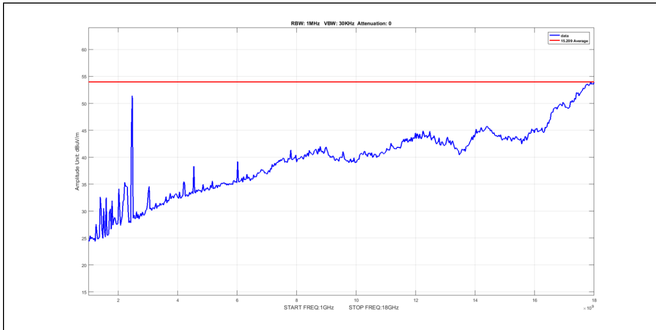
Plot 47. Radiated Emissions, Average, radiated spurious emissions, 802.11n, BW 20M, CF 2462M, 1-18GHz
