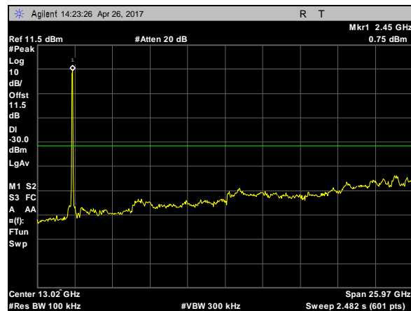
Plot 89. Spurious RF Conducted Emissions, 802.11n, 40M, CF 2437, 30MHz-26GHz
