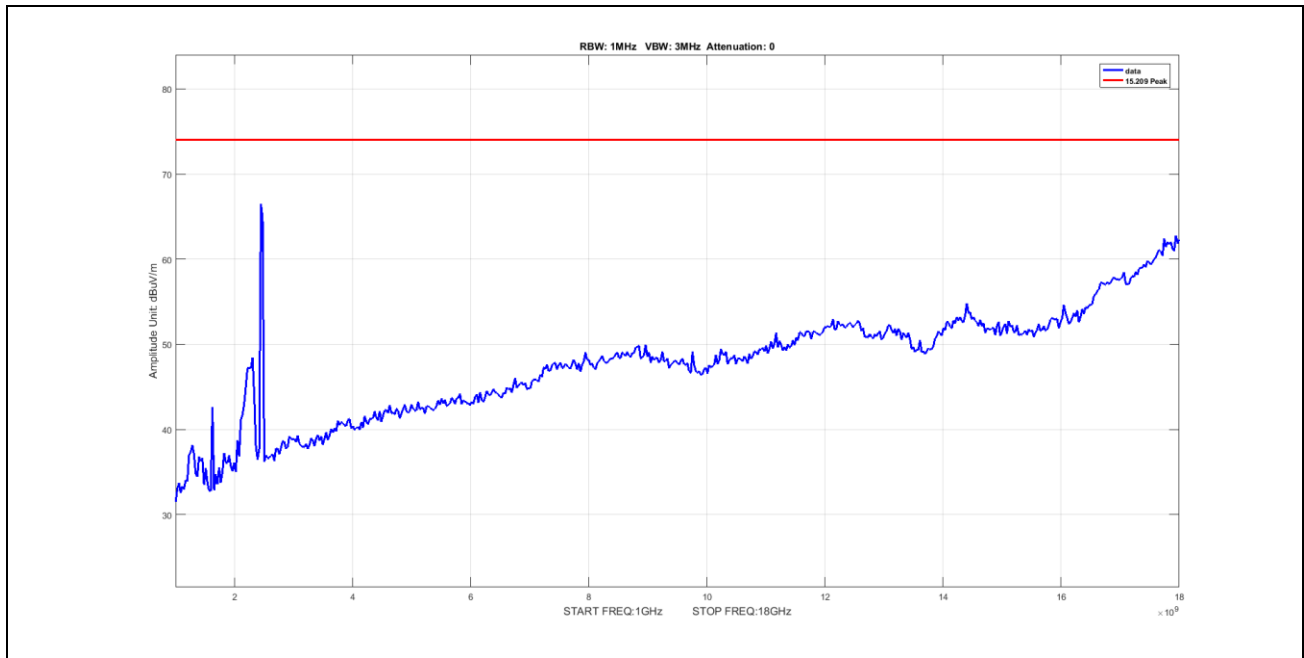
Plot 55. Radiated Emissions, Peak, radiated spurious emissions, 802.11g, BW 20M, CF 2437M, 1-18GHz
