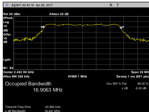
Plot 20. 99% Occupied Bandwidth, 802.11g, BW 20M, CF 2462M
