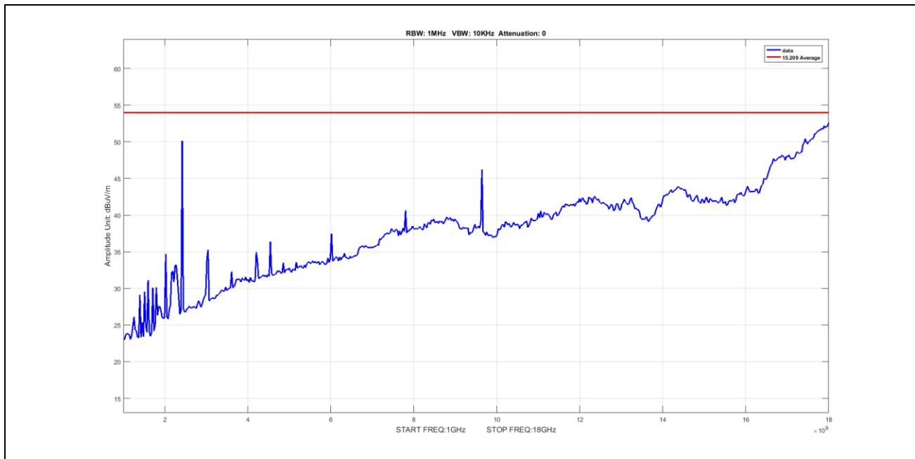
Plot 42. Radiated Emissions, Average, radiated spurious emissions, 802.11g, BW 20M, CF 2412M, 1-18GHz
