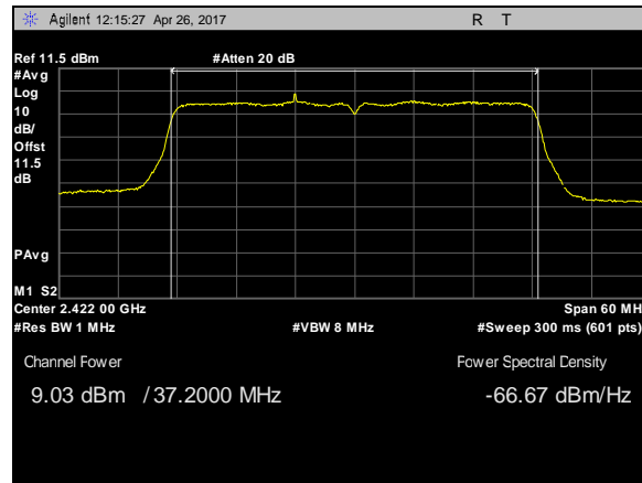
Plot 36. Peak Power Output, 802.11n, BW 40M, CF 2422M, c0
