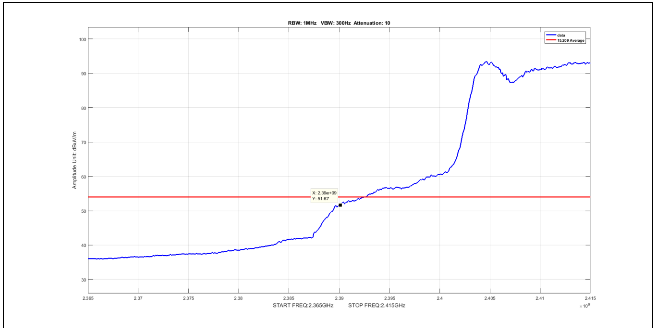
Plot 65. Radiated Emissions, Average, 2390M radiated band edge, 802.11g, BW 20, CF 2412
