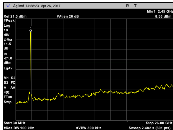
Plot 83. Spurious RF Conducted Emissions, 802.11g, 20M, CF 2437, 30MHz-26GHz
