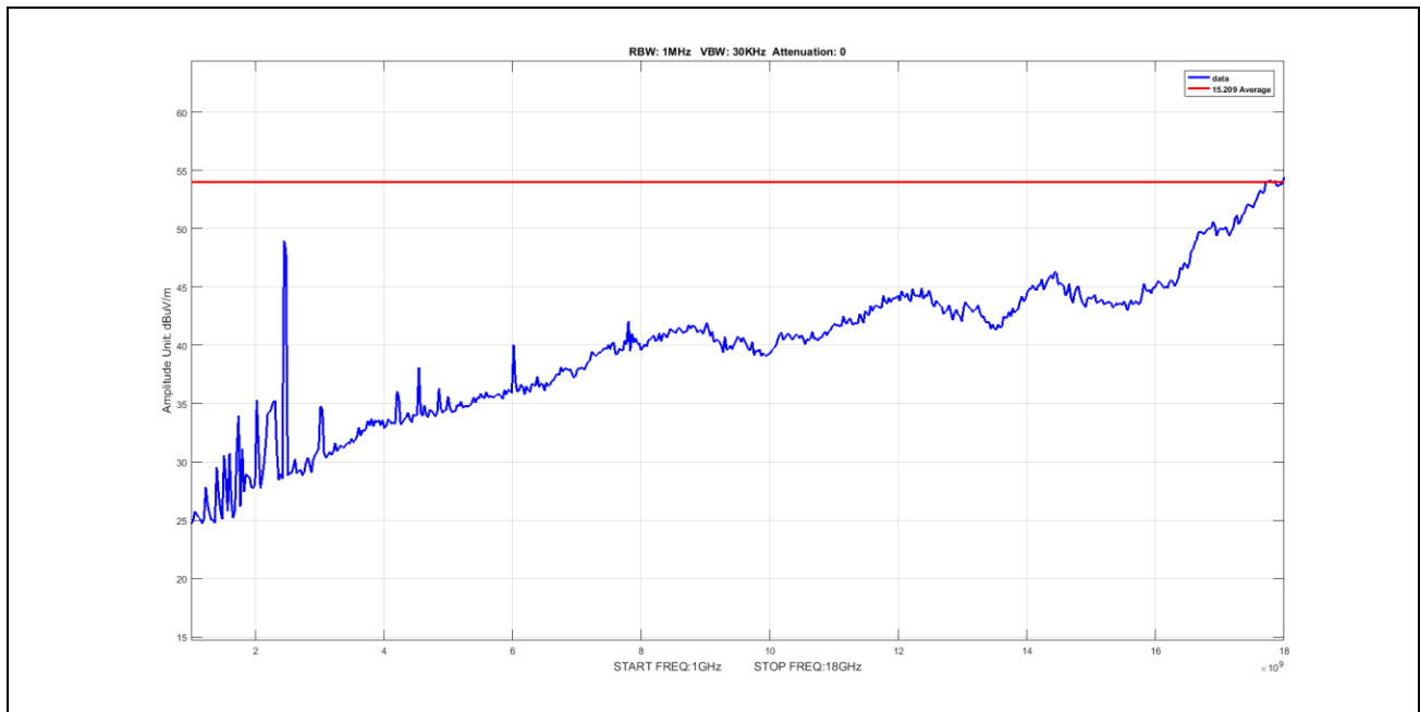
Plot 50. Radiated Emissions, Average, radiated spurious emissions, 802.11n, BW 40M, CF 2452M, 1-18GHz
