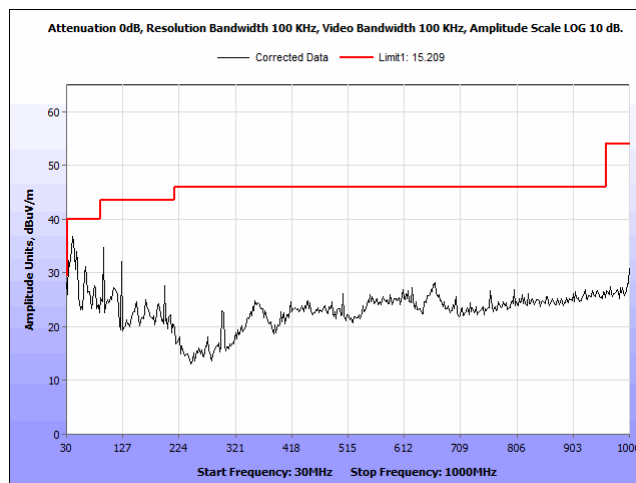
Radiated Emissions, Peak, radiated spurious emissions, 802.11n, BW 20M, CF 2412M, 30-1000MHz
