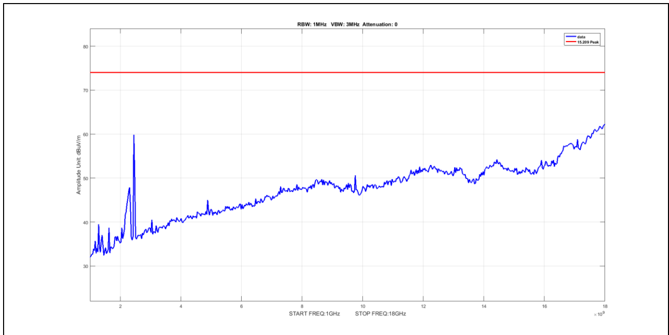
Plot 52. Radiated Emissions, Peak, radiated spurious emissions, 802.11b, BW 20M, CF 2437M, 1-18GHz
