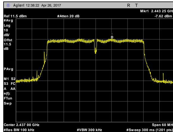
Plot 109. Power Spectral Density, 802.11n, BW 40M, CF 2437M, c0
