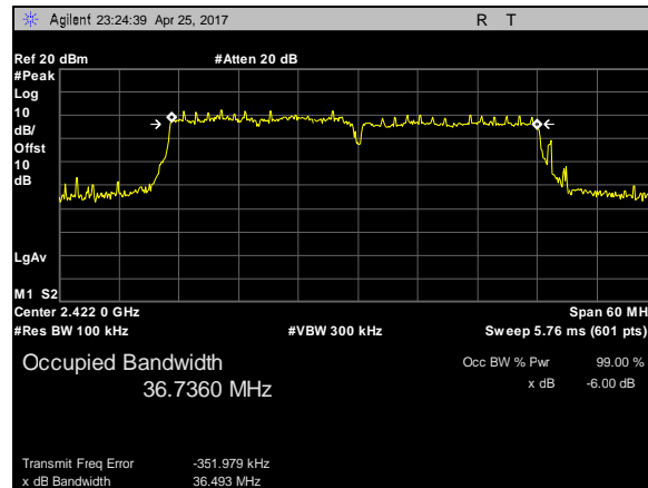
Plot 12. 6 dB Occupied DTS Bandwidth, 802.11n, BW 40M, CF 2422M
