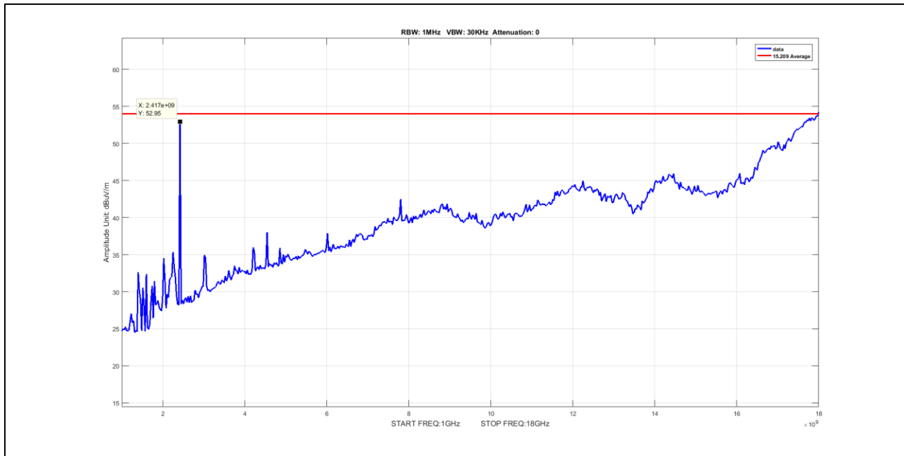
Plot 45. Radiated Emissions, Average, radiated spurious emissions, 802.11n, BW 20M, CF 2412M, 1-18GHz
