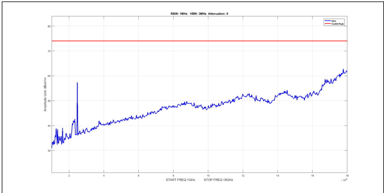
Plot 59. Radiated Emissions, Peak, radiated spurious emissions, 802.11n, BW 20M, CF 2462M, 1-18GHz
