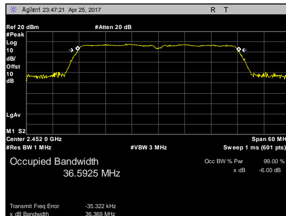
Plot 26. 99% Occupied Bandwidth, 802.11n, BW 40M, CF 2452M
