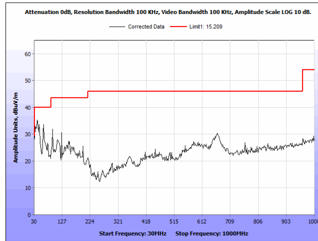
Radiated Emissions, Peak, radiated spurious emissions, 802.11n, BW 20M, CF 2437M, 30-1000MHz
