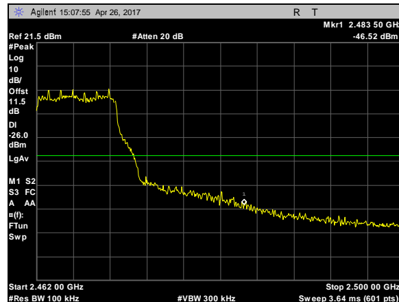
Plot 94. Spurious RF Conducted Emissions, 802.11g, 20M, CF 2462, high bandedge
