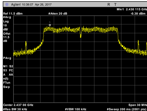
Plot 103. Power Spectral Density, 802.11g, BW 20M, CF 2437M, c0
