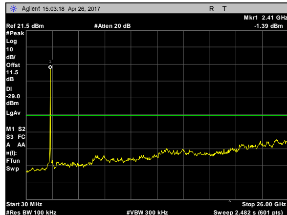
Plot 82. Spurious RF Conducted Emissions, 802.11g, 20M, CF 2412, 30MHz-26GHz
