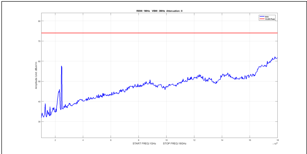
Plot 61. Radiated Emissions, Peak, radiated spurious emissions, 802.11n, BW 40M, CF 2437M, 1-18GHz
