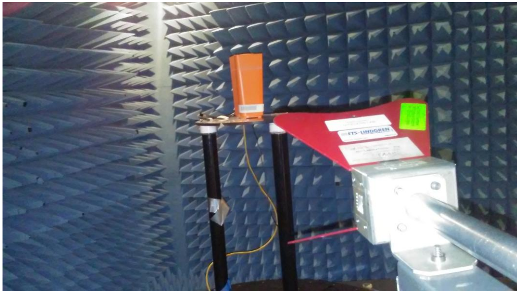
Photograph 3. Radiated Spurious Emissions, Test Setup above 1GHz
