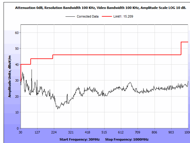
Radiated Emissions, Peak, radiated spurious emissions, 802.11g, BW 20M, CF 2412M, 30-1000MHz
