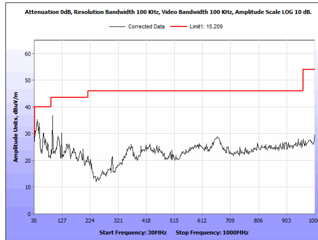
Radiated Emissions, Peak, radiated spurious emissions, 802.11b, BW 20M, CF 2462M, 30-1000MHz
