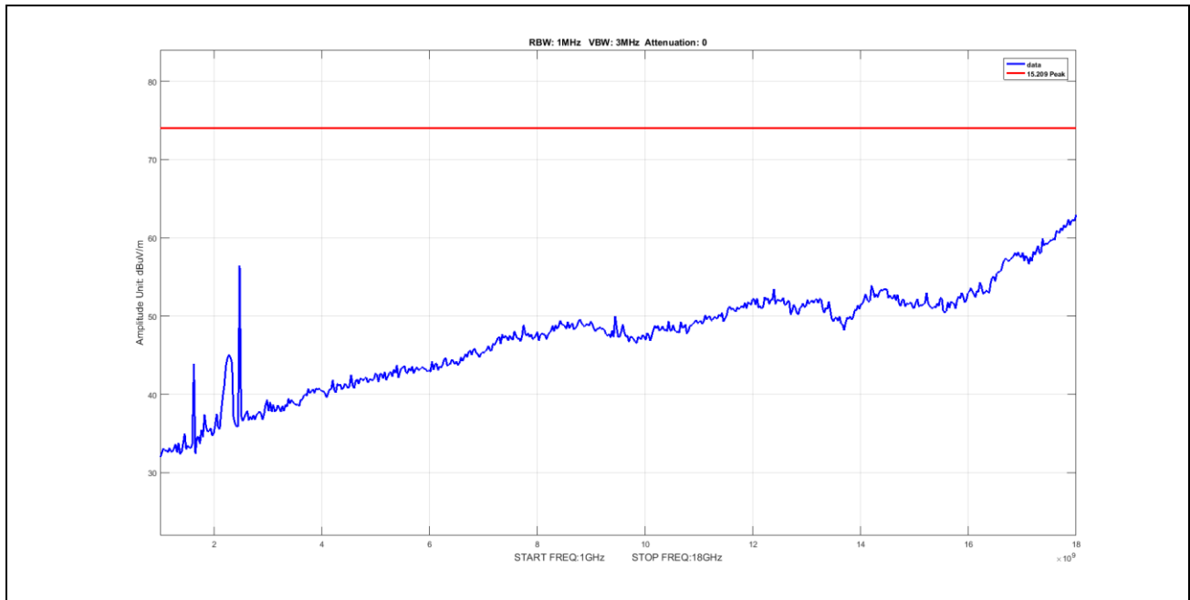
Plot 53. Radiated Emissions, Peak, radiated spurious emissions, 802.11b, BW 20M, CF 2462M, 1-18GHz
