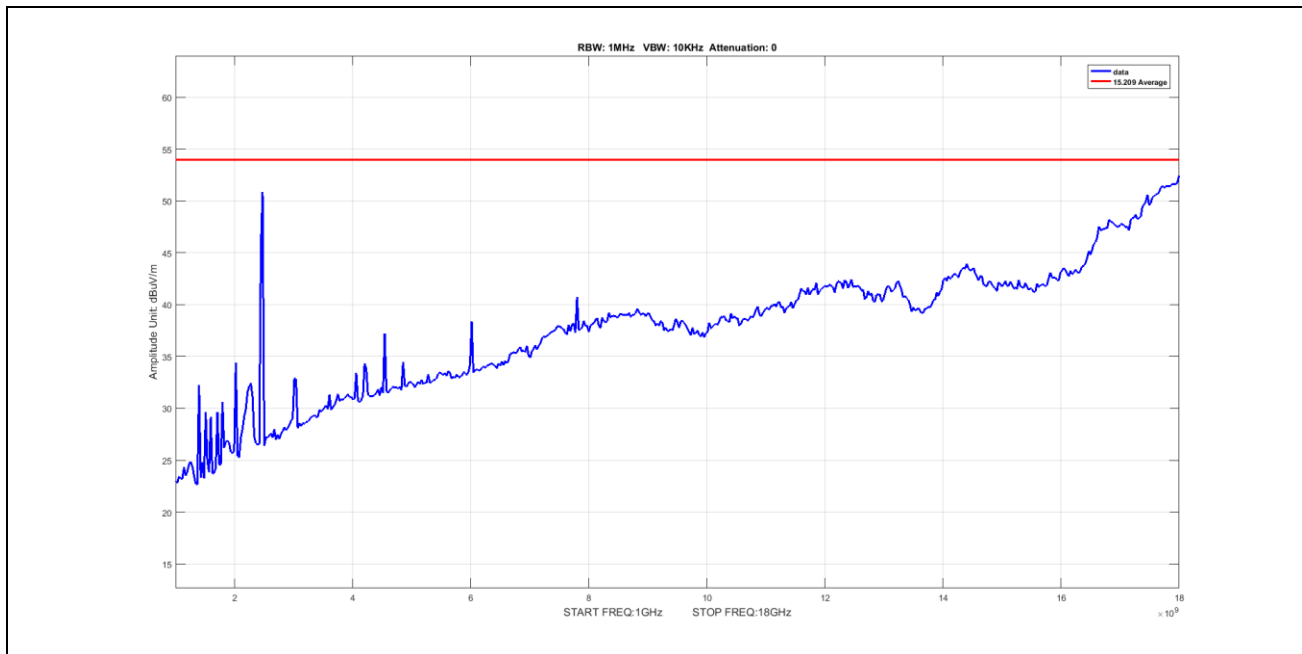
Plot 44. Radiated Emissions, Average, radiated spurious emissions, 802.11g, BW 20M, CF 2462M, 1-18GHz
