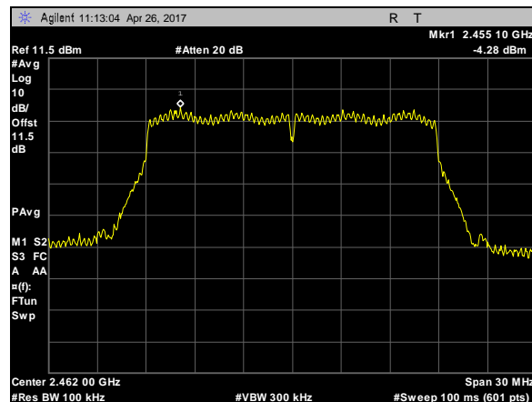
Plot 107. Power Spectral Density, 802.11n, BW 20M, CF 2462M, c0
