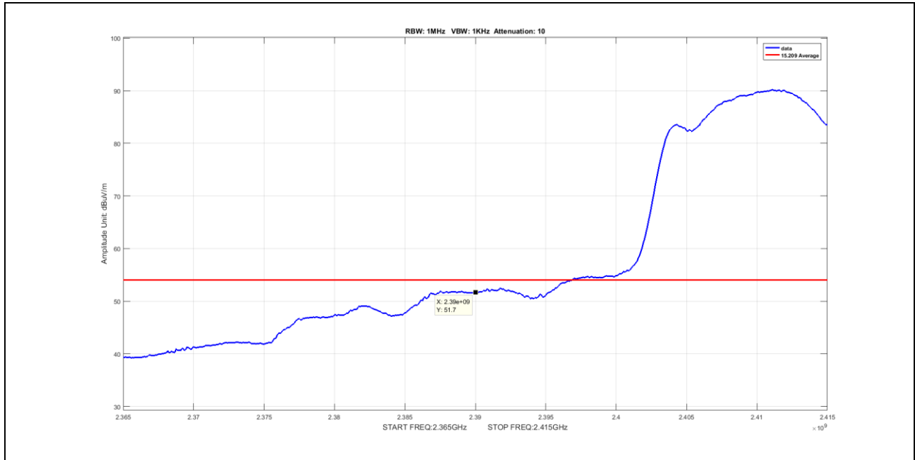
Plot 67. Radiated Emissions, Average, 2390M radiated band edge, 802.11n, BW 40, CF 2422
