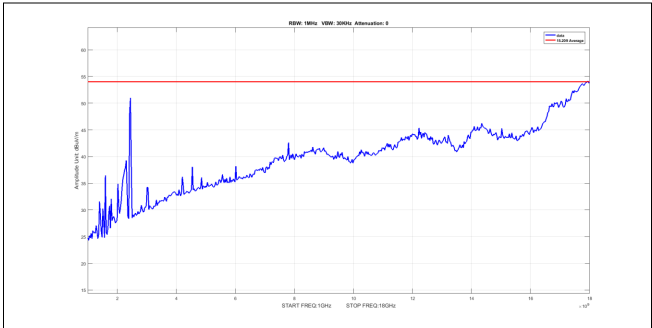
Plot 49. Radiated Emissions, Average, radiated spurious emissions, 802.11n, BW 40M, CF 2437M, 1-18GHz
