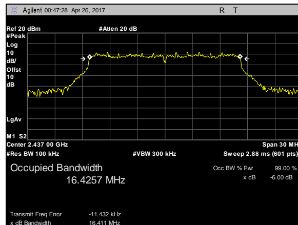
Plot 7. 6 dB Occupied DTS Bandwidth, 802.11g, BW 20M, CF 2437M
