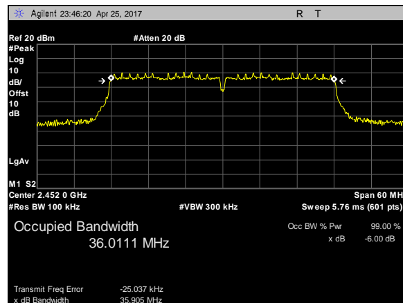
Plot 14. 6 dB Occupied DTS Bandwidth, 802.11n, BW 40M, CF 2452M
