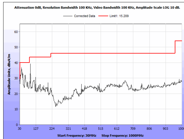
Radiated Emissions, Peak, radiated spurious emissions, 802.11n, BW 40M, CF 2412M, 30-1000MHz
