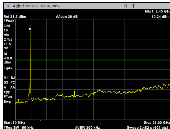
Plot 81. Spurious RF Conducted Emissions, 802.11b, 20M, CF 2462, 30MHz-26GHz
