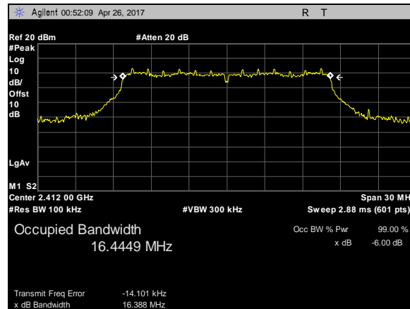
Plot 6. 6 dB Occupied DTS Bandwidth, 802.11g, BW 20M, CF 2412M
