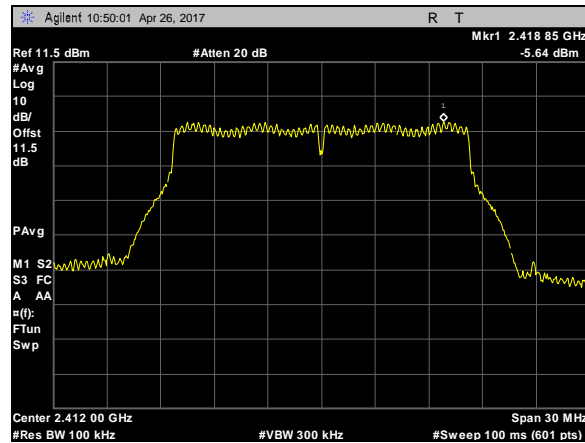
Plot 102. Power Spectral Density, 802.11g, BW 20M, CF 2412M, c0
