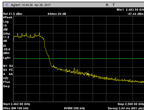
Plot 98. Spurious RF Conducted Emissions, 802.11n, 20M, CF 2462, high bandedge
