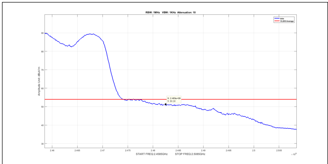
Plot 70. Radiated Emissions, Average, 2483.5M radiated band edge, 802.11n, BW 40, CF 2452
