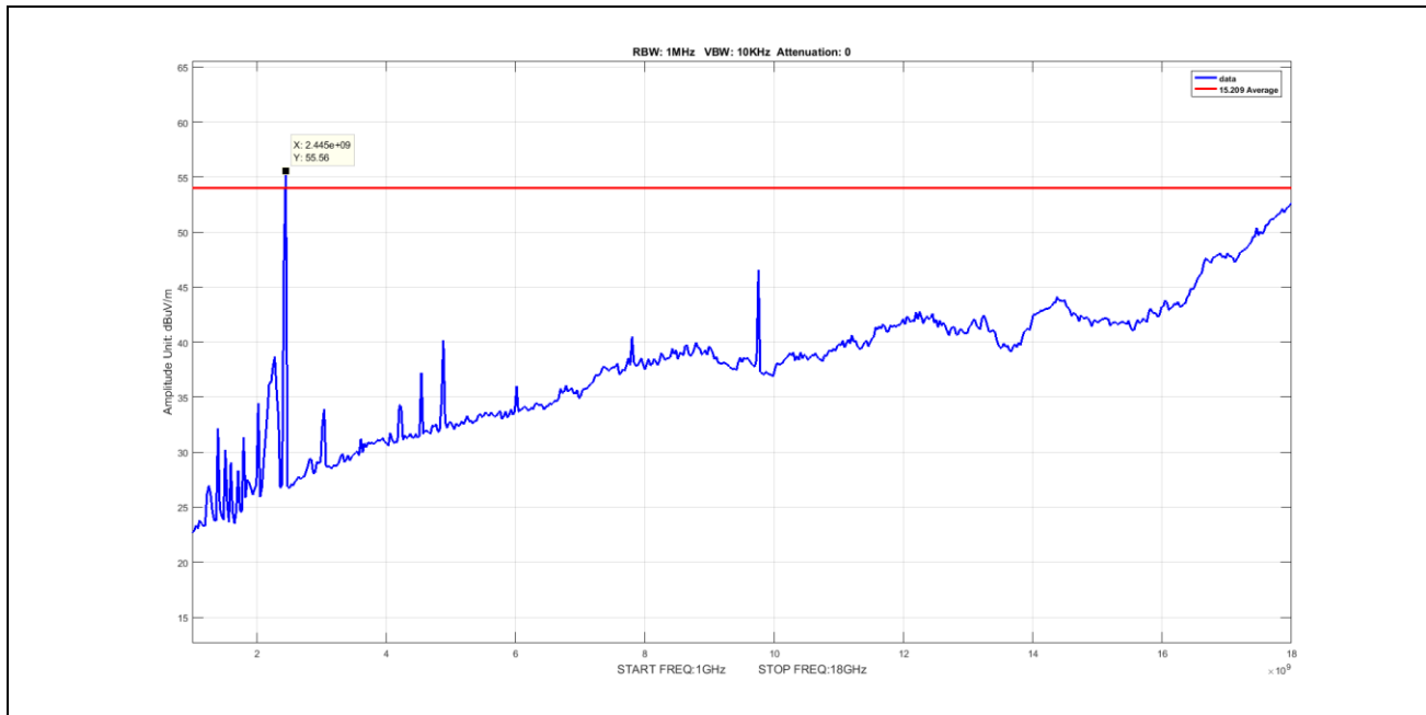
Plot 40. Radiated Emissions, Average, radiated spurious emissions, 802.11b, BW 20M, CF 2437M, 1-18GHz
