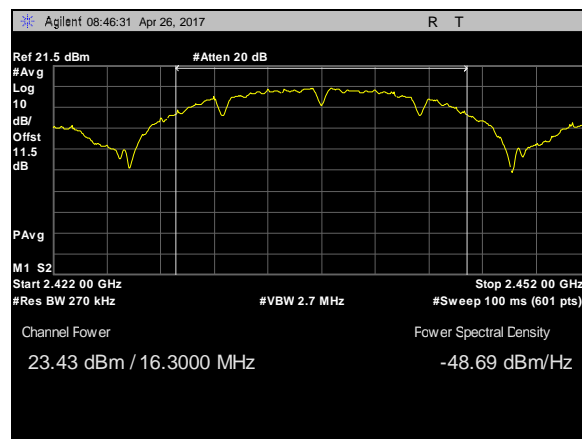
Plot 28. Peak Power Output, 802.11b, BW 20M, CF 2437M, c0
