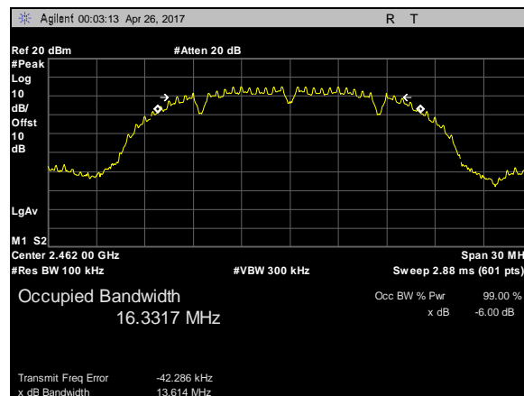
Plot 5. 6 dB Occupied DTS Bandwidth, 802.11b, BW 20M, CF 2462M
