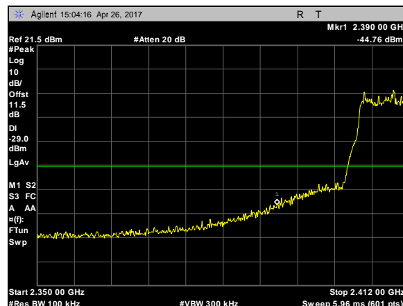
Plot 93. Spurious RF Conducted Emissions, 802.11g, 20M, CF 2412, low bandedge
