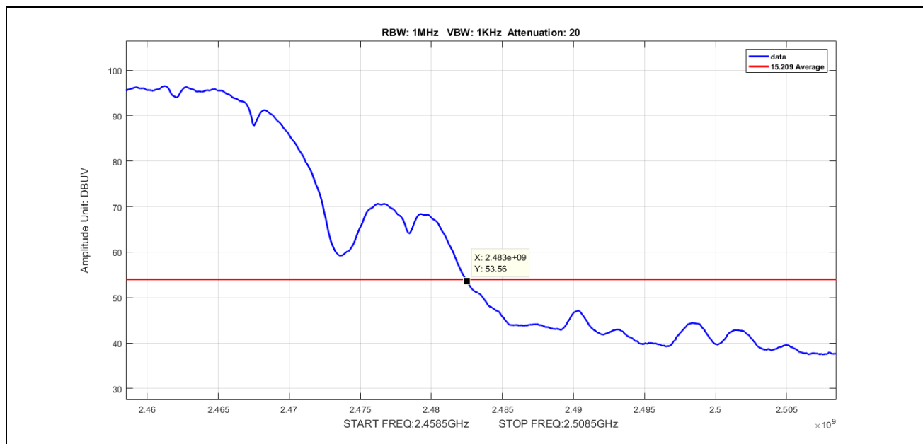
Plot 64. Radiated Emissions, Average, 802.11b, 2483.5M radiated band edge, BW 20, CF 2462M
