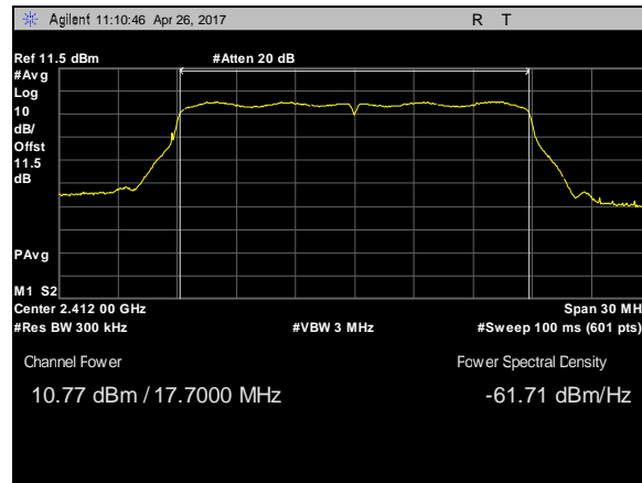
Plot 33. Peak Power Output, 802.11n, BW 20M, CF 2412M, c0
