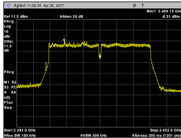
Plot 108. Power Spectral Density, 802.11n, BW 40M, CF 2422M, c0
