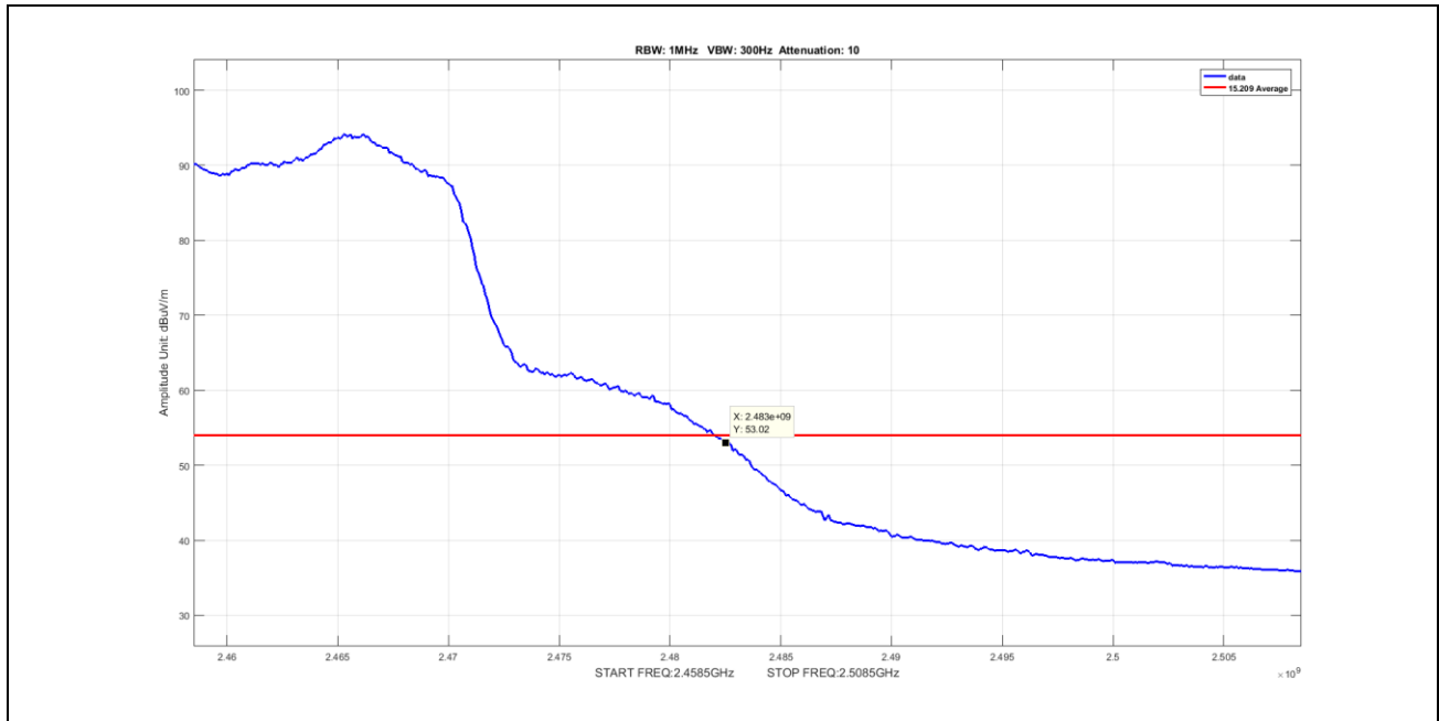
Plot 68. Radiated Emissions, Average, 2483.5M radiated band edge, 802.11g, BW 20, CF 2462
