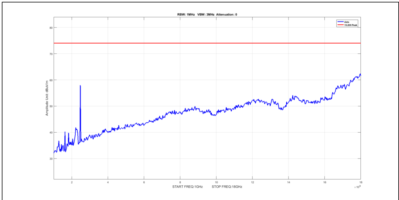
Plot 56. Radiated Emissions, Peak, radiated spurious emissions, 802.11g, BW 20M, CF 2462M, 1-18GHz
