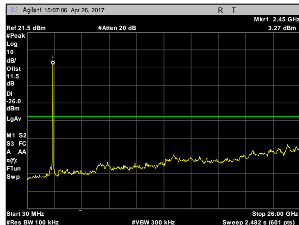
Plot 84. Spurious RF Conducted Emissions, 802.11g, 20M, CF 2462, 30MHz-26GHz
