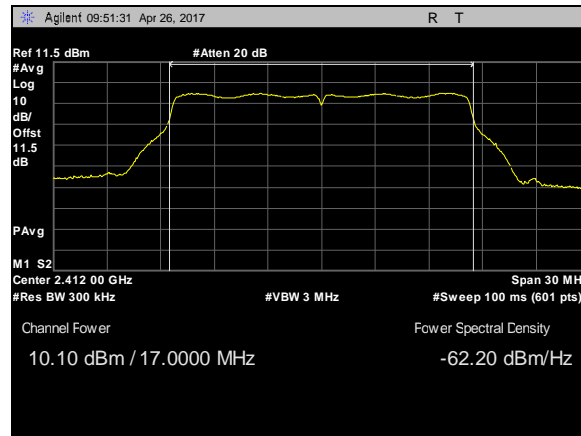
Plot 30. Peak Power Output, 802.11g, BW 20M, CF 2412M, c0
