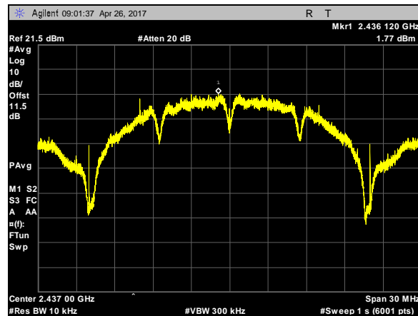
Plot 100. Power Spectral Density, 802.11b, BW 20M, CF 2437M, c0
