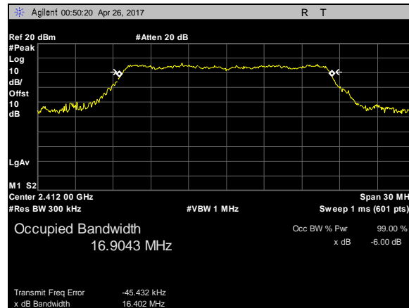
Plot 18. 99% Occupied Bandwidth, 802.11g, BW 20M, CF 2412M
