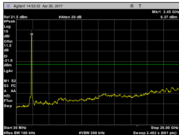
Plot 86. Spurious RF Conducted Emissions, 802.11n, 20M, CF 2437, 30MHz-26GHz
