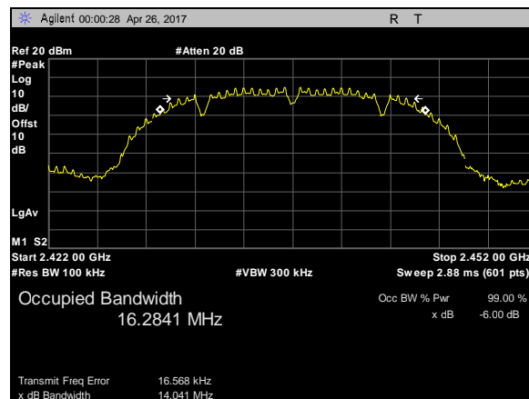
Plot 4. 6 dB Occupied DTS Bandwidth, 802.11b, BW 20M, CF 2437M
