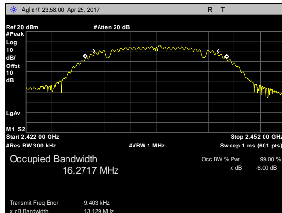
Plot 16. 99% Occupied Bandwidth, 802.11b, BW 20M, CF 2437M
