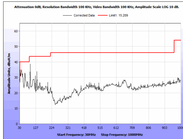
Radiated Emissions, Peak, radiated spurious emissions, 802.11n, BW 40M, CF 2462M, 30-1000MHz
