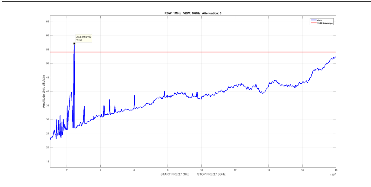
Plot 43. Radiated Emissions, Average, radiated spurious emissions, 802.11g, BW 20M, CF 2437M, 1-18GHz
