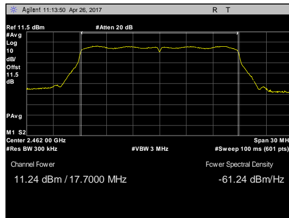
Plot 35. Peak Power Output, 802.11n, BW 20M, CF 2462M, c0
