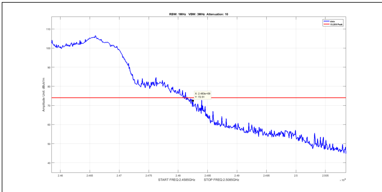
Plot 76. Radiated Emissions, Peak, 2483.5M radiated band edge, 802.11g, BW 20, CF 2462
