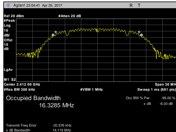
Plot 15. 99% Occupied Bandwidth, 802.11b, BW 20M, CF 2412M
