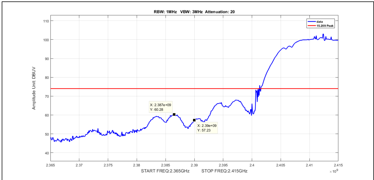
Plot 71. Radiated Emissions, Peak, 802.11b, 2390M radiated band edge, BW 20, CF 2412M
