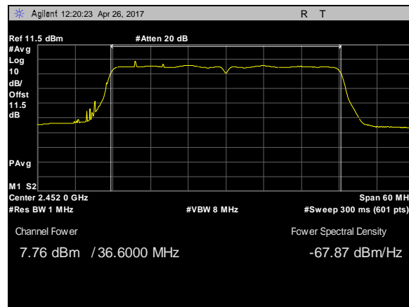
Plot 38. Peak Power Output, 802.11n, BW 40M, CF 2452M, c0
