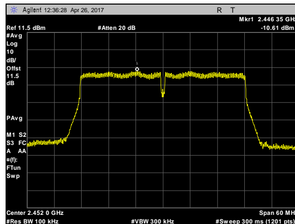
Plot 110. Power Spectral Density, 802.11n, BW 40M, CF 2452M, c0
