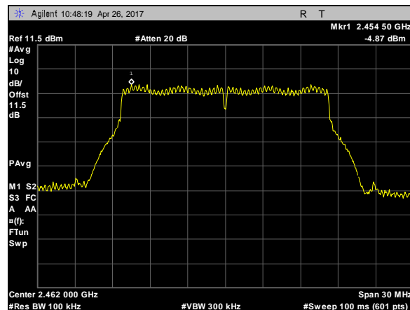
Plot 104. Power Spectral Density, 802.11g, BW 20M, CF 2462M, c0
