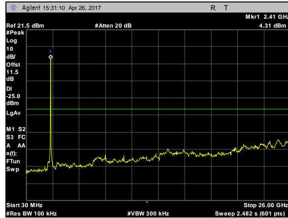
Plot 79. Spurious RF Conducted Emissions, 802.11b, 20M, CF 2412, 30MHz-26GHz
