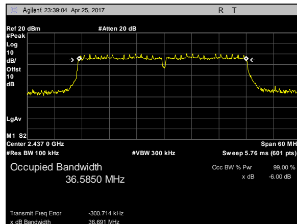
Plot 13. 6 dB Occupied DTS Bandwidth, 802.11n, BW 40M, CF 2437M
