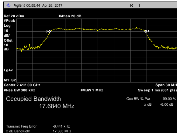
Plot 21. 99% Occupied Bandwidth, 802.11n, BW 20M, CF 2412M
