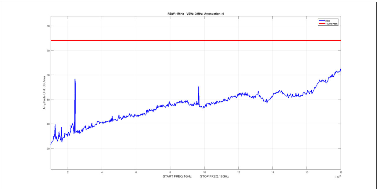
Plot 54. Radiated Emissions, Peak, radiated spurious emissions, 802.11g, BW 20M, CF 2412M, 1-18GHz
