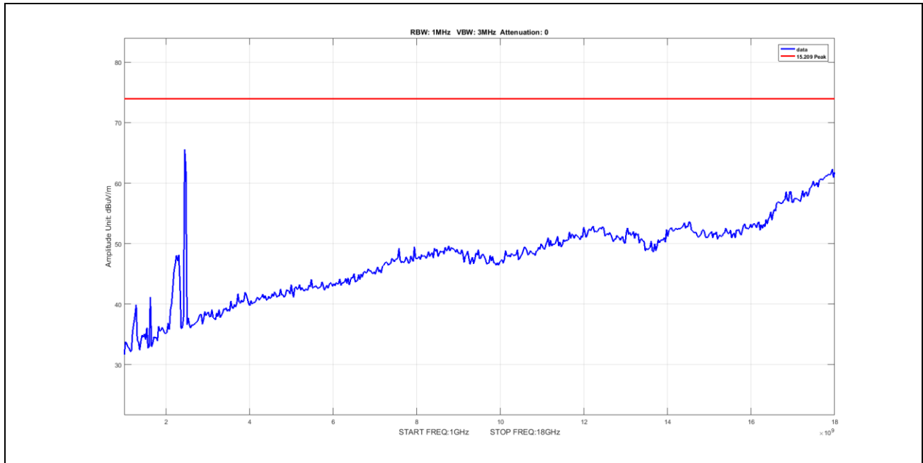
Plot 58. Radiated Emissions, Peak, radiated spurious emissions, 802.11n, BW 20M, CF 2437M, 1-18GHz
