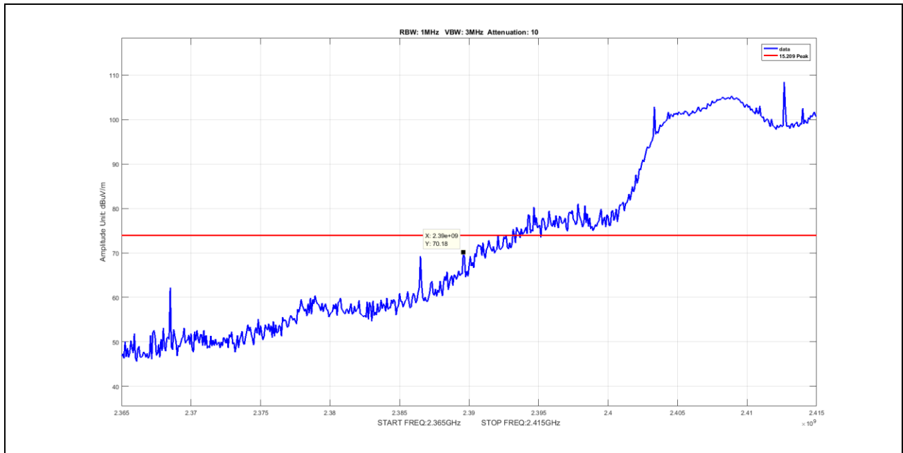
Plot 74. Radiated Emissions, Peak, 2390M radiated band edge, 802.11n, BW 20, CF 2412
