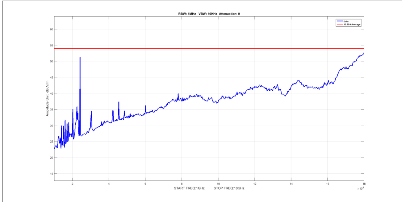
Plot 39. Radiated Emissions, Average, radiated spurious emissions, 802.11b, BW 20M, CF 2412M, 1-18GHz
