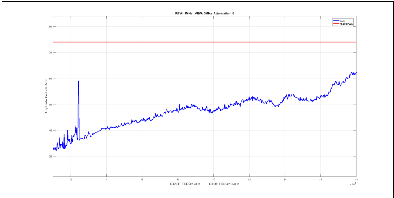
Plot 57. Radiated Emissions, Peak, radiated spurious emissions, 802.11n, BW 20M, CF 2412M, 1-18GHz
