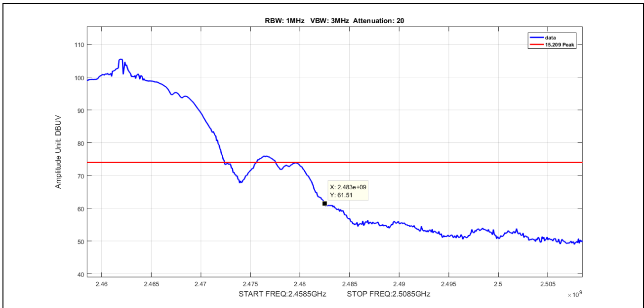
Plot 72. Radiated Emissions, Peak, 802.11b, 2483.5M radiated band edge, BW 20, CF 2462M
