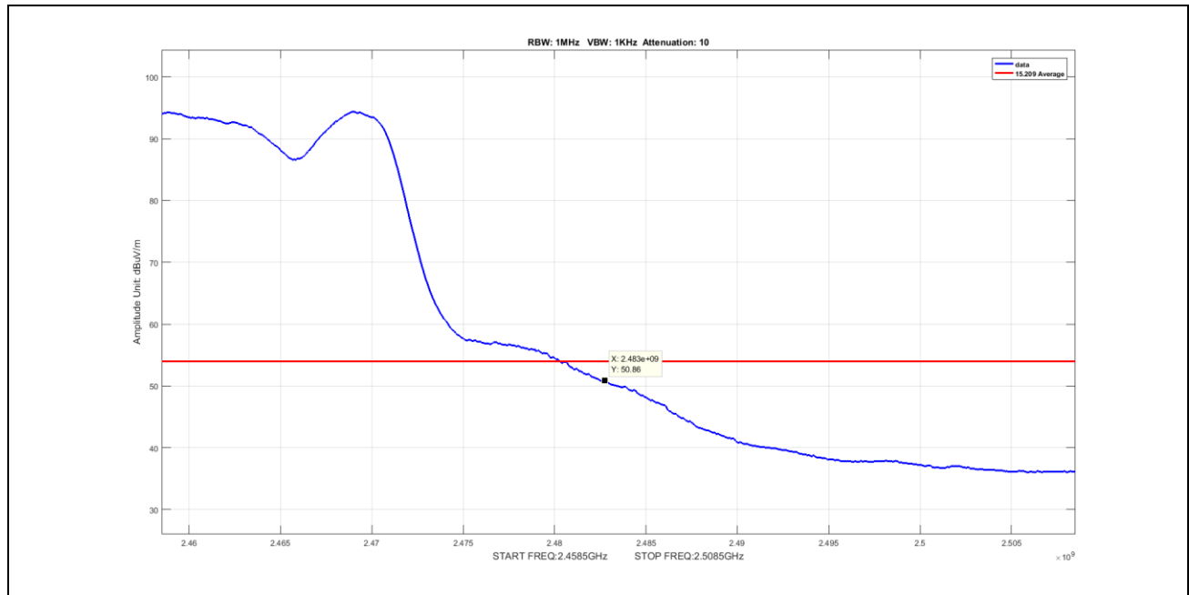
Plot 69. Radiated Emissions, Average, 2483.5M radiated band edge, 802.11n, BW 20, CF 2462
