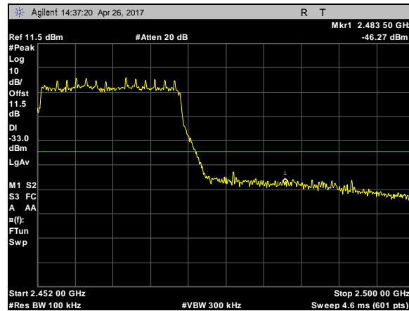
Plot 97. Spurious RF Conducted Emissions, 802.11n, 40M, CF 2452, high bandedge
