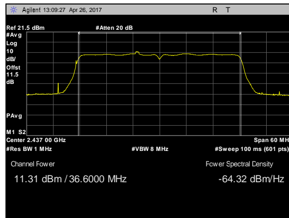
Plot 37. Peak Power Output, 802.11n, BW 40M, CF 2437M, c0
