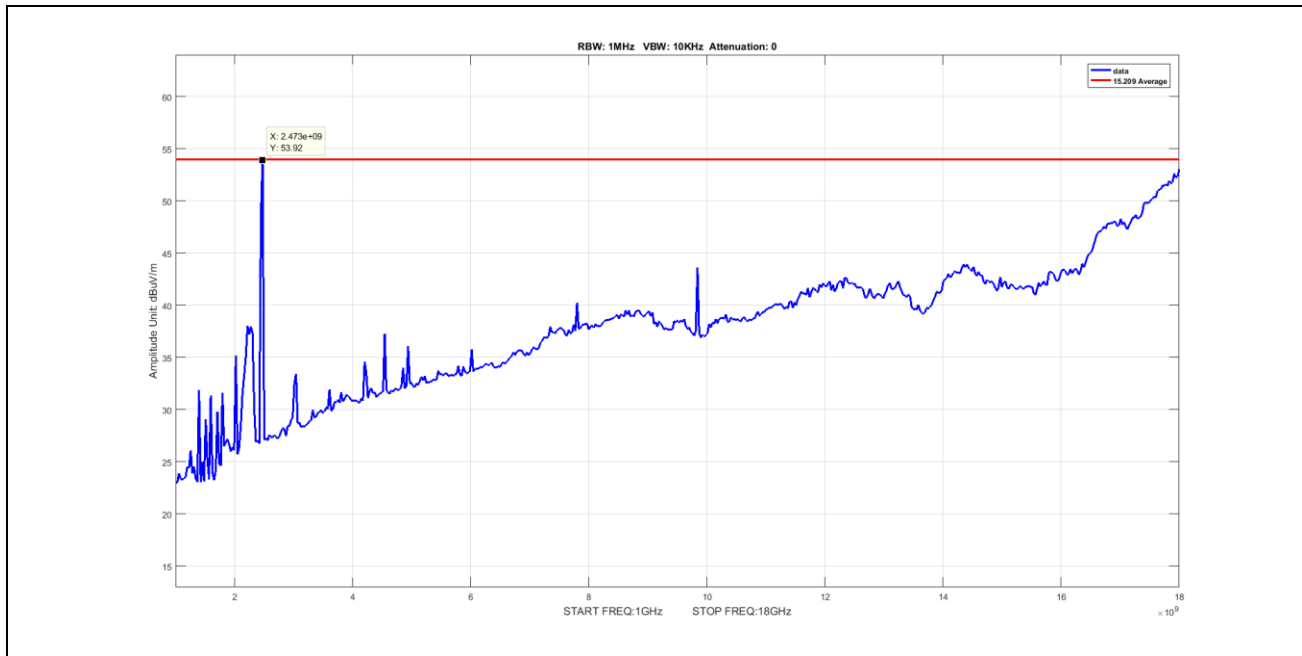
Plot 41. Radiated Emissions, Average, radiated spurious emissions, 802.11b, BW 20M, CF 2462M, 1-18GHz
