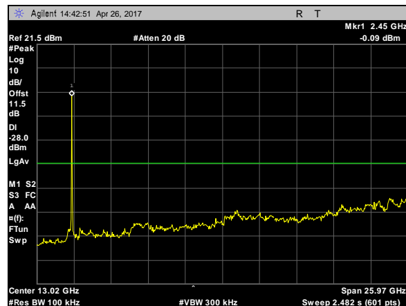
Plot 87. Spurious RF Conducted Emissions, 802.11n, 20M, CF 2462, 30MHz-26GHz
