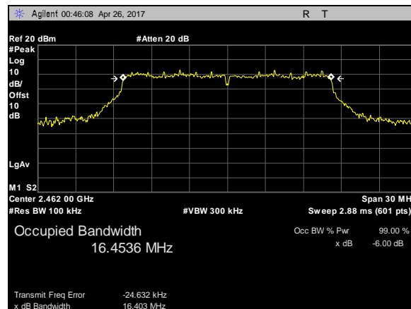
Plot 8. 6 dB Occupied DTS Bandwidth, 802.11g, BW 20M, CF 2462M
