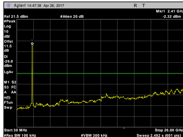
Plot 85. Spurious RF Conducted Emissions, 802.11n, 20M, CF 2412, 30MHz-26GHz
