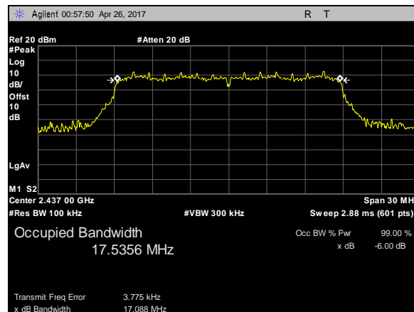
Plot 10. 6 dB Occupied DTS Bandwidth, 802.11n, BW 20M, CF 2437M
