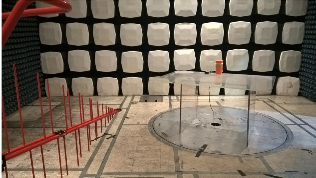
Photograph 2. Radiated Spurious Emissions, Test Setup below 1GHz
