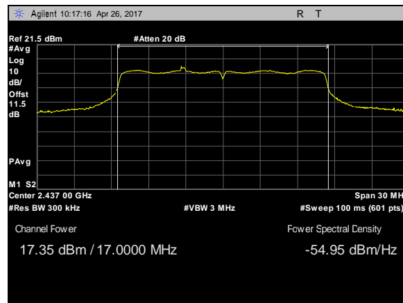
Plot 31. Peak Power Output, 802.11g, BW 20M, CF 2437M, c0
