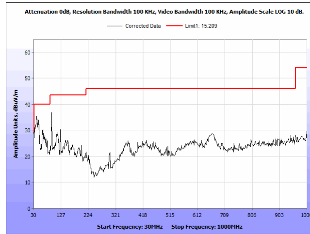
Radiated Emissions, Peak, radiated spurious emissions, 802.11g, BW 20M, CF 2437M, 30-1000MHz
