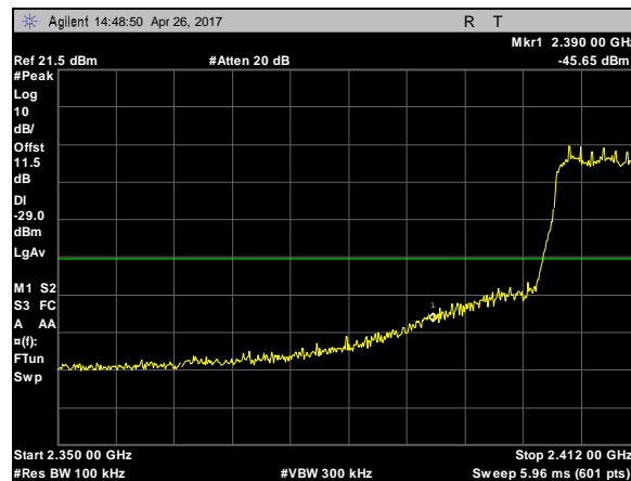
Plot 95. Spurious RF Conducted Emissions, 802.11n, 20M, CF 2412, low bandedge
