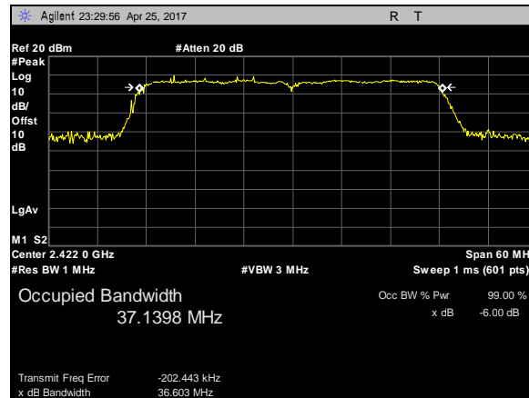
Plot 24. 99% Occupied Bandwidth, 802.11n, BW 40M, CF 2422M
