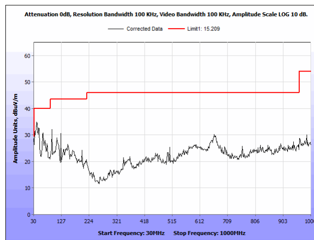
Radiated Emissions, Peak, radiated spurious emissions, 802.11b, BW 20M, CF 2437M, 30-1000MHz
