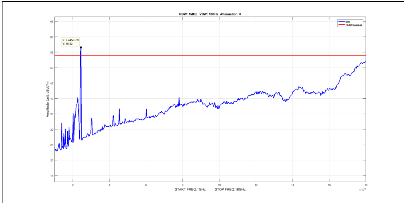
Plot 46. Radiated Emissions, Average, radiated spurious emissions, 802.11n, BW 20M, CF 2437M, 1-18GHz
