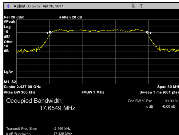
Plot 22. 99% Occupied Bandwidth, 802.11n, BW 20M, CF 2437M
