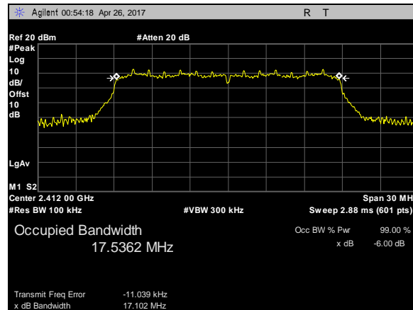
Plot 9. 6 dB Occupied DTS Bandwidth, 802.11n, BW 20M, CF 2412M
