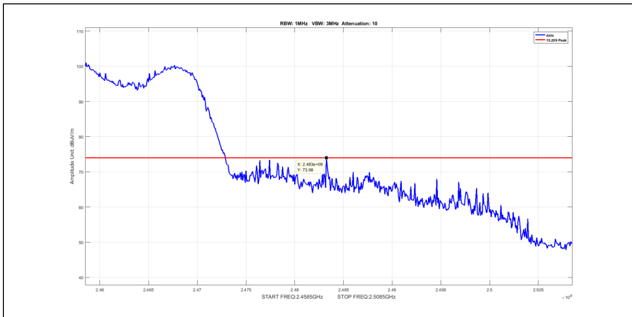
Plot 78. Radiated Emissions, Peak, 2483.5M radiated band edge, 802.11n, BW 40, CF 2452
