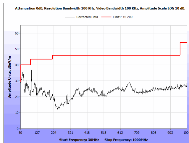
Radiated Emissions, Peak, radiated spurious emissions, 802.11g, BW 20M, CF 2462M, 30-1000MHz
