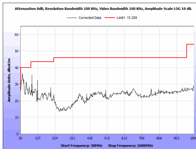
Radiated Emissions, Peak, radiated spurious emissions, 802.11n, BW 40M, CF 2437M, 30-1000MHz
