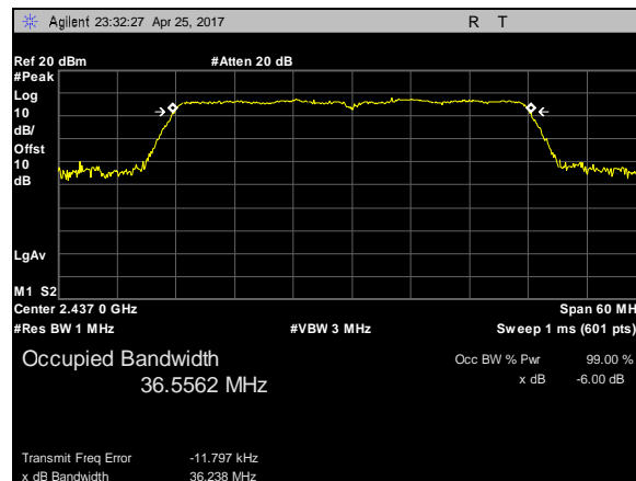
Plot 25. 99% Occupied Bandwidth, 802.11n, BW 40M, CF 2437M
