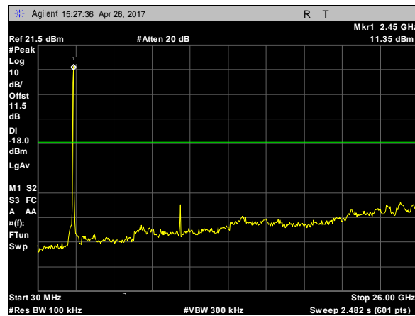
Plot 80. Spurious RF Conducted Emissions, 802.11b, 20M, CF 2437, 30MHz-26GHz
