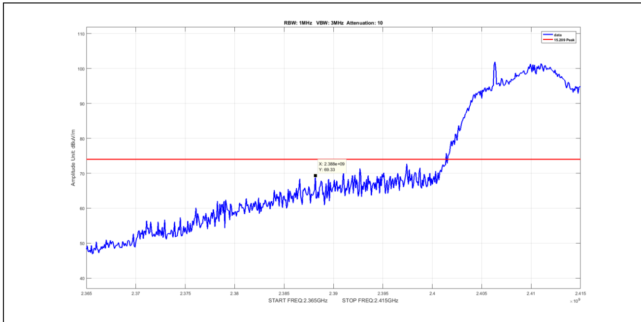
Plot 75. Radiated Emissions, Peak, 2390M radiated band edge, 802.11n, BW 40, CF 2422
