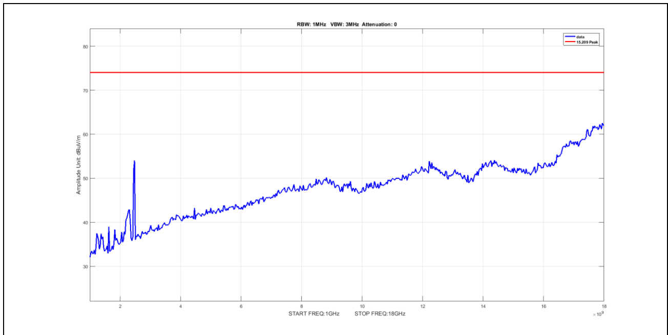
Plot 62. Radiated Emissions, Peak, radiated spurious emissions, 802.11n, BW 40M, CF 2452M, 1-18GHz
