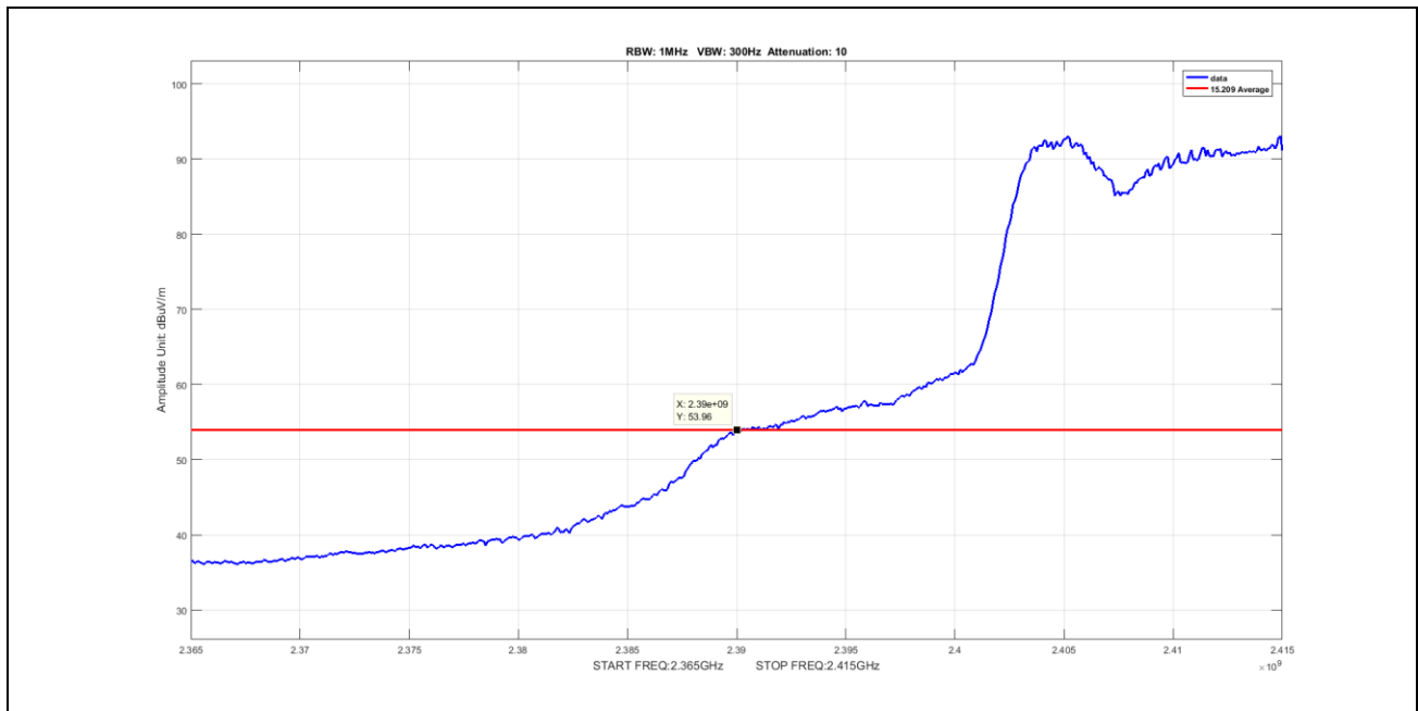
Plot 66. Radiated Emissions, Average, 2390M radiated band edge, 802.11n, BW 20, CF 2412
