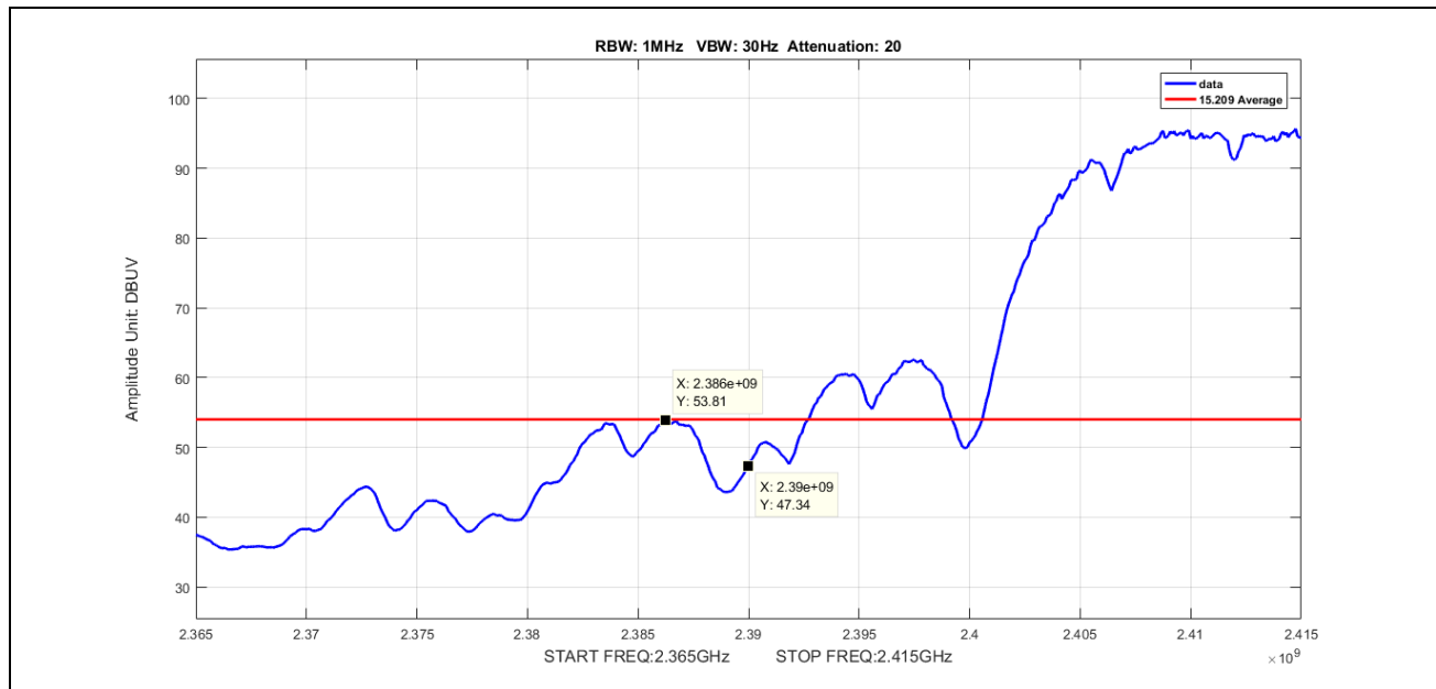
Plot 63. Radiated Emissions, Average, 802.11b, 2390M radiated band edge, BW 20, CF 2412M
