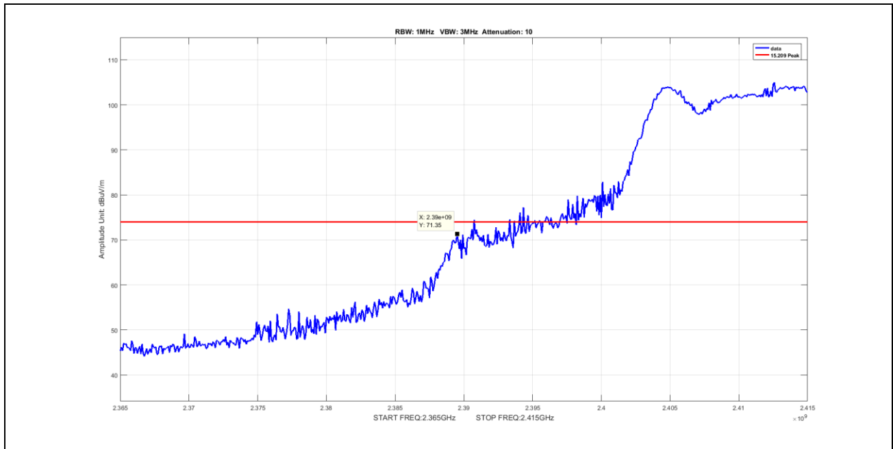
Plot 73. Radiated Emissions, Peak, 2390M radiated band edge, 802.11g, BW 20, CF 2412
