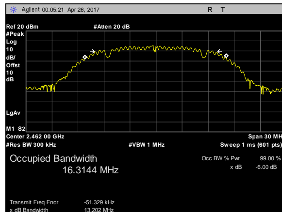
Plot 17. 99% Occupied Bandwidth, 802.11b, BW 20M, CF 2462M
