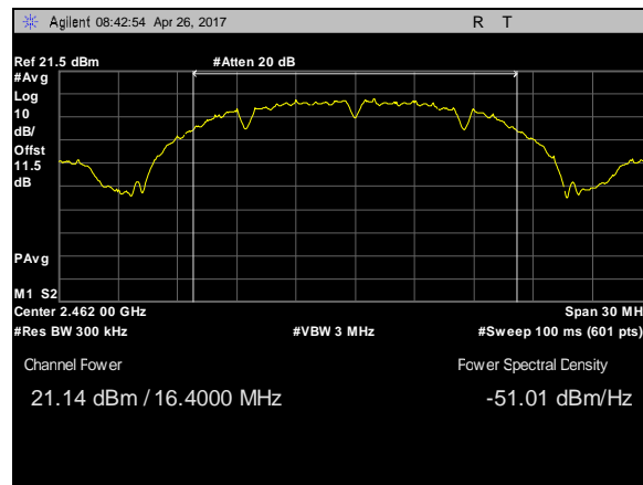
Plot 29. Peak Power Output, 802.11b, BW 20M, CF 2462M, c0
