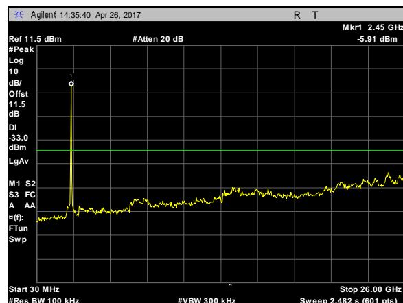
Plot 90. Spurious RF Conducted Emissions, 802.11n, 40M, CF 2452, 30MHz-26GHz
