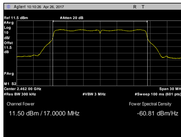
Plot 32. Peak Power Output, 802.11g, BW 20M, CF 2462M, c0
