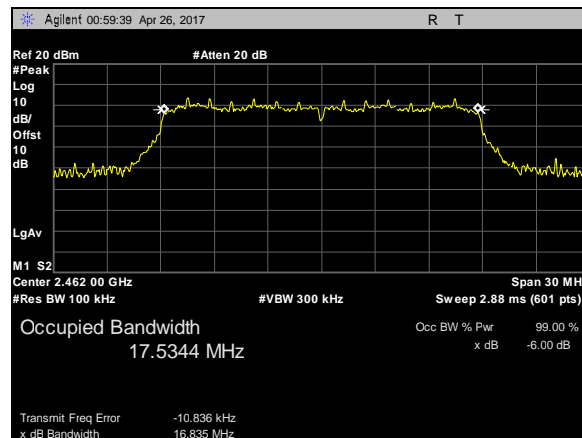
Plot 11. 6 dB Occupied DTS Bandwidth, 802.11n, BW 20M, CF 2462M
