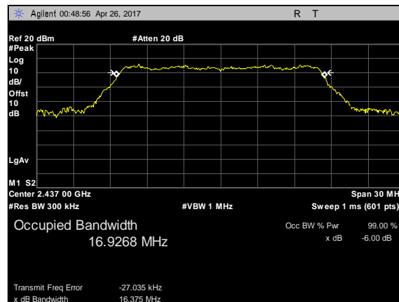
Plot 19. 99% Occupied Bandwidth, 802.11g, BW 20M, CF 2437M
