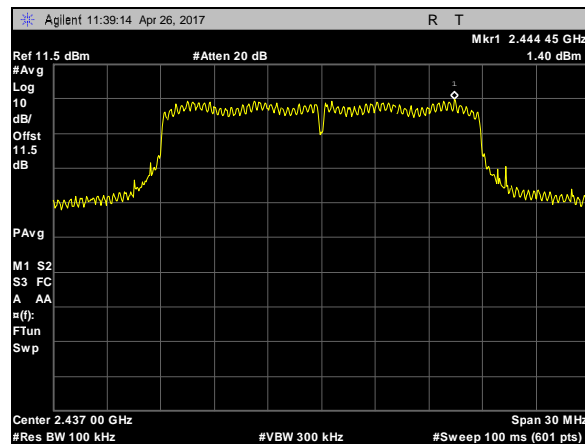
Plot 106. Power Spectral Density, 802.11n, BW 20M, CF 2437M, c0
