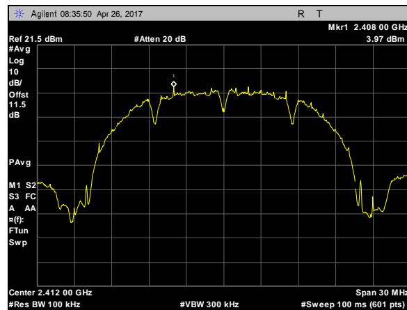
Plot 99. Power Spectral Density, 802.11b, BW 20M, CF 2412M, c0
