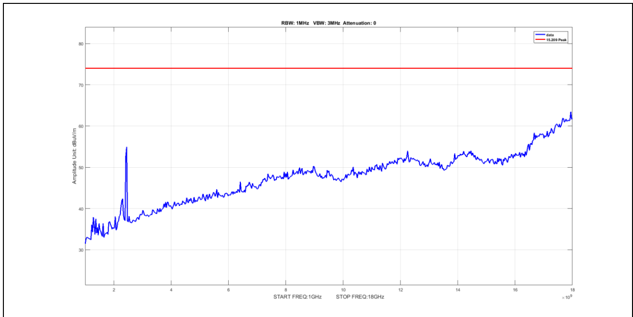
Plot 60. Radiated Emissions, Peak, radiated spurious emissions, 802.11n, BW 40M, CF 2422M, 1-18GHz
