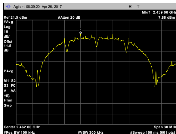
Plot 101. Power Spectral Density, 802.11b, BW 20M, CF 2462M, c0
