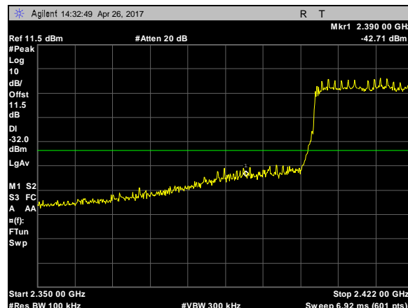
Plot 96. Spurious RF Conducted Emissions, 802.11n, 40M, CF 2422, low bandedge
