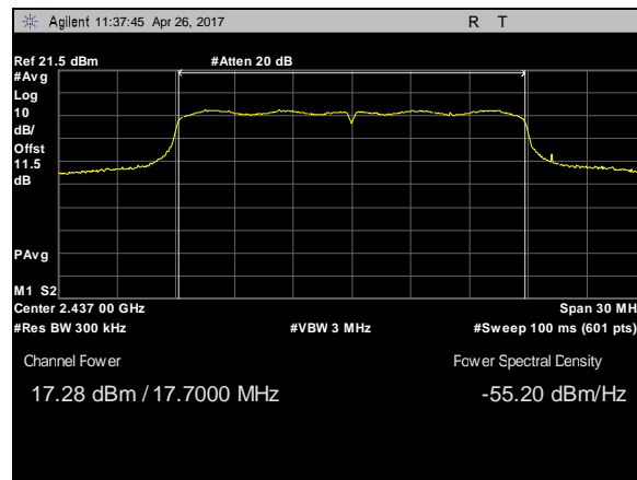
Plot 34. Peak Power Output, 802.11n, BW 20M, CF 2437M, c0
