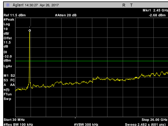
Plot 88. Spurious RF Conducted Emissions, 802.11n, 40M, CF 2422, 30MHz-26GHz
