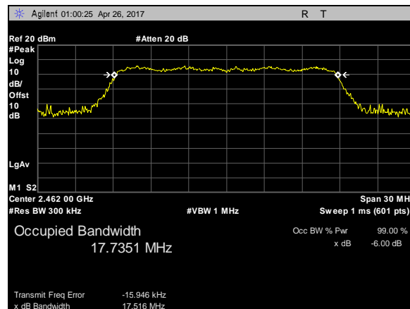
Plot 23. 99% Occupied Bandwidth, 802.11n, BW 20M, CF 2462M
