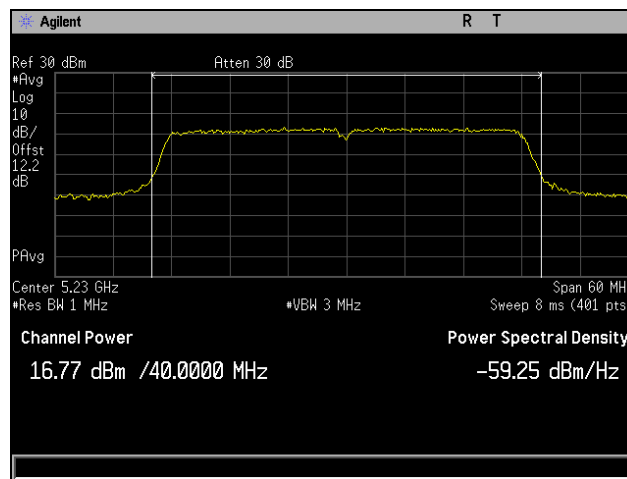
Plot 28. Output Power, 802.11n 40 MHz, Channel 5230 MHz, 4x8 MCS0 CH3
