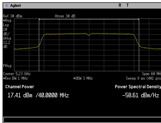
Plot 36. Output Power, 802.11ac 40 MHz, Channel 5230 MHz, 8x8 MCS0 NSS1 CH1
