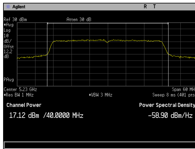
Plot 42. Output Power, 802.11n 40 MHz, Channel 5230 MHz, 8x8 MCS0 CH1
