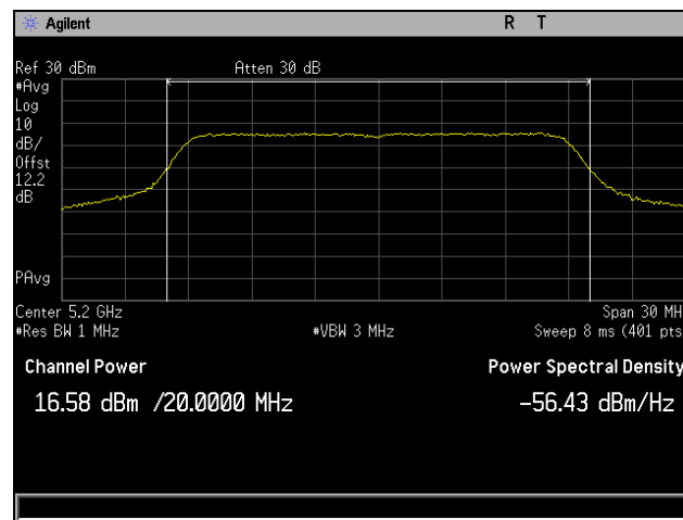
Plot 19. Output Power, 802.11ac 20 MHz, Channel 5200 MHz, 4x8 MCS0 CH3
