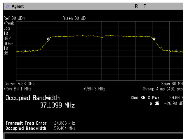
Plot 14. Occupied Bandwidth, 802.11n 40 MHz, Channel 5230 MHz, MCS0
