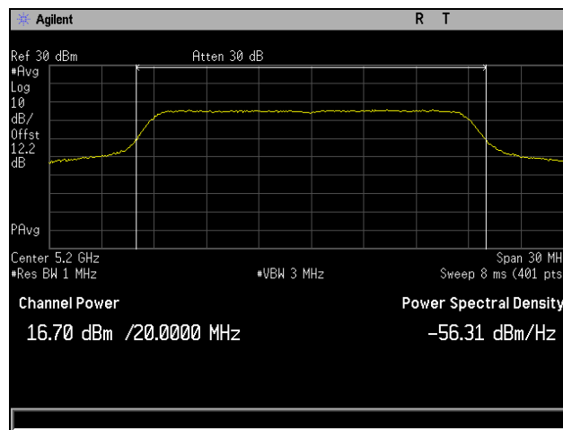
Plot 33. Output Power, 802.11ac 20 MHz, Channel 5200 MHz, 8x8 MCS0 NSS1 CH1
