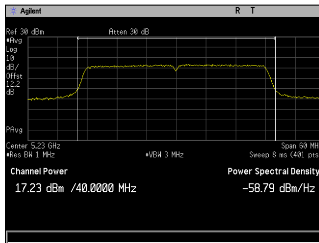
Plot 22. Output Power, 802.11ac 40 MHz, Channel 5230 MHz, 4x8 MCS0 CH3
