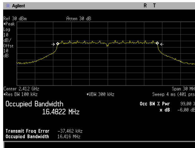
Plot 6. 6 dB Occupied Bandwidth, 802.11g 20 MHz, Channel 2412 MHz, 2x2, 6M
