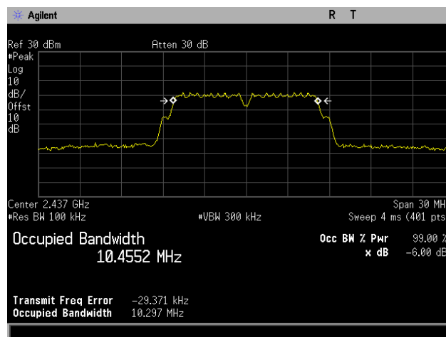
Plot 4. 6 dB Occupied Bandwidth, 802.11b, Channel 2437 MHz, 2x2, 1M
