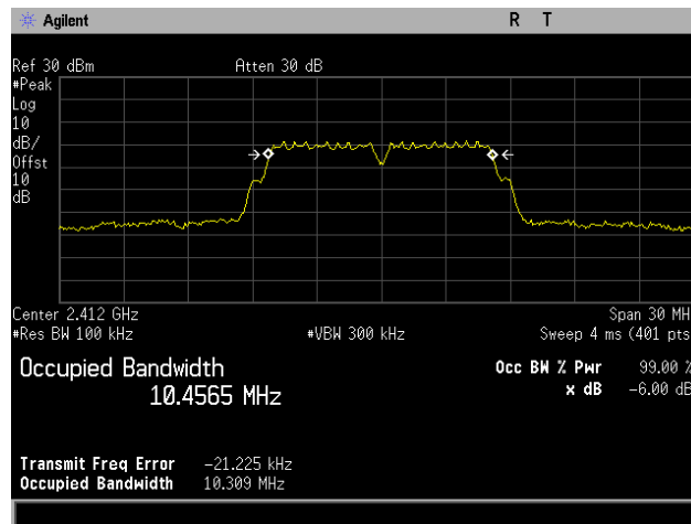
Plot 3. 6 dB Occupied Bandwidth, 802.11b, Channel 2412 MHz, 2x2, 1M
