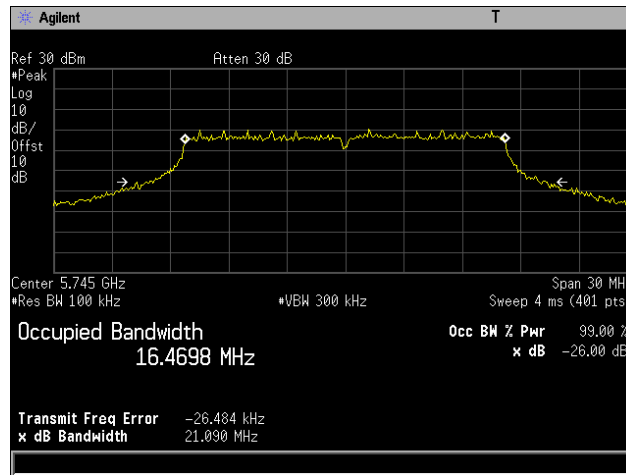
Plot 15. 26 dB Occupied Bandwidth, 802.11a 20 MHz, Channel 5745 MHz, 6x8, 6M
