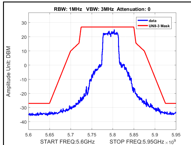
Plot 327. Radiated Spurious Emissions, Mask, 802.11ac 40 MHz, Channel 5795 MHz, 6x8, NSS1 MCS0
