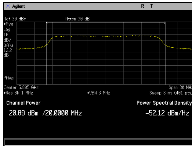
Plot 116. Conducted Output Power, 802.11ac 20 MHz, Channel 5805 MHz, 6x8, MCS0 NSS1, CH6
