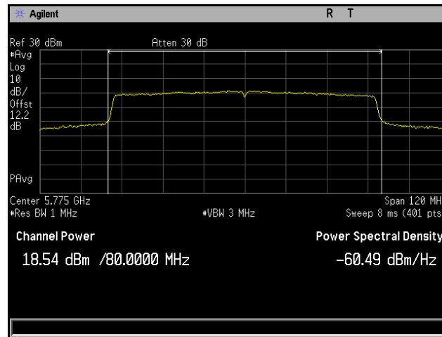
Plot 136. Conducted Output Power, 802.11ac 80 MHz, Channel 5775 MHz, 6x8, MCS0 NSS1, CH5
