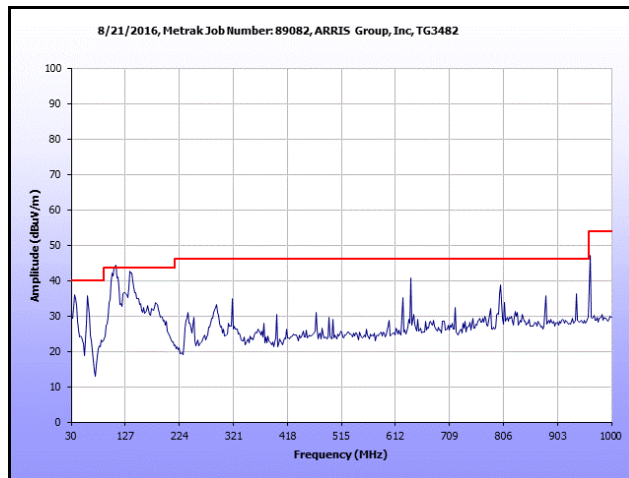
Plot 310. Radiated Spurious Emissions, 30 MHz – 1 GHz, Radio On
