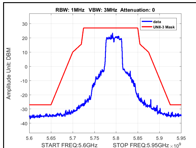
Plot 321. Radiated Spurious Emissions, Mask, 802.11n 40 MHz, Channel 5795 MHz, 4x8, MCS0
