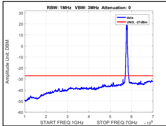
Plot 342. Radiated Spurious Emissions, 802.11n 40 MHz, Channel 5755 MHz, 4x8, MCS0, 1 GHz – 7 GHz
