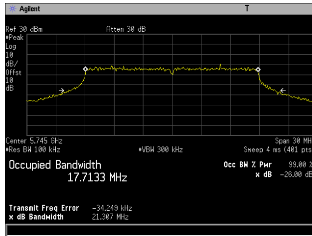
Plot 10. 26 dB Occupied Bandwidth, 802.11n 20 MHz, Channel 5745 MHz, 4x8, MCS0
