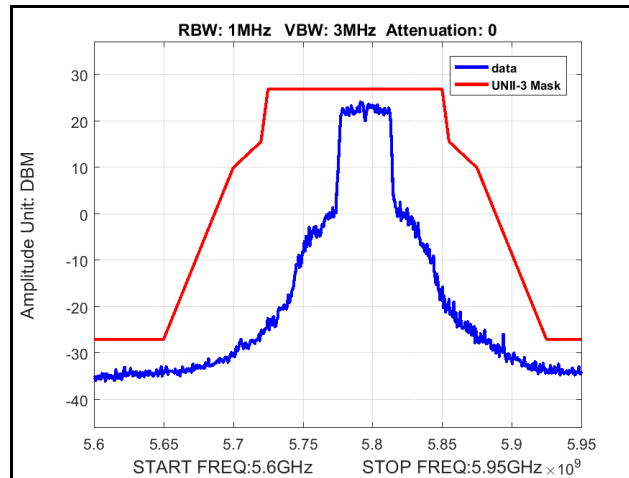
Plot 332. Radiated Spurious Emissions, Mask, 802.11n 40 MHz, Channel 5795 MHz, 6x8, MCS0
