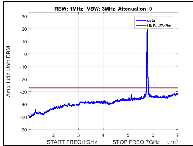
Plot 340. Radiated Spurious Emissions, 802.11n 20 MHz, Channel 5745 MHz, 4x8, MCS0, 1 GHz – 7 GHz
