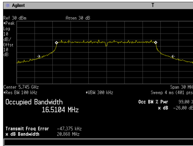
Plot 1. 26 dB Occupied Bandwidth, 802.11a 20 MHz, Channel 5745 MHz, 4x8, 6M
