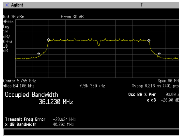
Plot 27. 26 dB Occupied Bandwidth, 802.11n 40 MHz, Channel 5755 MHz, 6x8, MCS0
