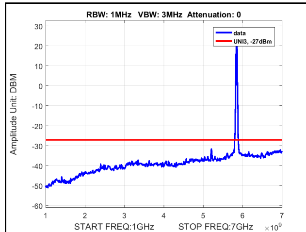
Plot 341. Radiated Spurious Emissions, 802.11n 20 MHz, Channel 5825 MHz, 4x8, MCS0, 1 GHz – 7 GHz
