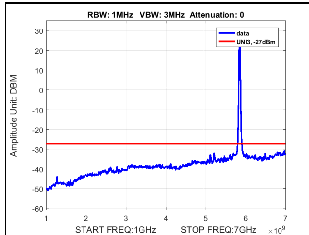
Plot 345. Radiated Spurious Emissions, 802.11a 20 MHz, Channel 5825 MHz, 6x8, 6M, 1 GHz – 7 GHz
