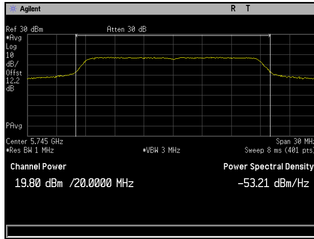
Plot 151. Conducted Output Power, 802.11n 20 MHz, Channel 5745 MHz, 6x8, MCS0 NSS1, CH6
