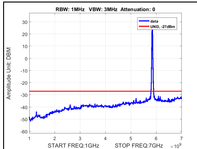
Plot 352. Radiated Spurious Emissions, 802.11n 20 MHz, Channel 5825 MHz, 6x8, MCS0, 1 GHz – 7 GHz
