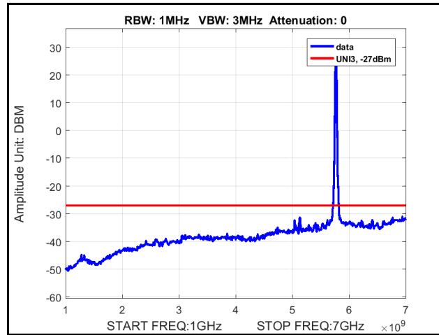
Plot 344. Radiated Spurious Emissions, 802.11a 20 MHz, Channel 5745 MHz, 6x8, 6M, 1 GHz – 7 GHz
