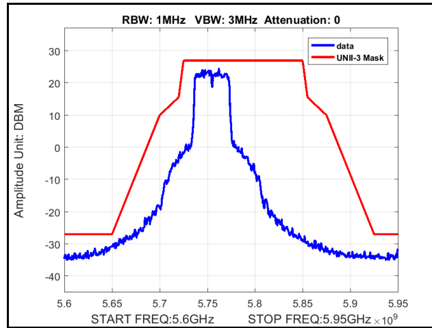
Plot 326. Radiated Spurious Emissions, Mask, 802.11ac 40 MHz, Channel 5755 MHz, 6x8, NSS1 MCS0
