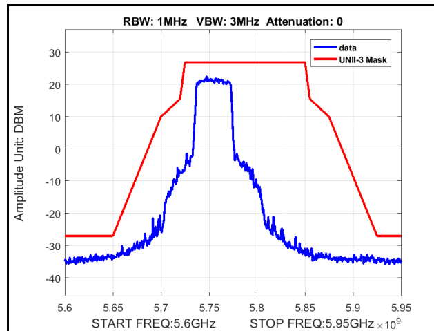
Plot 320. Radiated Spurious Emissions, Mask, 802.11n 40 MHz, Channel 5755 MHz, 4x8, MCS0
