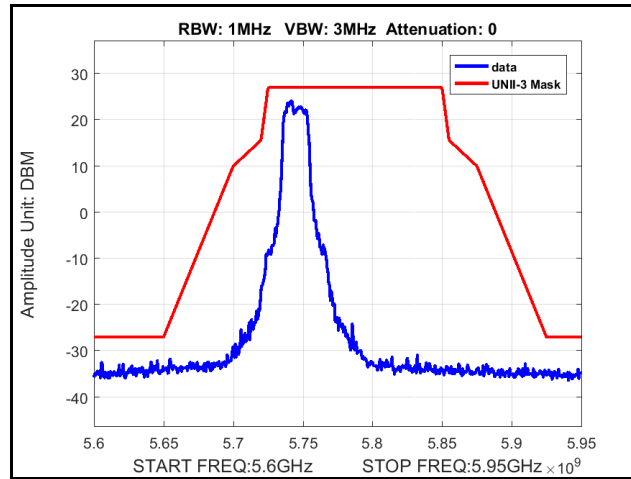
Plot 318. Radiated Spurious Emissions, Mask, 802.11n 20 MHz, Channel 5745 MHz, 4x8, MCS0
