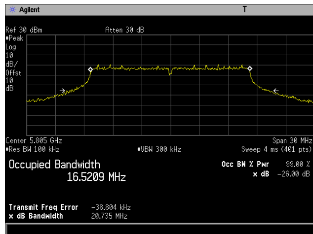
Plot 16. 26 dB Occupied Bandwidth, 802.11a 20 MHz, Channel 5805 MHz, 6x8, 6M
