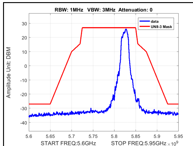
Plot 312. Radiated Spurious Emissions, Mask, 802.11a 20 MHz, Channel 5825 MHz, 4x8, 6M
