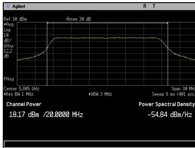
Plot 140. Conducted Output Power, 802.11n 20 MHz, Channel 5805 MHz, 6x8, MCS0 NSS1, CH2
