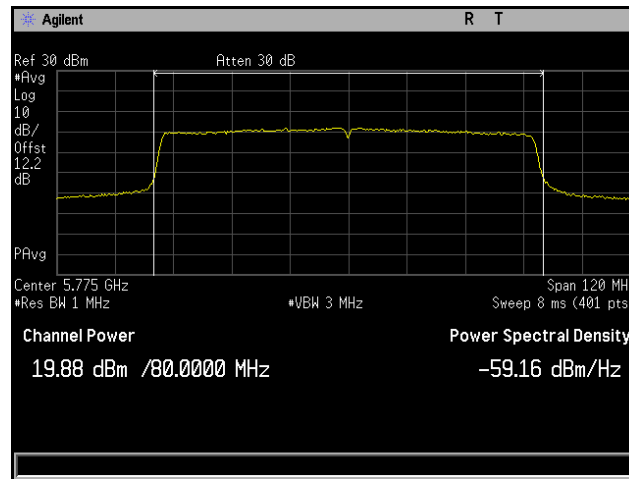
Plot 134. Conducted Output Power, 802.11ac 80 MHz, Channel 5775 MHz, 6x8, MCS0 NSS1, CH3
