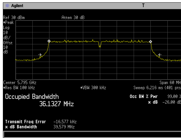
Plot 28. 26 dB Occupied Bandwidth, 802.11n 40 MHz, Channel 5795 MHz, 6x8, MCS0
