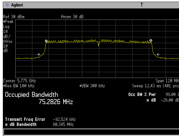
Plot 23. 26 dB Occupied Bandwidth, 802.11ac 80 MHz, Channel 5775 MHz, 6x8, NSS1 MCS0
