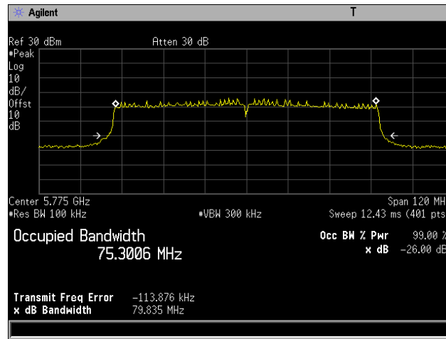
Plot 9. 26 dB Occupied Bandwidth, 802.11ac 80 MHz, Channel 5775 MHz, 4x8, NSS1 MCS0
