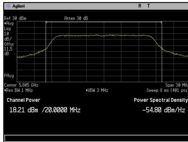
Plot 30. Conducted Output Power, 802.11a 20 MHz, Channel 5805 MHz, 4x8, 6M, CH3
