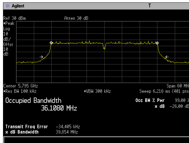
Plot 22. 26 dB Occupied Bandwidth, 802.11ac 40 MHz, Channel 5795 MHz, 6x8, NSS1 MCS0
