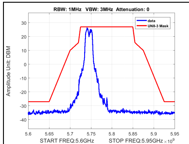
Plot 311. Radiated Spurious Emissions, Mask, 802.11a 20 MHz, Channel 5745 MHz, 4x8, 6M
