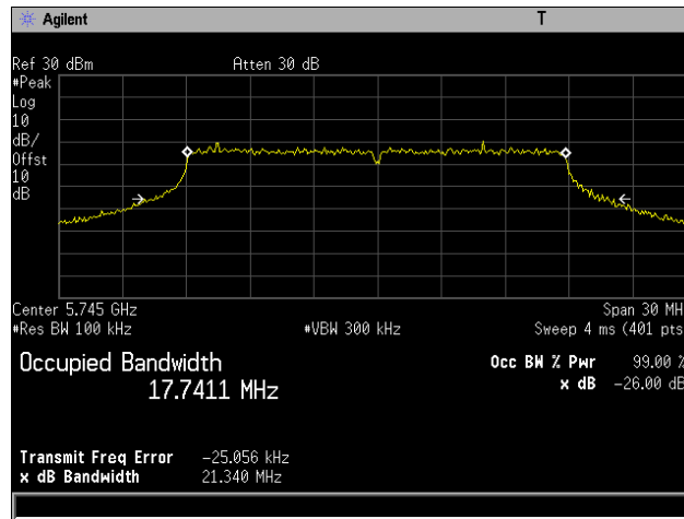
Plot 4. 26 dB Occupied Bandwidth, 802.11ac 20 MHz, Channel 5745 MHz, 4x8, NSS1 MCS0
