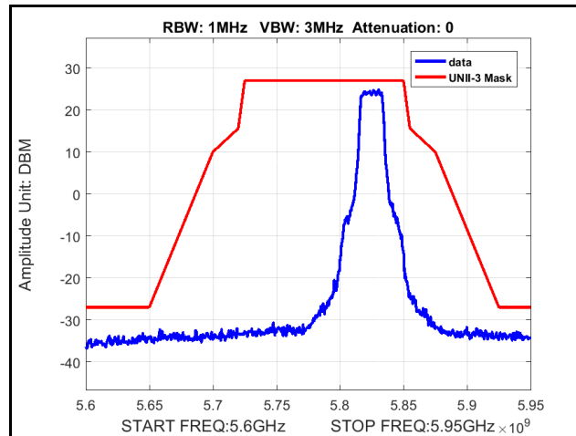
Plot 314. Radiated Spurious Emissions, Mask, 802.11ac 20 MHz, Channel 5825 MHz, 4x8, NSS1 MCS0
