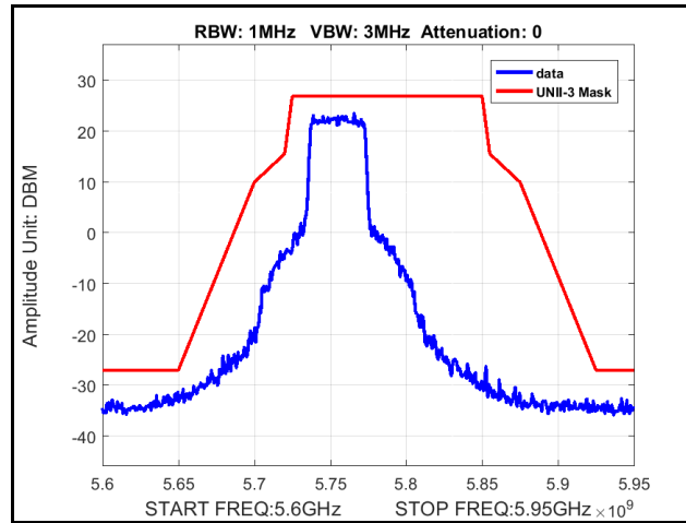
Plot 331. Radiated Spurious Emissions, Mask, 802.11n 40 MHz, Channel 5755 MHz, 6x8, MCS0
