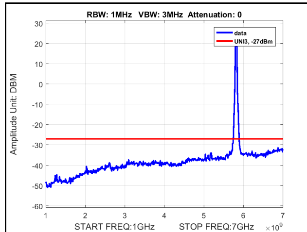
Plot 343. Radiated Spurious Emissions, 802.11n 40 MHz, Channel 5795 MHz, 4x8, MCS0, 1 GHz – 7 GHz
