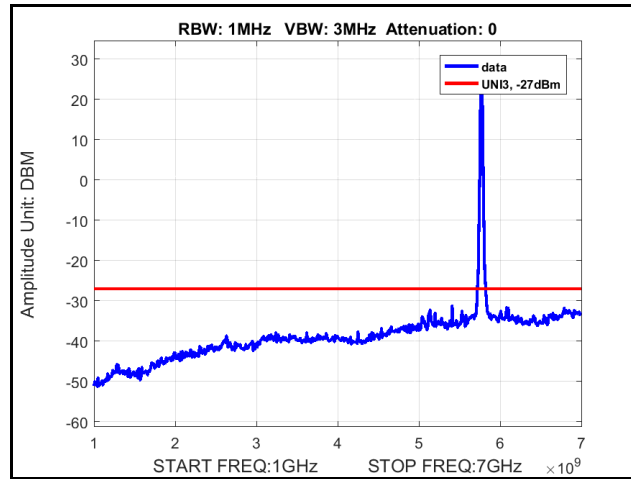
Plot 351. Radiated Spurious Emissions, 802.11n 20 MHz, Channel 5745 MHz, 6x8, MCS0, 1 GHz – 7 GHz
