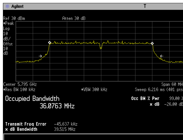
Plot 8. 26 dB Occupied Bandwidth, 802.11ac 40 MHz, Channel 5795 MHz, 4x8, NSS1 MCS0
