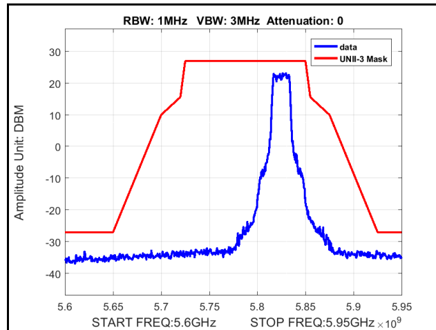
Plot 319. Radiated Spurious Emissions, Mask, 802.11n 20 MHz, Channel 5825 MHz, 4x8, MCS0
