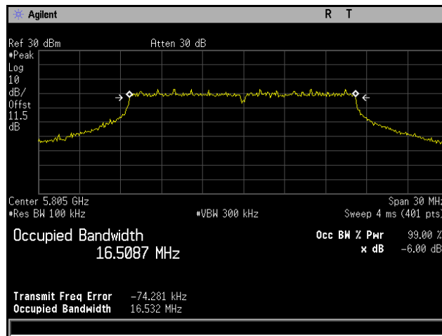
Plot 358. 6 dB Occupied Bandwidth, 802.11a 20 MHz, Channel 5805 MHz, 4x8, 6M
