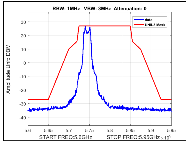
Plot 313. Radiated Spurious Emissions, Mask, 802.11ac 20 MHz, Channel 5745 MHz, 4x8, NSS1 MCS0
