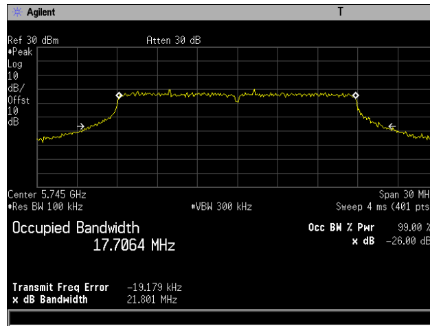
Plot 24. 26 dB Occupied Bandwidth, 802.11n 20 MHz, Channel 5745 MHz, 6x8, MCS0
