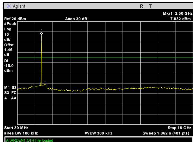
Plot 25. Conducted Spurious Emissions, High Channel
