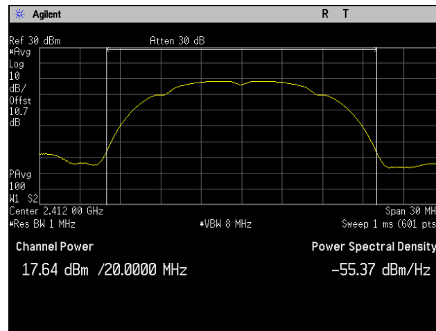
Plot 15. Peak Power Output, Low Channel, 802.11b 20 MHz, Port 2
