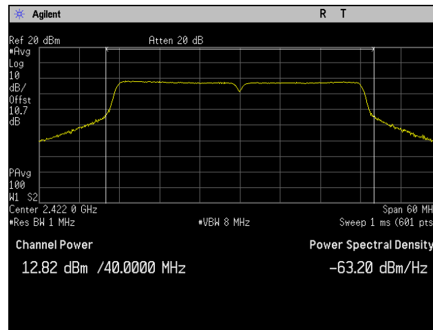
Plot 12. Peak Power Output, Low Channel, 802.11n 40 MHz, Port 1
