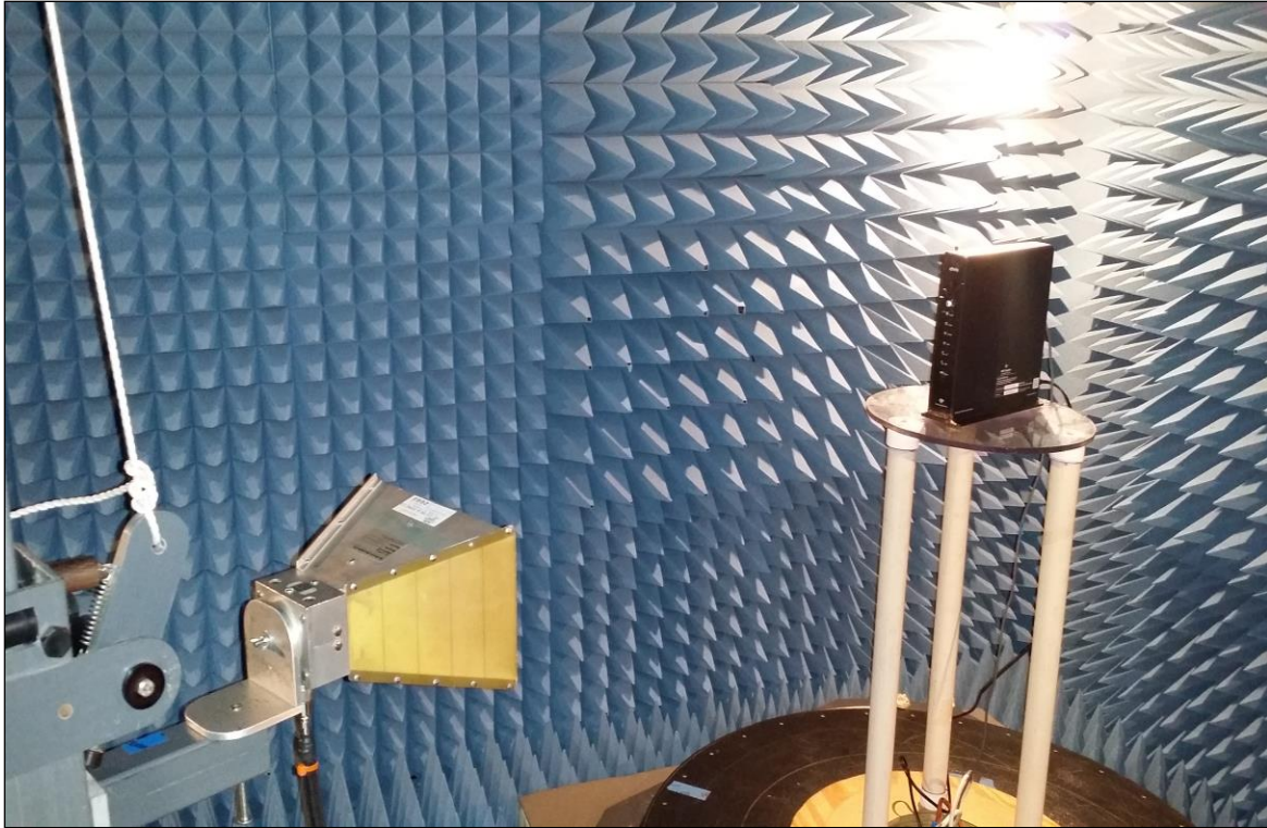
Photograph 3. DFS, Test Setup
