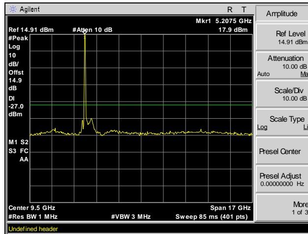
Plot 50. Radiated Spurious Emissions, Above 1 GHz, Channel 36, 802.11ac 40 MHz
