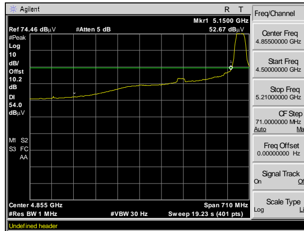
Plot 72. Radiated Band Edge, Average, Channel 36, 802.11a 20 MHz
