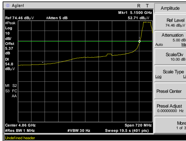
Plot 78. Radiated Band Edge, Average, Channel 36, 802.11ac 40 MHz
