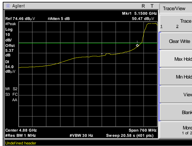
Plot 79. Radiated Band Edge, Average, Channel 44, 802.11ac 40 MHz
