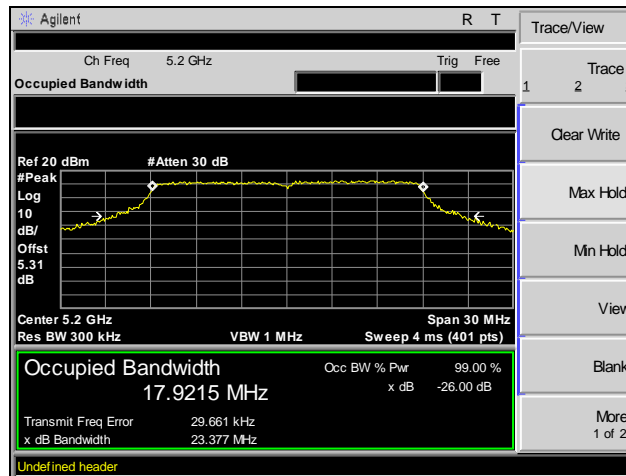
Plot 5. 26 dB Occupied Bandwidth, Channel 40, 802.11ac 20 MHz
