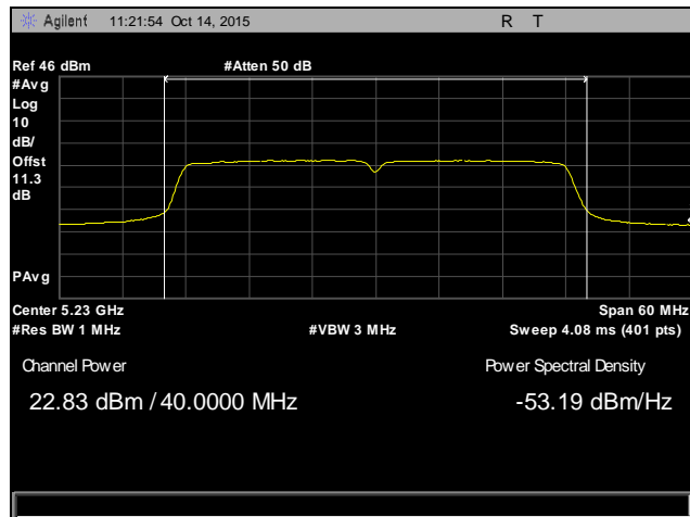
Plot 28. Maximum Conducted Output Power, Channel 46, 802.11n 40 MHz
