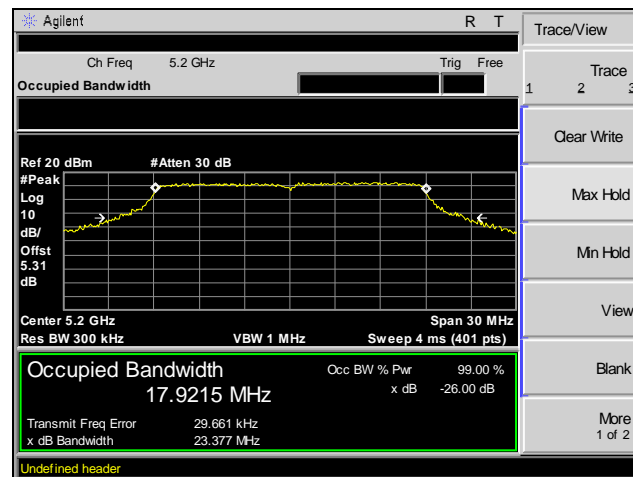
Plot 2. 26 dB Occupied Bandwidth, Channel 40, 802.11a 20 MHz
