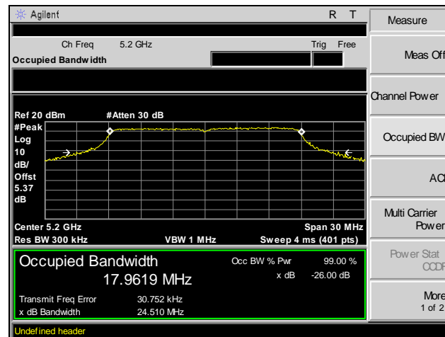
Plot 11. 26 dB Occupied Bandwidth, Channel 40, 802.11n 20 MHz
