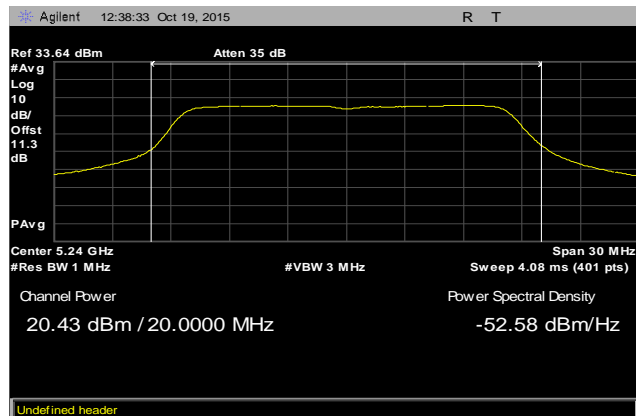
Plot 17. Maximum Conducted Output Power, Channel 48, 802.11a 20 MHz
