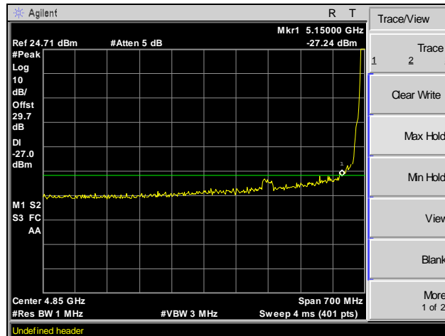
Plot 59. Radiated Band Edge, -27 dBm, Channel 40, 802.11a 20 MHz
