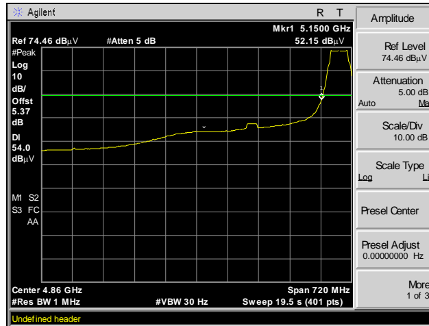
Plot 84. Radiated Band Edge, Average, Channel 36, 802.11n 40 MHz
