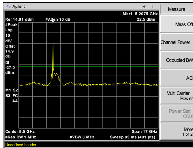
Plot 53. Radiated Spurious Emissions, Above 1 GHz, Channel 36, 802.11n 20 MHz
