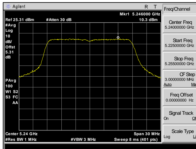
Plot 40. Peak Power Spectral Density, Channel 48, 802.11n 20 MHz
