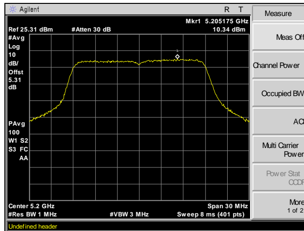
Plot 39. Peak Power Spectral Density, Channel 40, 802.11n 20 MHz
