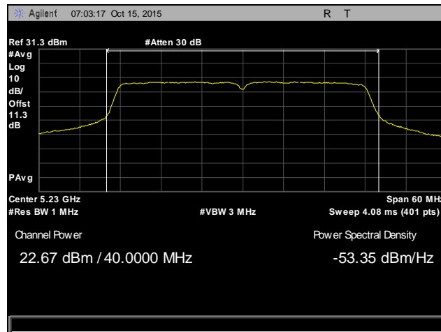
Plot 22. Maximum Conducted Output Power, Channel 46, 802.11ac 40 MHz
