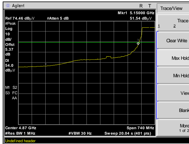
Plot 80. Radiated Band Edge, Average, Channel 36, 802.11ac 80 MHz
