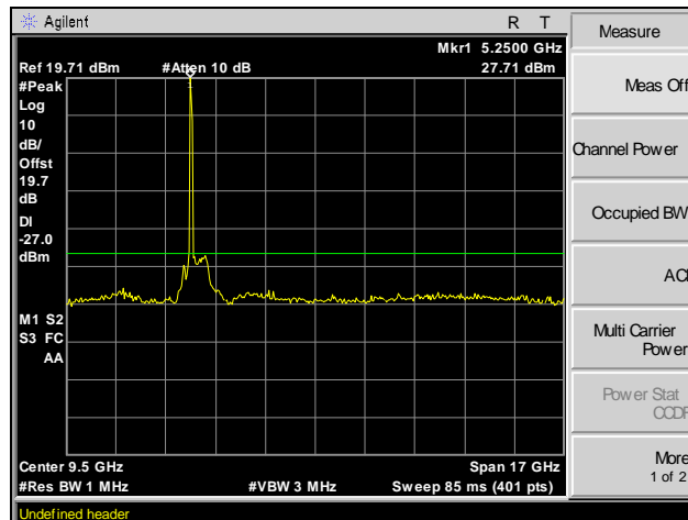
Plot 46. Radiated Spurious Emissions, Above 1 GHz, Channel 48, 802.11a 20 MHz
