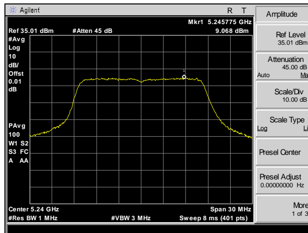
Plot 31. Peak Power Spectral Density, Channel 48, 802.11a 20 MHz
