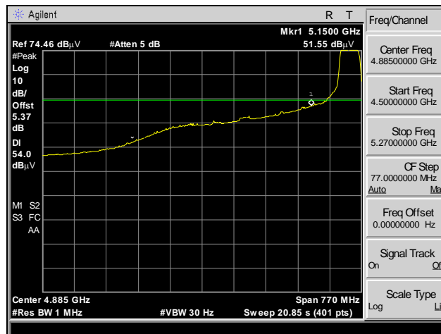
Plot 83. Radiated Band Edge, Average, Channel 48, 802.11n 20 MHz
