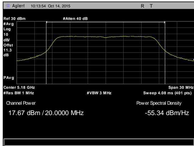
Plot 15. Maximum Conducted Output Power, Channel 36, 802.11a 20 MHz
