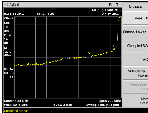
Plot 68. Radiated Band Edge, -27 dBm, Channel 40, 802.11n 20 MHz
