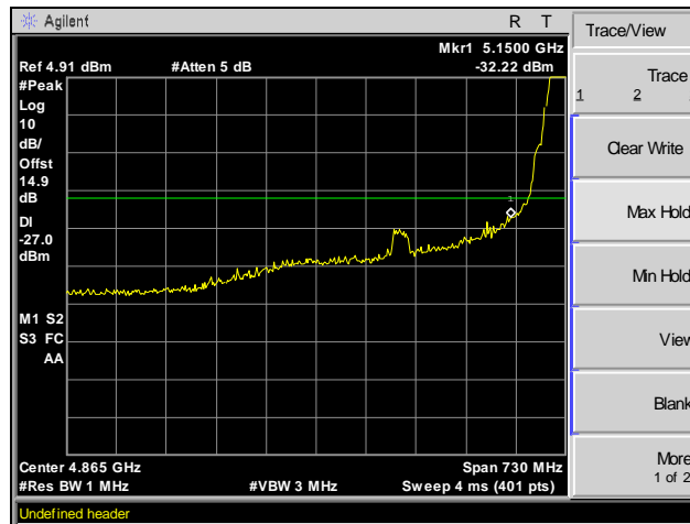
Plot 65. Radiated Band Edge, -27 dBm, Channel 44, 802.11ac 40 MHz
