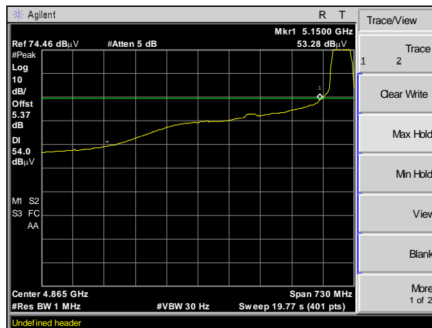
Plot 76. Radiated Band Edge, Average, Channel 40, 802.11ac 20 MHz
