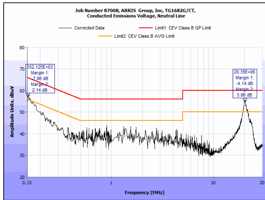
Plot 87. Conducted Emissions, Neutral Line
