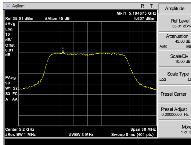
Plot 30. Peak Power Spectral Density, Channel 40, 802.11a 20 MHz
