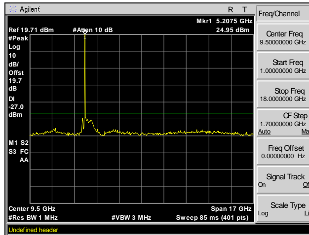
Plot 44. Radiated Spurious Emissions, Above 1 GHz, Channel 36, 802.11a 20 MHz
