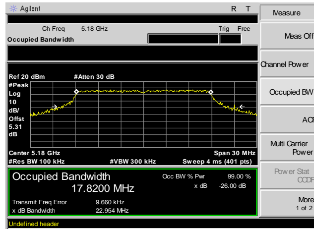
Plot 1. 26 dB Occupied Bandwidth, Channel 36, 802.11a 20 MHz
