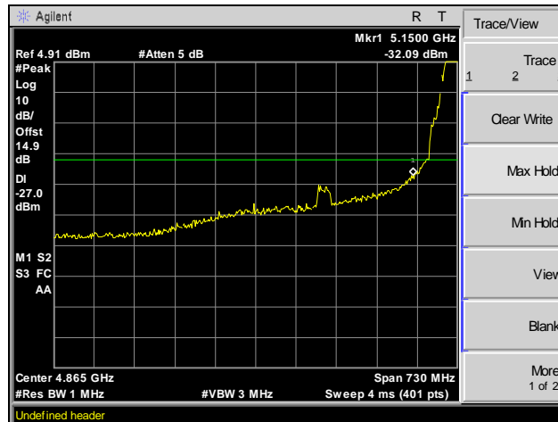
Plot 71. Radiated Band Edge, -27 dBm, Channel 44, 802.11n 40 MHz
