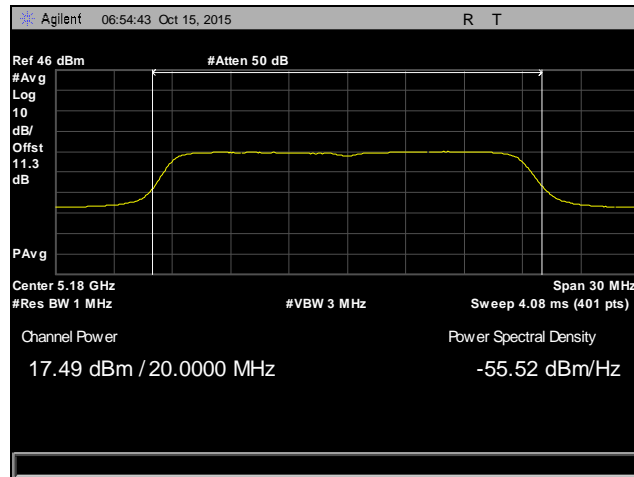
Plot 18. Maximum Conducted Output Power, Channel 36, 802.11ac 20 MHz
