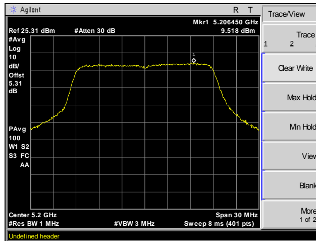
Plot 33. Peak Power Spectral Density, Channel 40, 802.11ac 20 MHz
