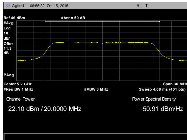
Plot 19. Maximum Conducted Output Power, Channel 40, 802.11ac 20 MHz
