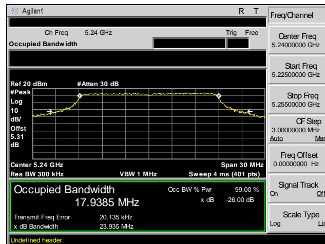
Plot 3. 26 dB Occupied Bandwidth, Channel 48, 802.11a 20 MHz
