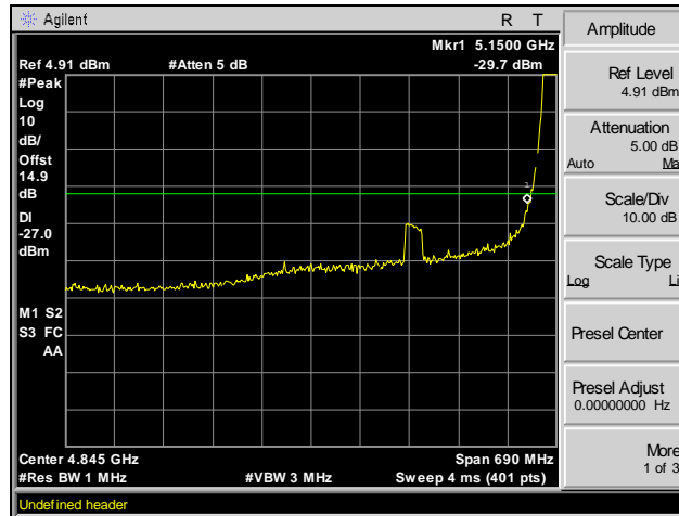
Plot 70. Radiated Band Edge, -27 dBm, Channel 36, 802.11n 40 MHz
