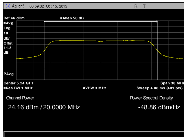
Plot 20. Maximum Conducted Output Power, Channel 48, 802.11ac 20 MHz
