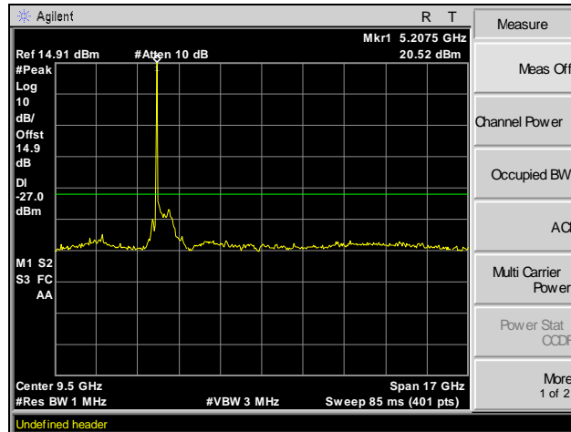
Plot 47. Radiated Spurious Emissions, Above 1 GHz, Channel 36, 802.11ac 20 MHz
