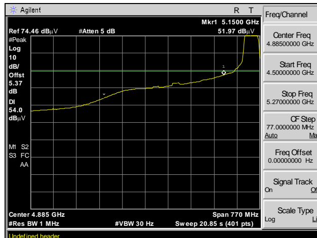
Plot 77. Radiated Band Edge, Average, Channel 48, 802.11ac 20 MHz
