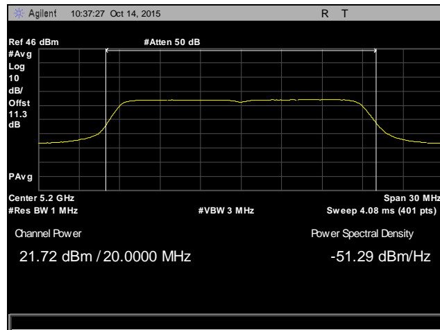
Plot 25. Maximum Conducted Output Power, Channel 40, 802.11n 20 MHz
