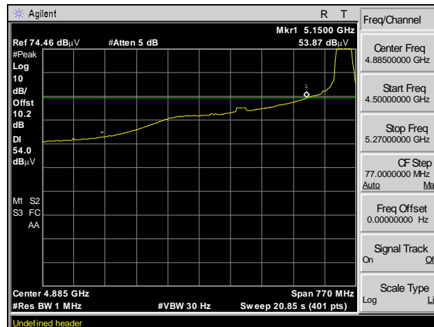
Plot 74. Radiated Band Edge, Average, Channel 48, 802.11a 20 MHz
