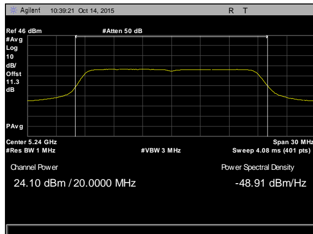
Plot 26. Maximum Conducted Output Power, Channel 48, 802.11n 20 MHz
