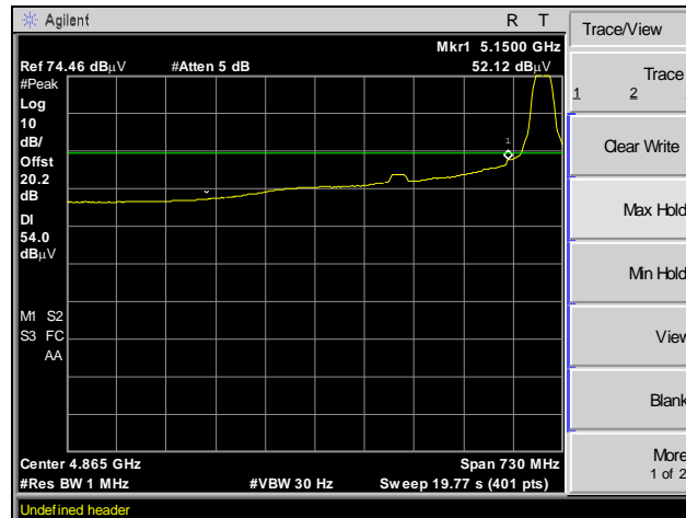
Plot 73. Radiated Band Edge, Average, Channel 40, 802.11a 20 MHz
