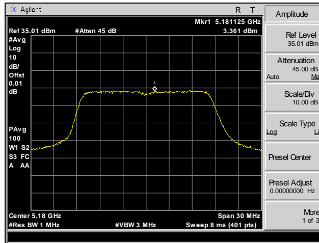
Plot 29. Peak Power Spectral Density, Channel 36, 802.11a 20 MHz
