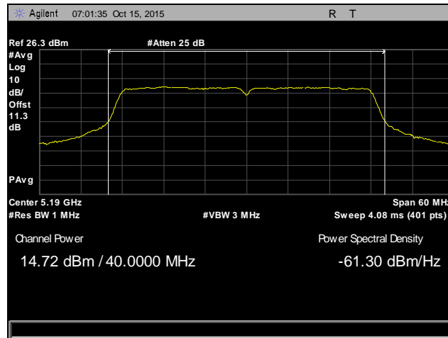
Plot 21. Maximum Conducted Output Power, Channel 38, 802.11ac 40 MHz
