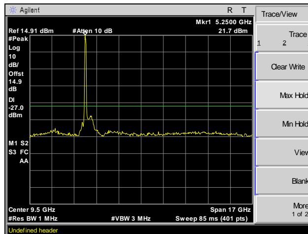
Plot 57. Radiated Spurious Emissions, Above 1 GHz, Channel 44, 802.11n 40 MHz
