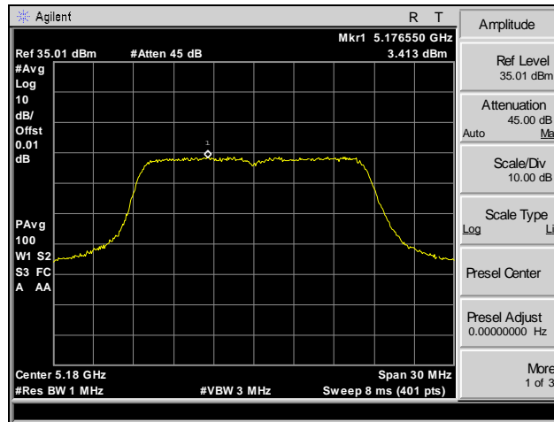
Plot 32. Peak Power Spectral Density, Channel 36, 802.11ac 20 MHz
