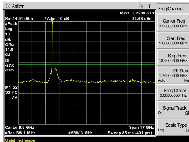
Plot 49. Radiated Spurious Emissions, Above 1 GHz, Channel 48, 802.11ac 20 MHz
