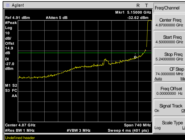
Plot 63. Radiated Band Edge, -27 dBm, Channel 48, 802.11ac 20 MHz
