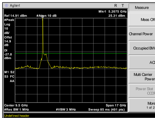
Plot 54. Radiated Spurious Emissions, Above 1 GHz, Channel 40, 802.11n 20 MHz
