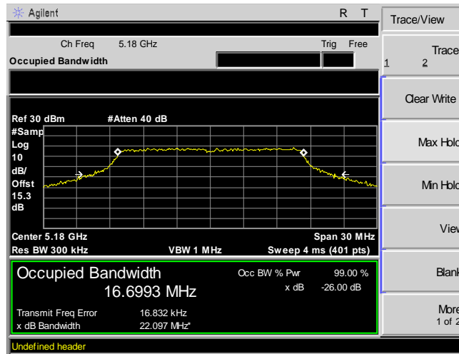
Plot 10. 26 dB Occupied Bandwidth, Channel 36, 802.11n 20 MHz
