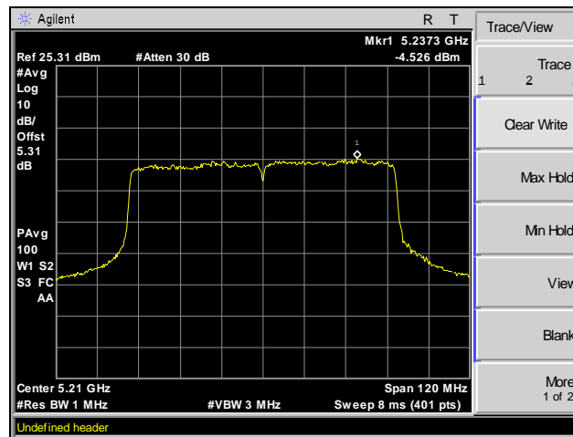
Plot 37. Peak Power Spectral Density, Channel 36, 802.11ac 80 MHz
