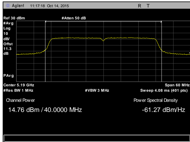
Plot 27. Maximum Conducted Output Power, Channel 38, 802.11n 40 MHz
