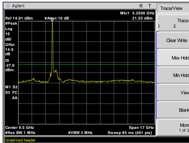
Plot 51. Radiated Spurious Emissions, Above 1 GHz, Channel 44, 802.11ac 40 MHz
