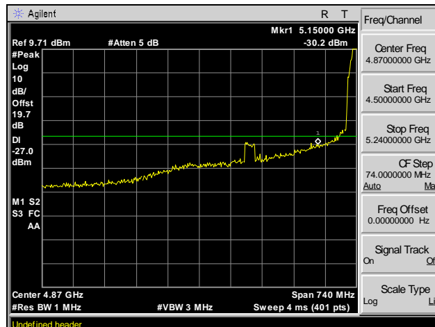
Plot 60. Radiated Band Edge, -27 dBm, Channel 48, 802.11a 20 MHz
