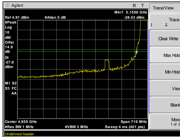
Plot 66. Radiated Band Edge, -27 dBm, Channel 36, 802.11ac 80 MHz
