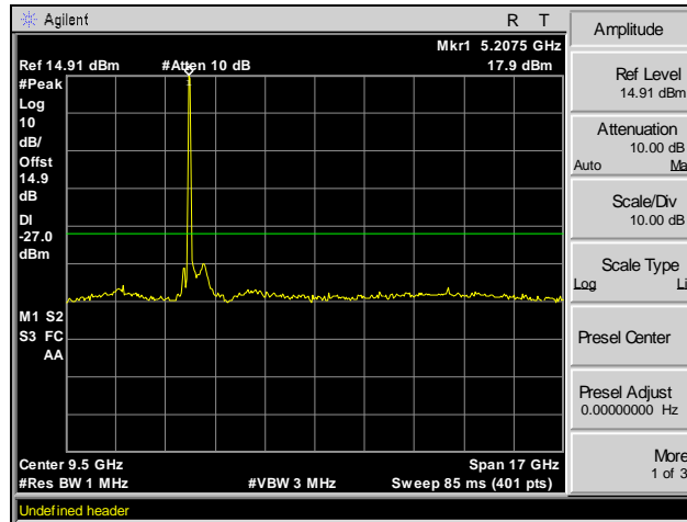
Plot 56. Radiated Spurious Emissions, Above 1 GHz, Channel 36, 802.11n 40 MHz
