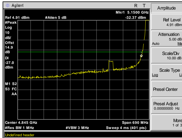
Plot 64. Radiated Band Edge, -27 dBm, Channel 36, 802.11ac 40 MHz
