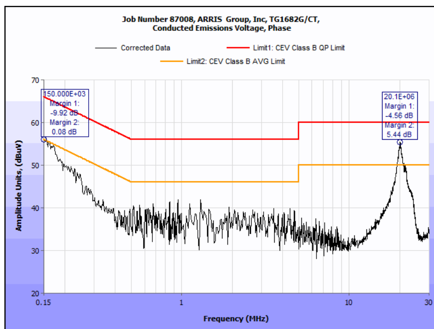
Plot 86. Conducted Emissions, Phase Line
