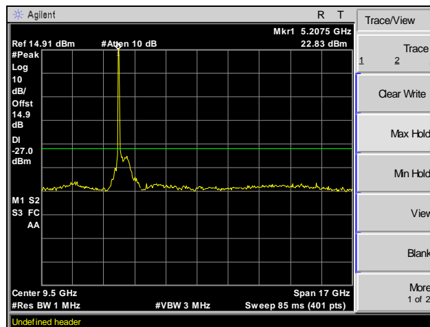
Plot 48. Radiated Spurious Emissions, Above 1 GHz, Channel 40, 802.11ac 20 MHz
