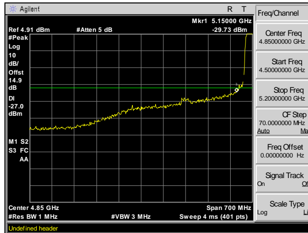
Plot 62. Radiated Band Edge, -27 dBm, Channel 40, 802.11ac 20 MHz
