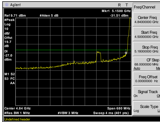
Plot 58. Radiated Band Edge, -27 dBm, Channel 36, 802.11a 20 MHz
