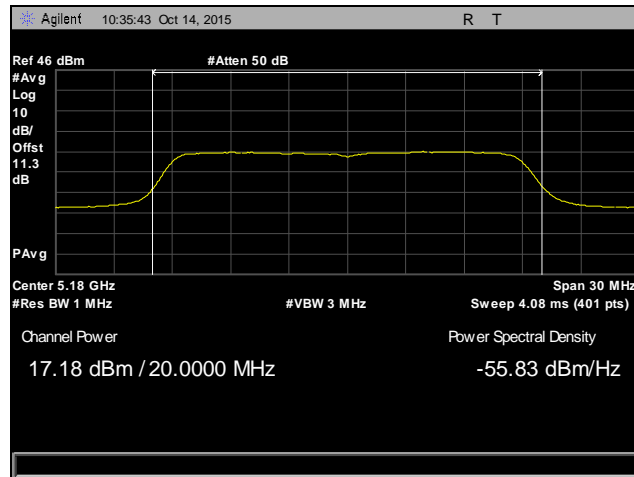
Plot 24. Maximum Conducted Output Power, Channel 36, 802.11n 20 MHz
