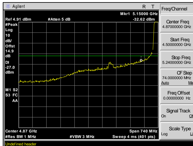
Plot 69. Radiated Band Edge, -27 dBm, Channel 48, 802.11n 20 MHz
