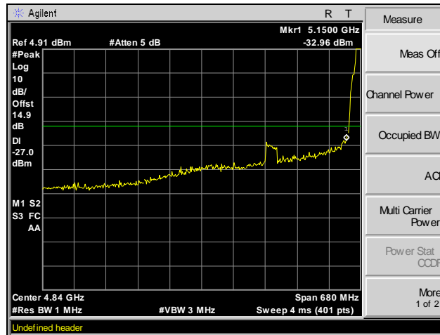
Plot 67. Radiated Band Edge, -27 dBm, Channel 36, 802.11n 20 MHz
