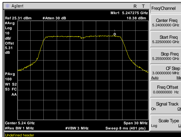
Plot 34. Peak Power Spectral Density, Channel 48, 802.11ac 20 MHz
