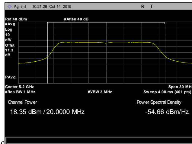
Plot 16. Maximum Conducted Output Power, Channel 40, 802.11a 20 MHz
