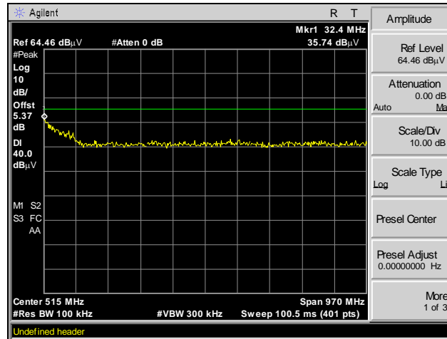
Plot 43. Radiated Spurious Emissions, 30 MHz – 1 GHz, Worst Case Emission
