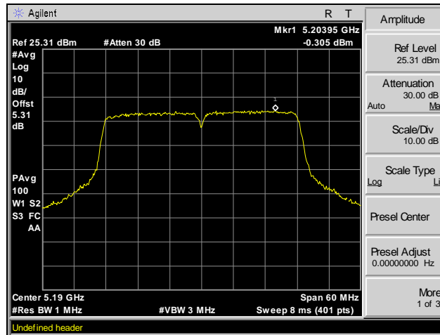
Plot 41. Peak Power Spectral Density, Channel 36, 802.11n 40 MHz
