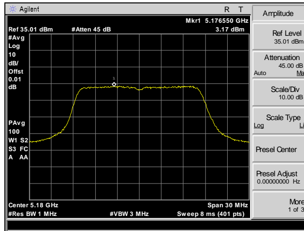
Plot 38. Peak Power Spectral Density, Channel 36, 802.11n 20 MHz
