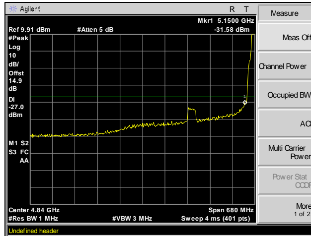
Plot 61. Radiated Band Edge, -27 dBm, Channel 36, 802.11ac 20 MHz
