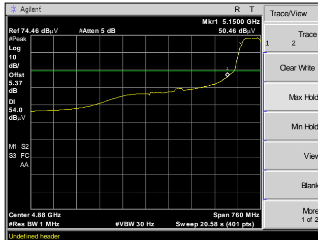
Plot 85. Radiated Band Edge, Average, Channel 44, 802.11n 40 MHz
