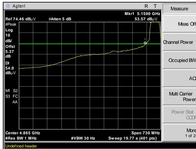
Plot 82. Radiated Band Edge, Average, Channel 40, 802.11n 20 MHz
