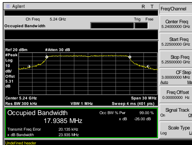
Plot 6. 26 dB Occupied Bandwidth, Channel 48, 802.11ac 20 MHz
