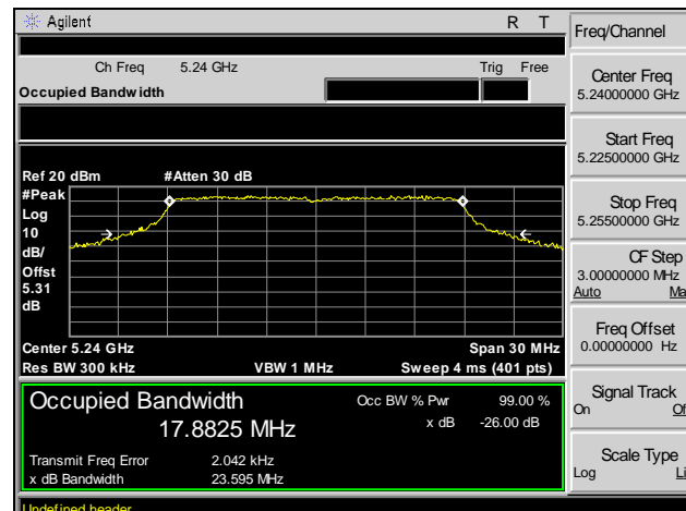
Plot 12. 26 dB Occupied Bandwidth, Channel 48, 802.11n 20 MHz
