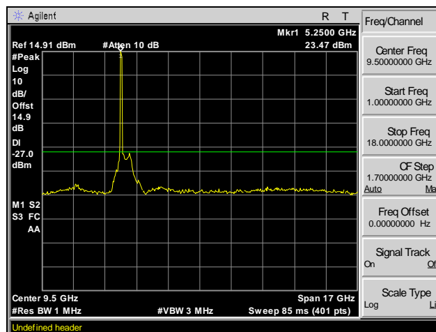
Plot 55. Radiated Spurious Emissions, Above 1 GHz, Channel 48, 802.11n 20 MHz
