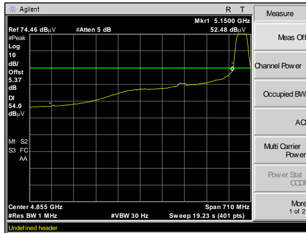
Plot 81. Radiated Band Edge, Average, Channel 36, 802.11n 20 MHz
