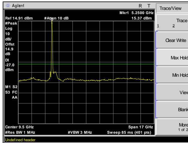
Plot 52. Radiated Spurious Emissions, Above 1 GHz, Channel 36, 802.11ac 80 MHz
