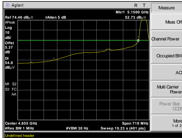
Plot 75. Radiated Band Edge, Average, Channel 36, 802.11ac 20 MHz
