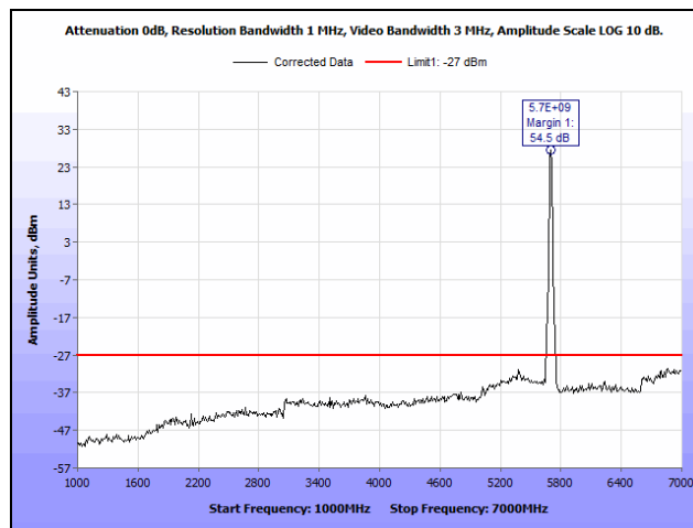
Plot 176. Radiated Spurious Emissions, Channel 140, 802.11n 20 MHz, 1 GHz – 7 GHz
