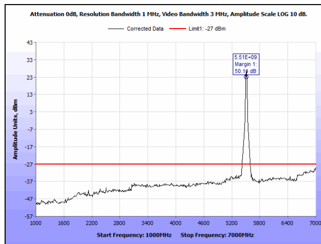
Plot 185. Radiated Spurious Emissions, Channel 100, 802.11n 40 MHz, 1 GHz – 7 GHz
