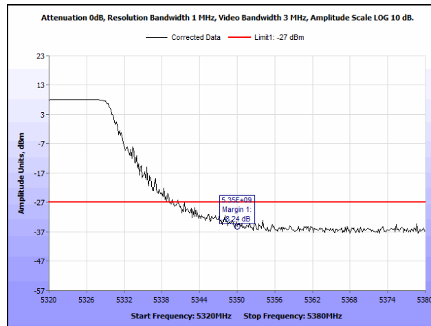
Plot 194. Radiated Band Edge, 802.11a 20 MHz, Channel 64, Peak
