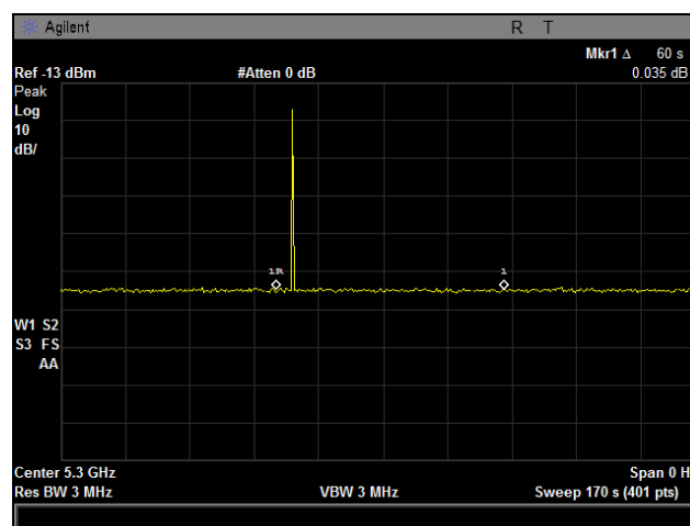
Plot 225. Radar Burst at the Beginning of CACT
