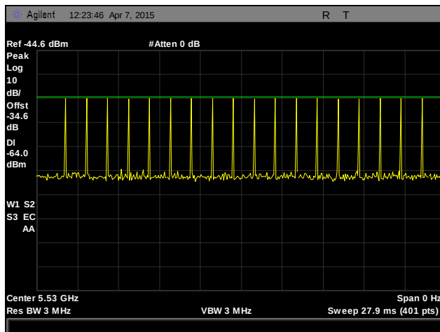
Plot 217. Radar Type 0 Calibration
