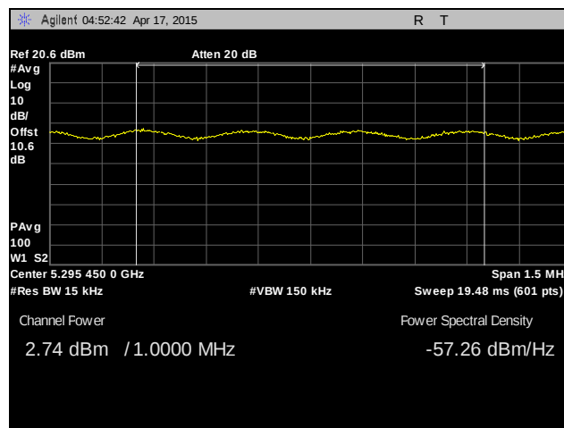
Plot 66. Peak Power Spectral Density, Channel 60, 802.11a 20 MHz, 5300 MHz
