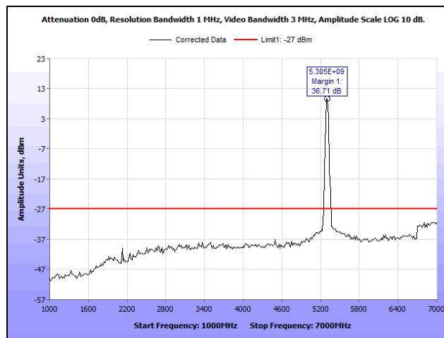
Plot 119. Radiated Spurious Emissions, Channel 60, 802.11ac 20 MHz, 1 GHz – 7 GHz
