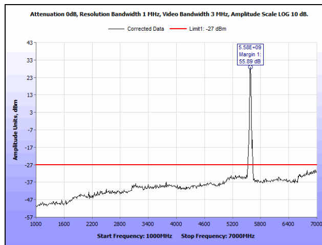
Plot 110. Radiated Spurious Emissions, Channel 116, 802.11a 20 MHz, 1 GHz – 7 GHz
