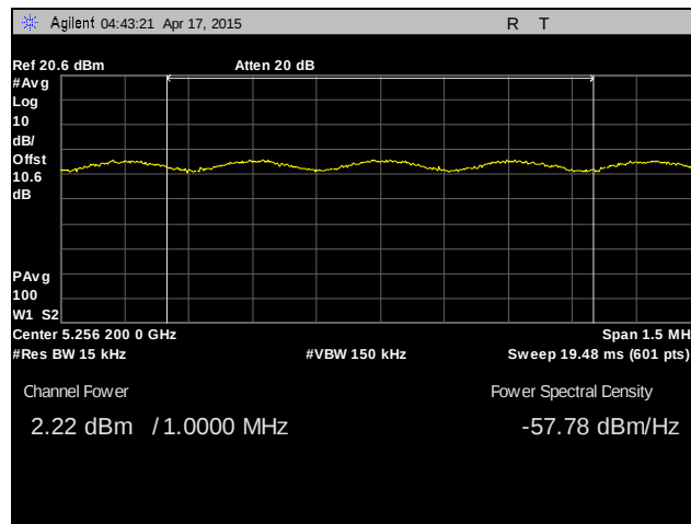
Plot 65. Peak Power Spectral Density, Channel 52, 802.11a 20 MHz, 5260 MHz
