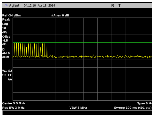
Plot 218. Radar Type 1 Calibration
