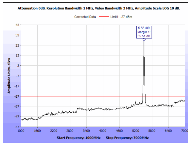
Plot 107. Radiated Spurious Emissions, Channel 100, 802.11a 20 MHz, 1 GHz – 7 GHz
