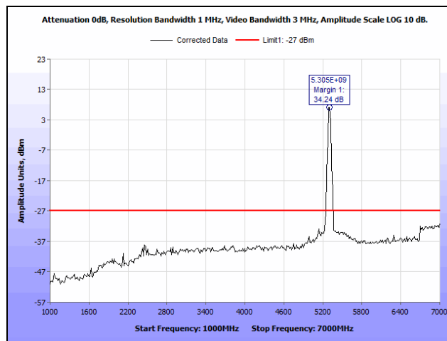
Plot 101. Radiated Spurious Emissions, Channel 60, 802.11a 20 MHz, 1 GHz – 7 GHz
