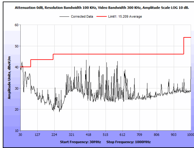
Plot 160. Radiated Spurious Emissions, Channel 52, 802.11n 20 MHz, 30 MHz – 1 GHz
