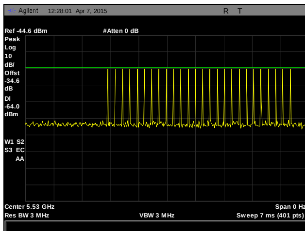
Plot 219. Radar Type 2 Calibration
