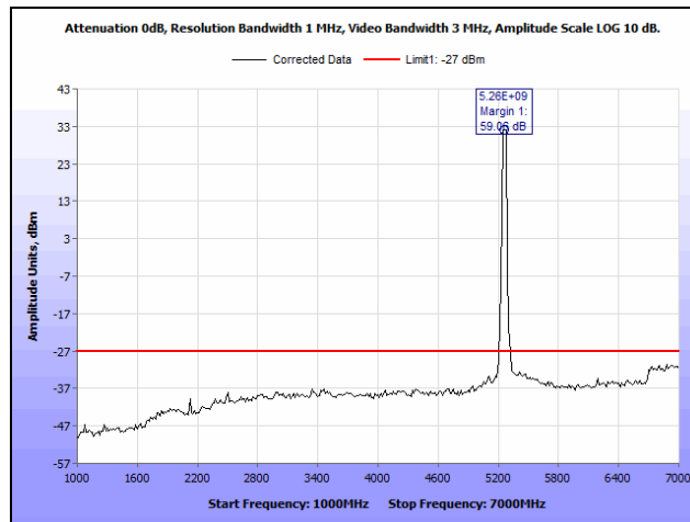
Plot 116. Radiated Spurious Emissions, Channel 52, 802.11ac 20 MHz, 1 GHz – 7 GHz
