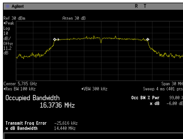
Plot 55. 6 dB Occupied Bandwidth, Mid Channel, 802.11a
