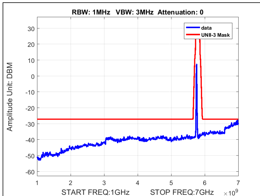
Plot 30. Radiated Spurious Emissions, Low Channel, 802.11a, 1 GHz – 7 GHz
