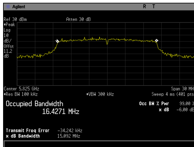
Plot 56. 6 dB Occupied Bandwidth, High Channel, 802.11a
