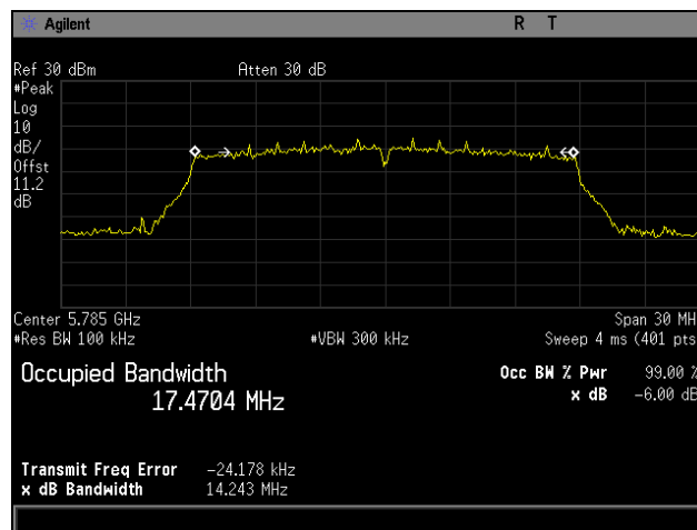
Plot 58. 6 dB Occupied Bandwidth, Mid Channel, 802.11ac 20 MHz
