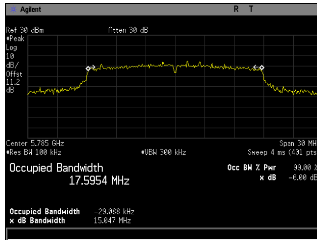
Plot 64. 6 dB Occupied Bandwidth, Mid Channel, 802.11n 20 MHz
