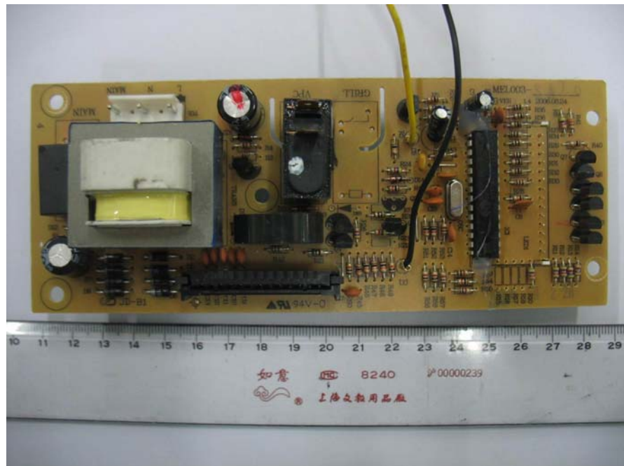
PCB View
