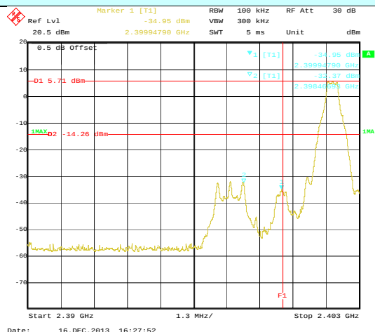
No-hopping mode
