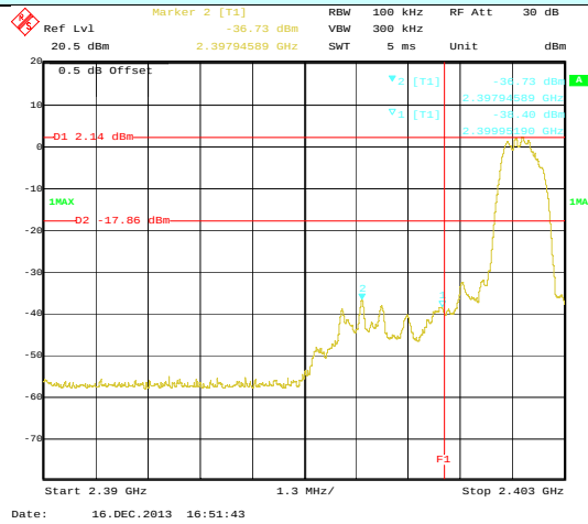
No-hopping mode
