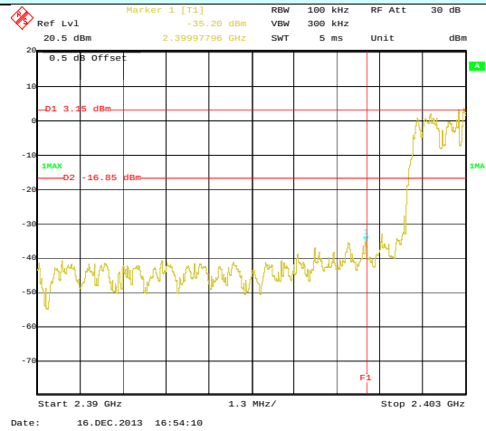
Hopping mode
