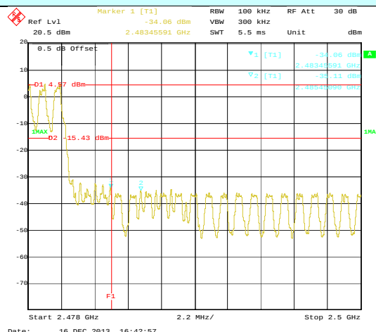
Hopping mode
