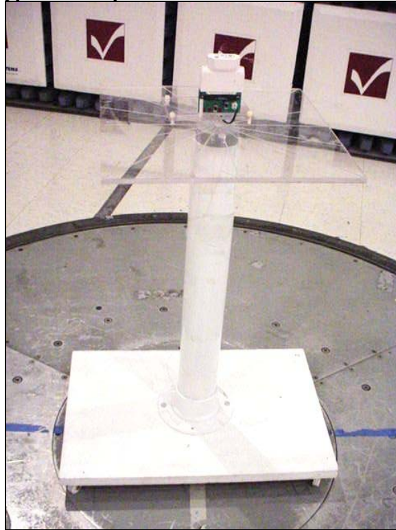
Typical EUT placement on the Test Pedestal
