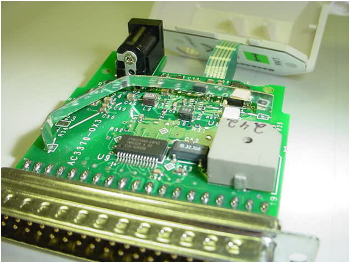
Photo Four – Internal Wall Unit - Wire Band Antenna
