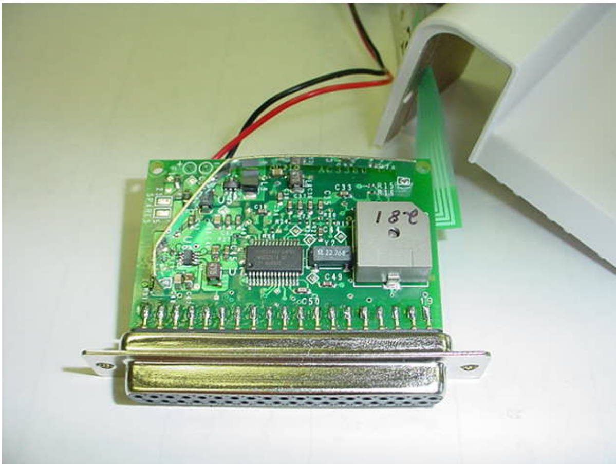
Photo Seven – Internal Bed Unit – Non-RF Component Side w/Antenna
