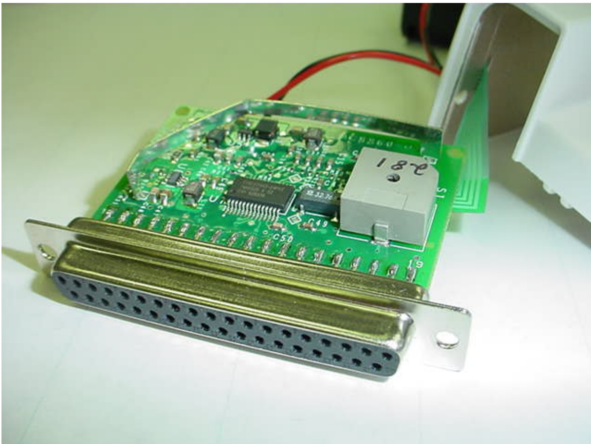
Photo Eight – Internal Bed Unit – Close-up of Wire Band Antenna
