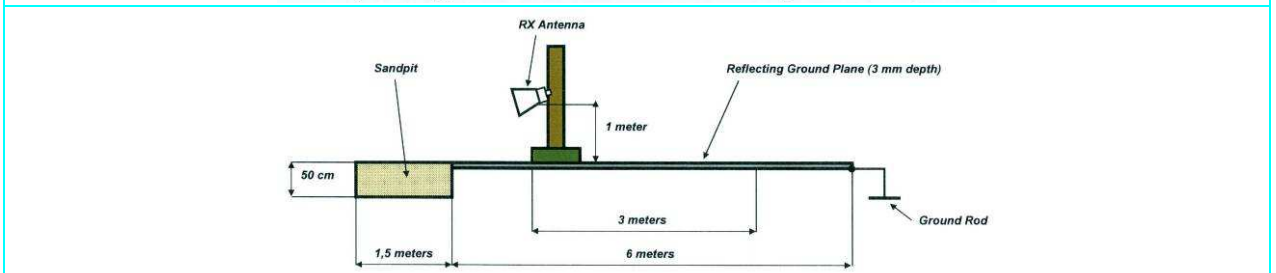
Radiated measurement above 960 MHz
