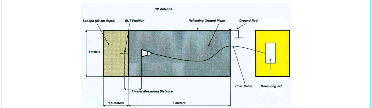
Radiated measurement below 960 MHz
