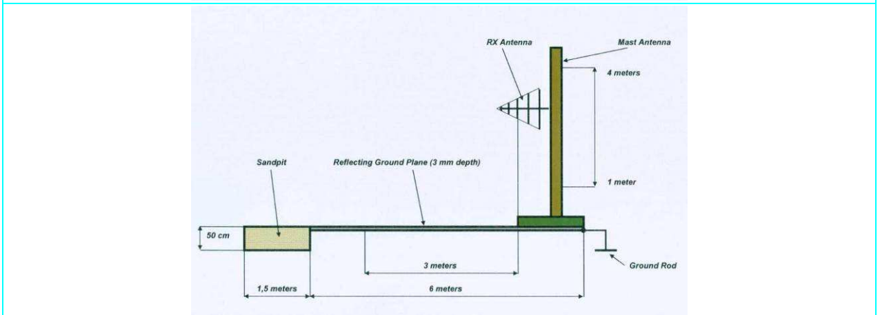
Radiated measurement below 960 MHz
