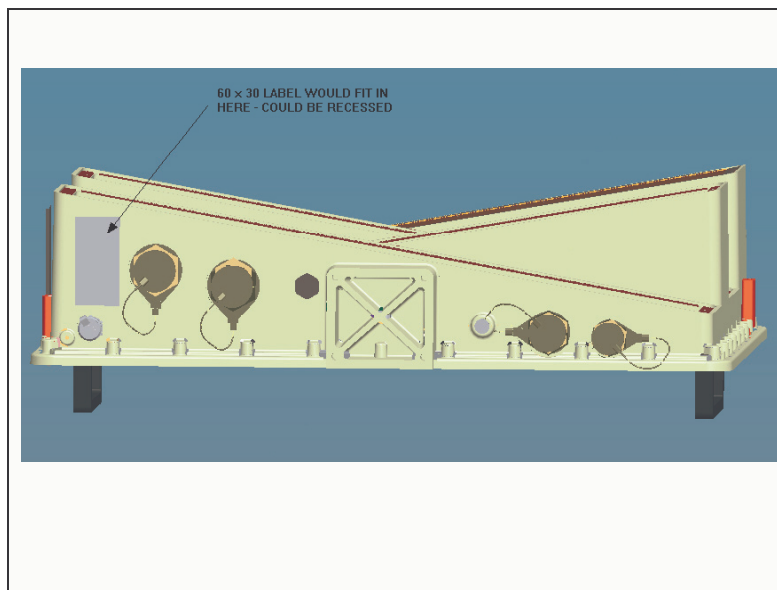
Figure 2 : Location of Label
