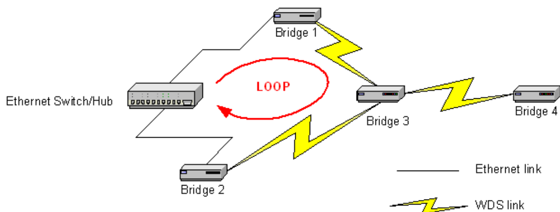
Fig. 351. Network topology containing a loop.
