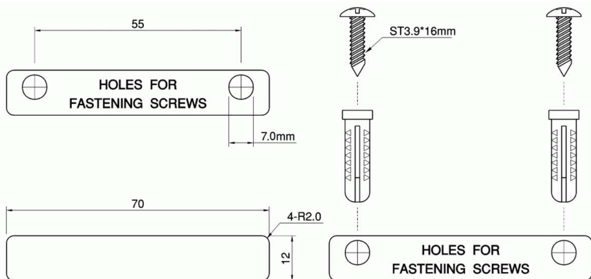
Fig. 1. Mounting the DDC36g on a wall.
