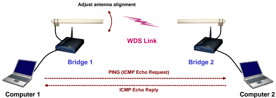
Fig. 362. Adjusting alignments of external directional antennas.
