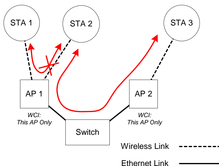
Fig. 384. Behavior of the “This AP Only” wireless client isolation option.
