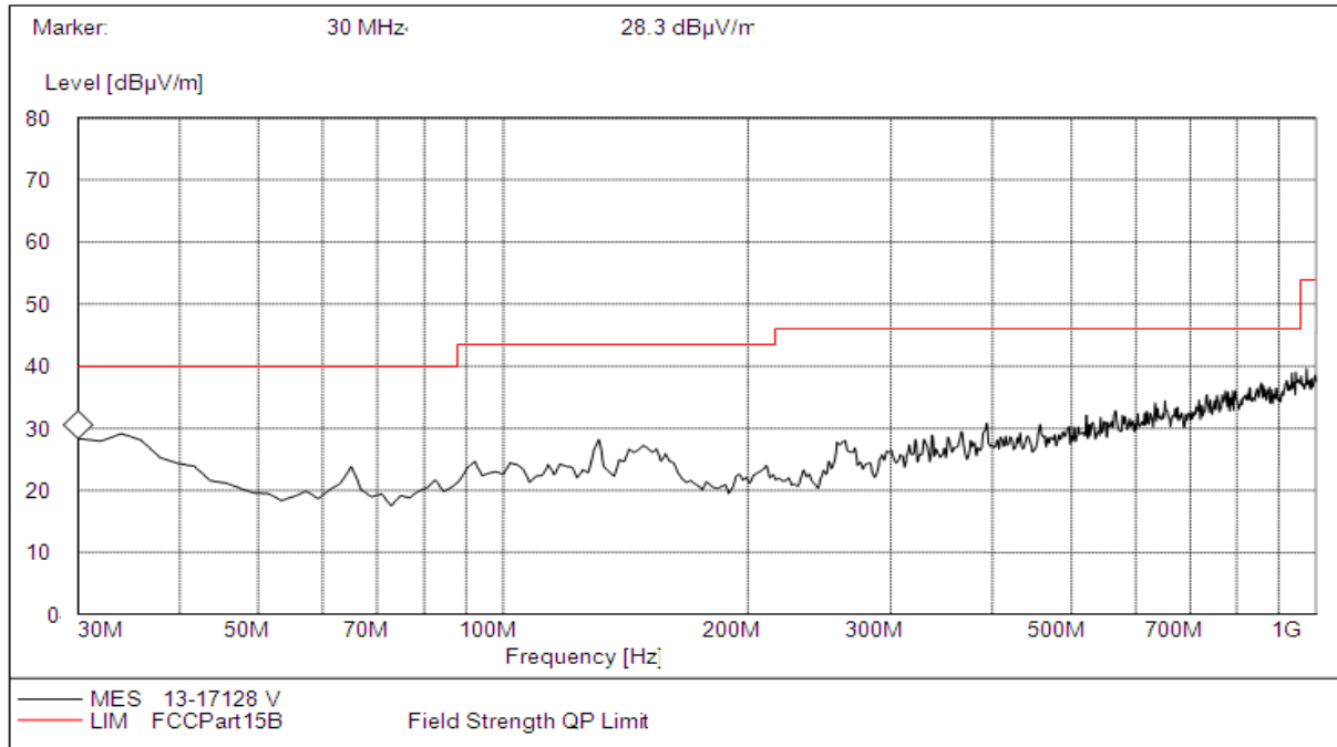
(Plot B: 30MHz to 1GHz, Antenna Vertical)
