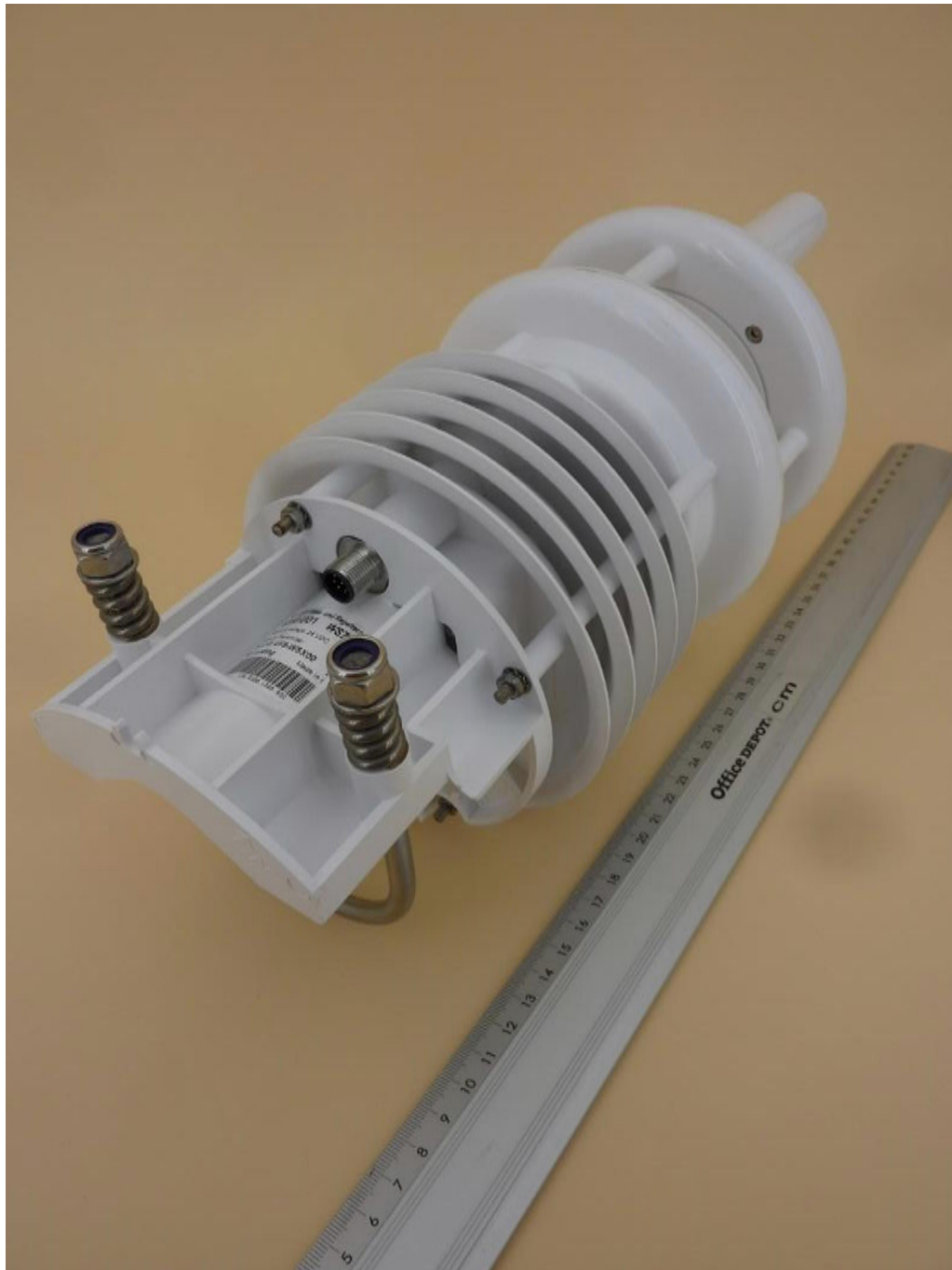
WS700-UMB, 3-D-view 2
