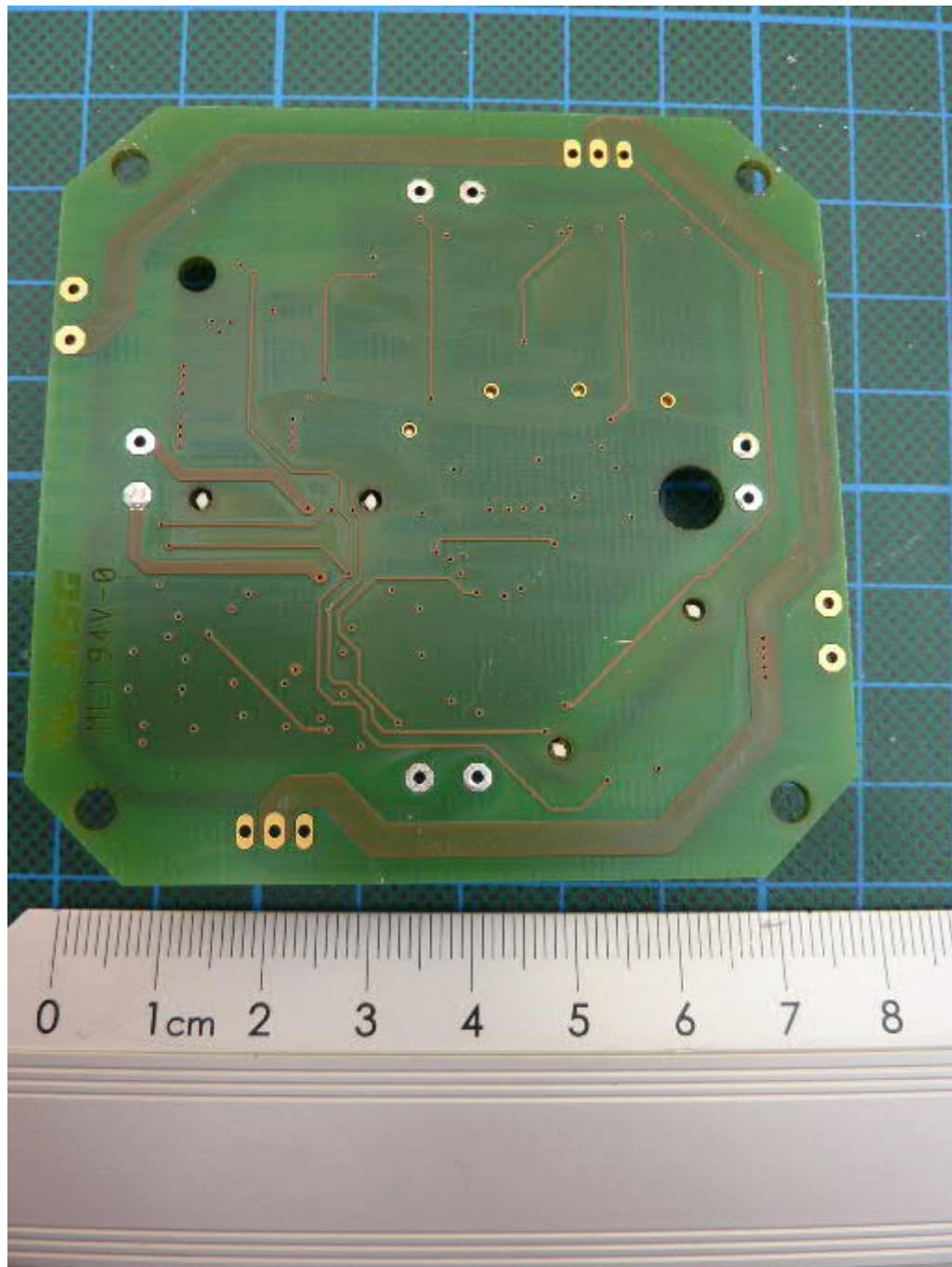
WS700-UMB, ultra sonic PCB, bottom view
