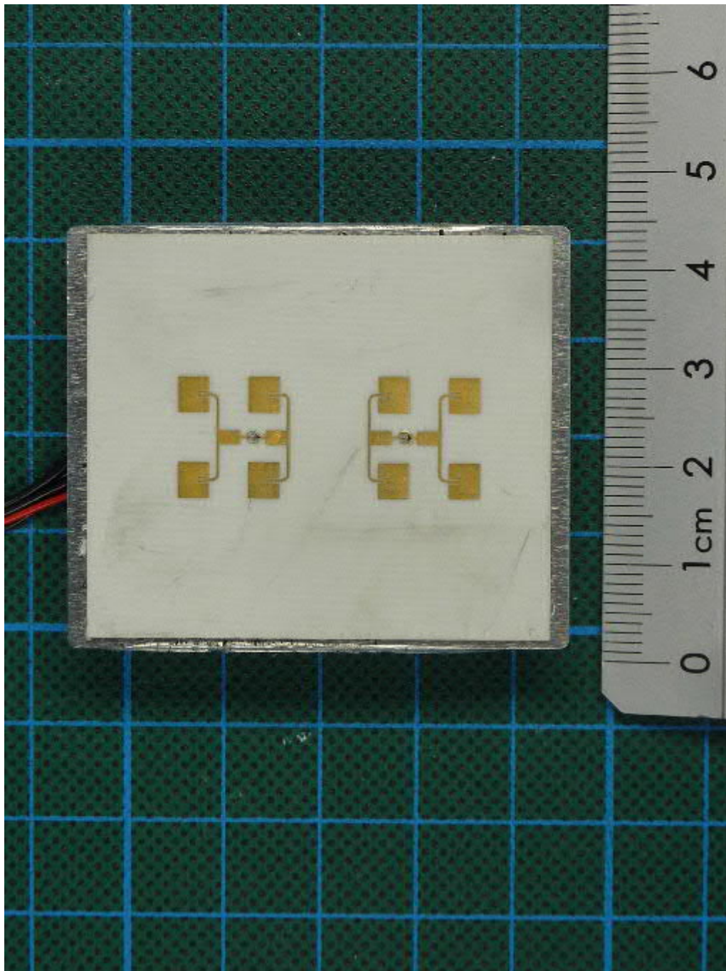
WS700-UMB, radar module, top view
