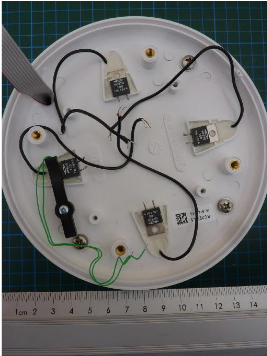
WS700-UMB, housing, ultra sonic PCB removed
