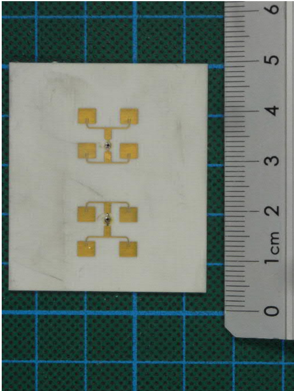
WS700-UMB, radar module, antenna PCB, top view
