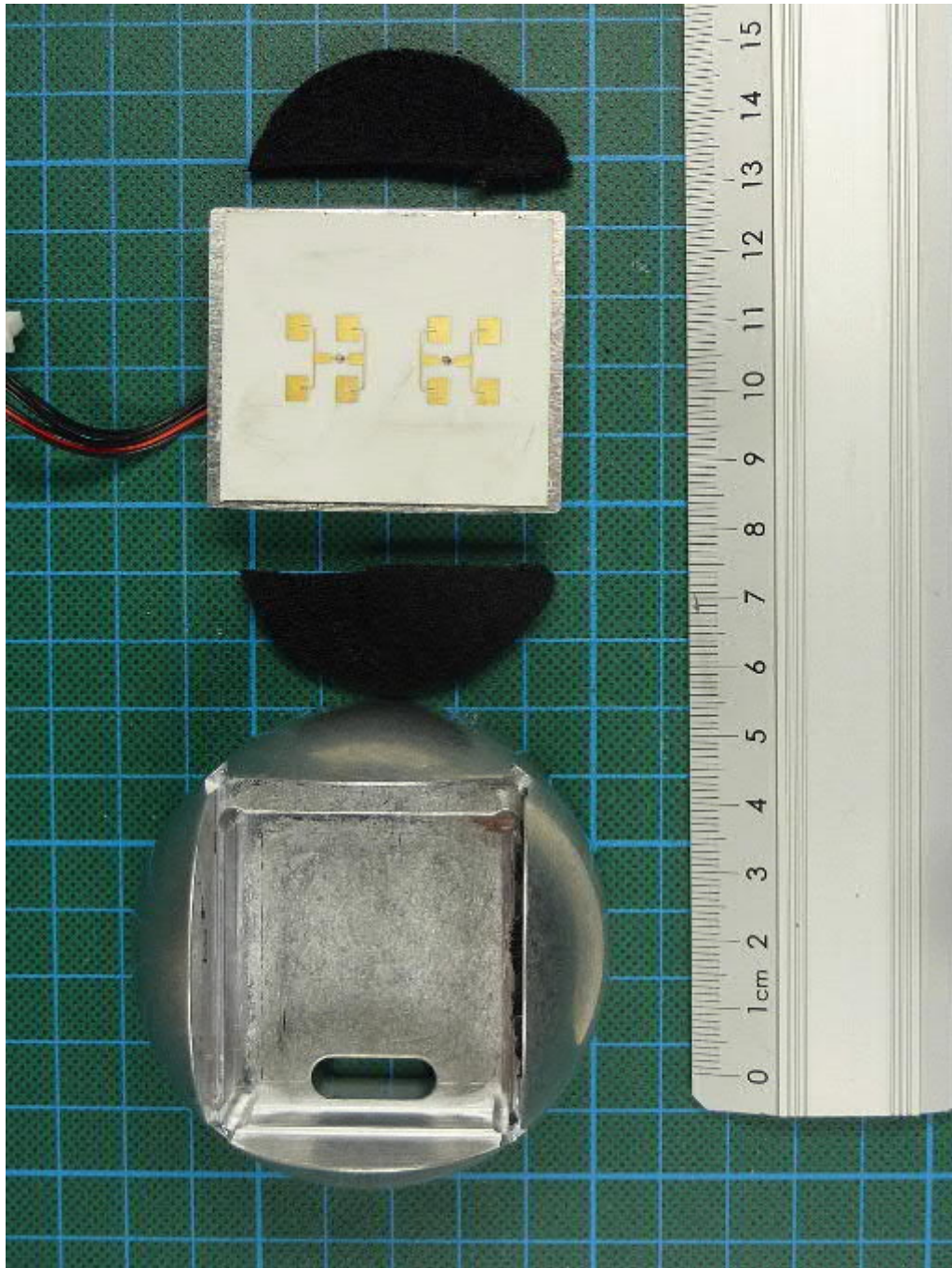
WS700-UMB, radar modul carrier, module removed
