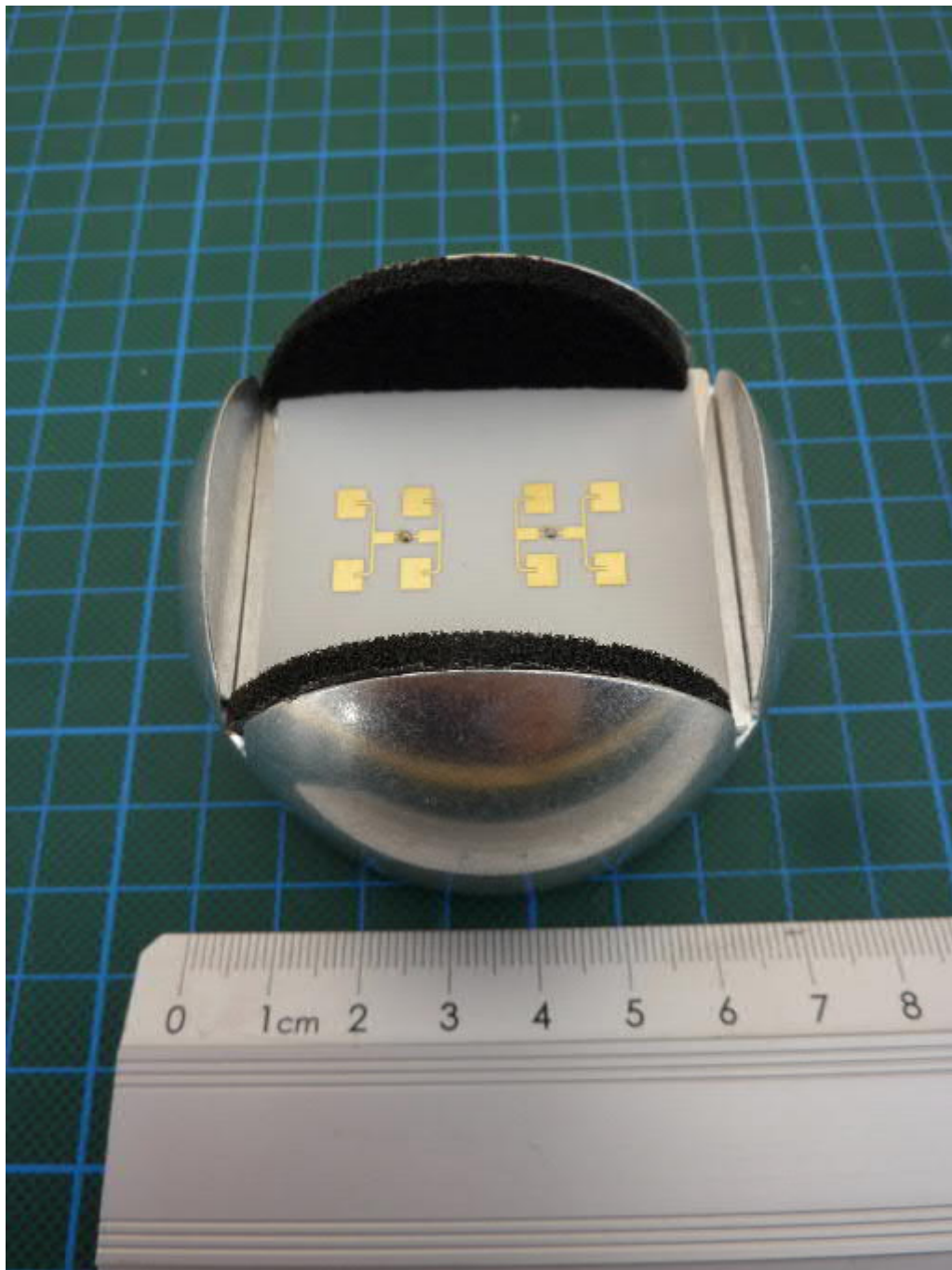
WS700-UMB, radar modul carrier, total view
