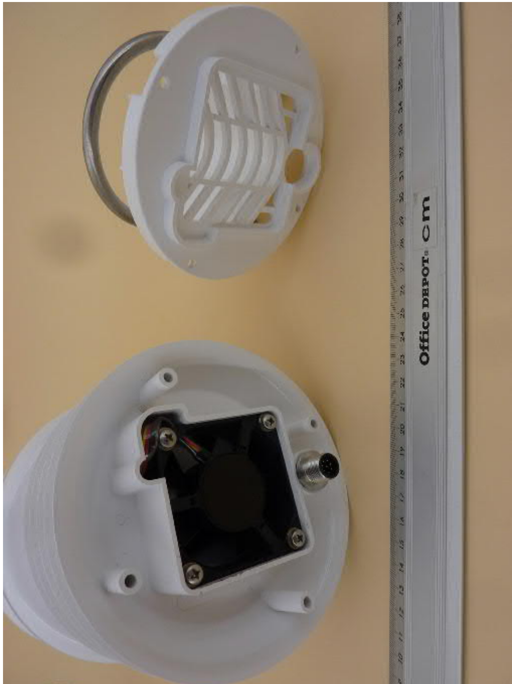
WS700-UMB, internal view 1
