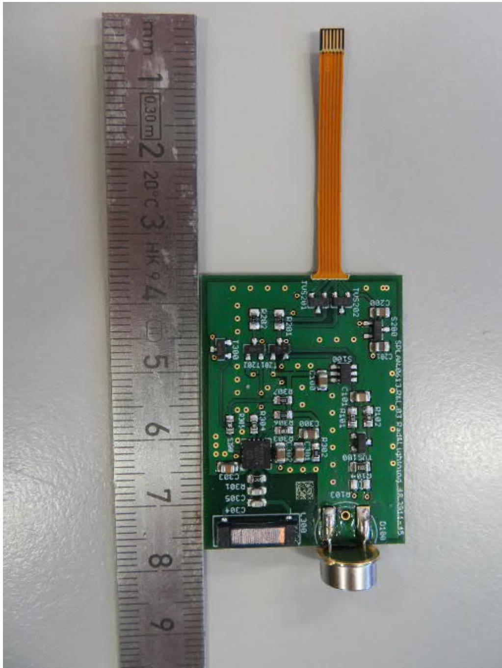
WS700-UMB, lightning sensor PCB, top view (supplied by the applicant)
