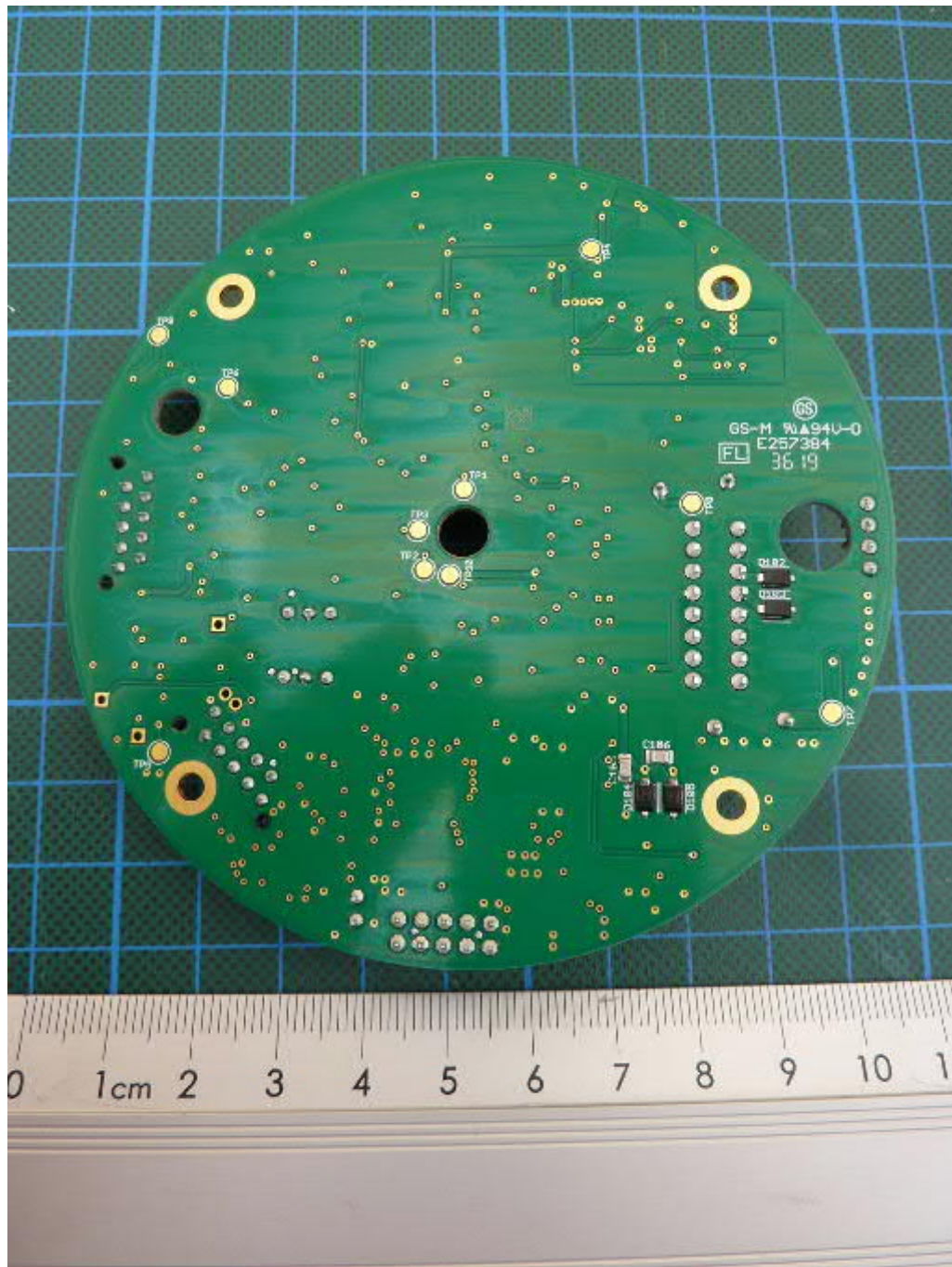
WS700-UMB, main PCB, bottom view
