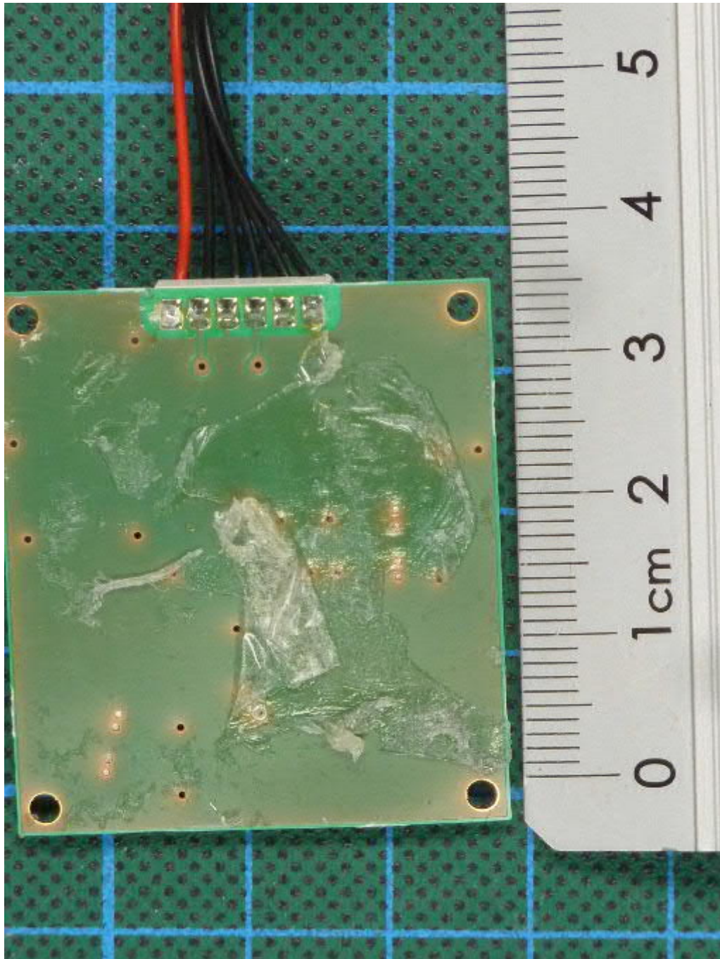
WS700-UMB, radar module, PCB, bottom view
