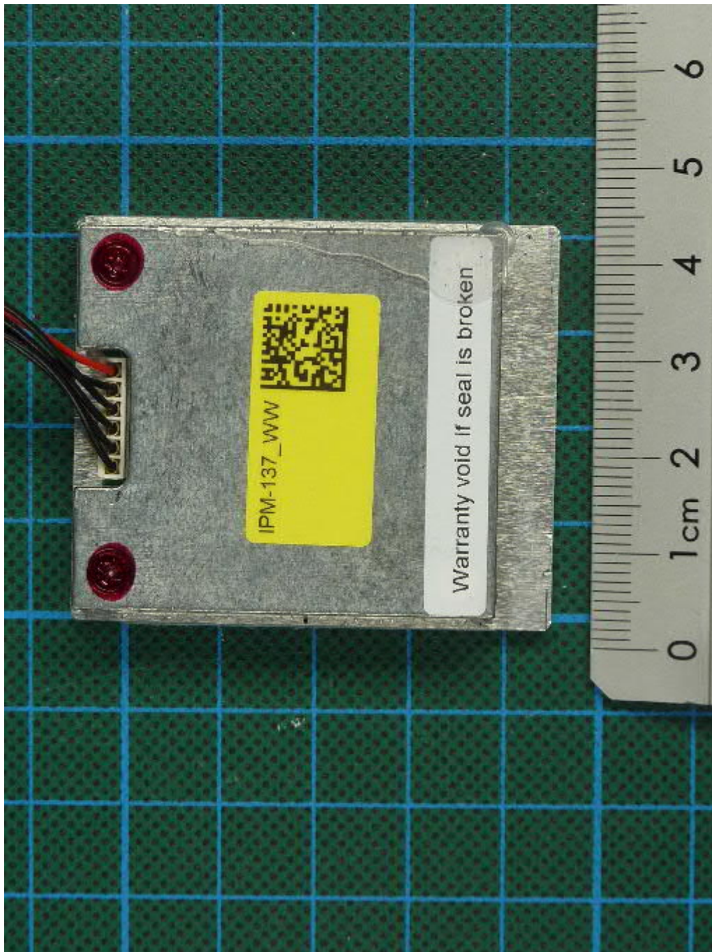
WS700-UMB, radar module, bottom view
