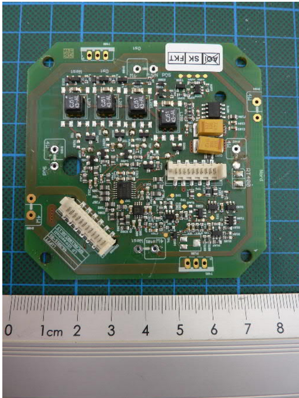
WS700-UMB, ultra sonic PCB, top view
