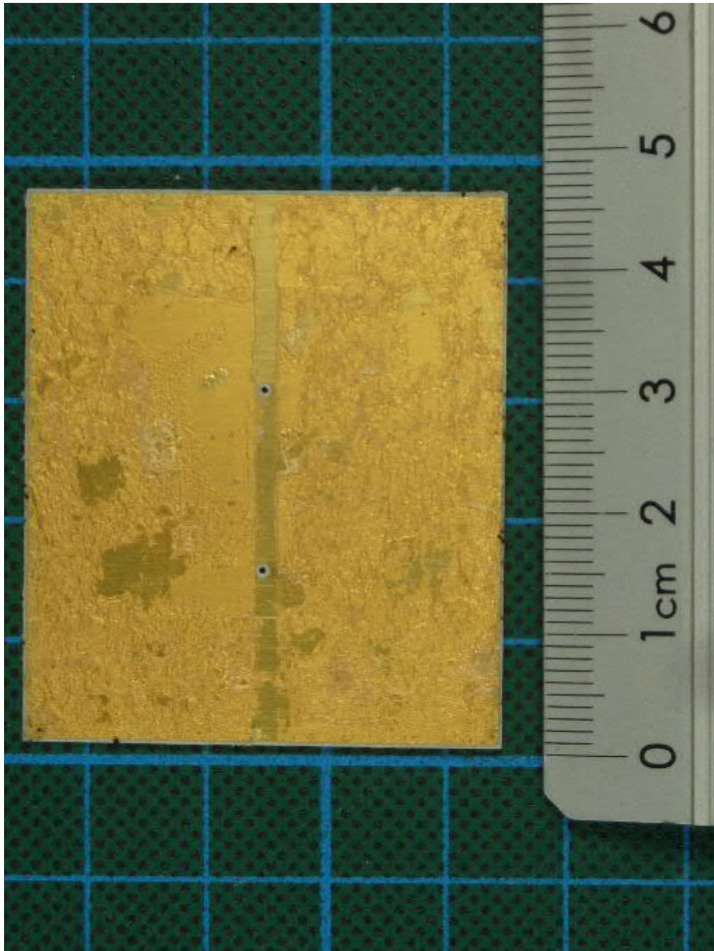
WS700-UMB, radar module, antenna PCB, bottom view
