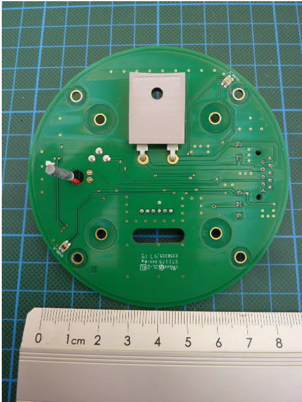
WS700-UMB, radar carrier PCB, bottom view
