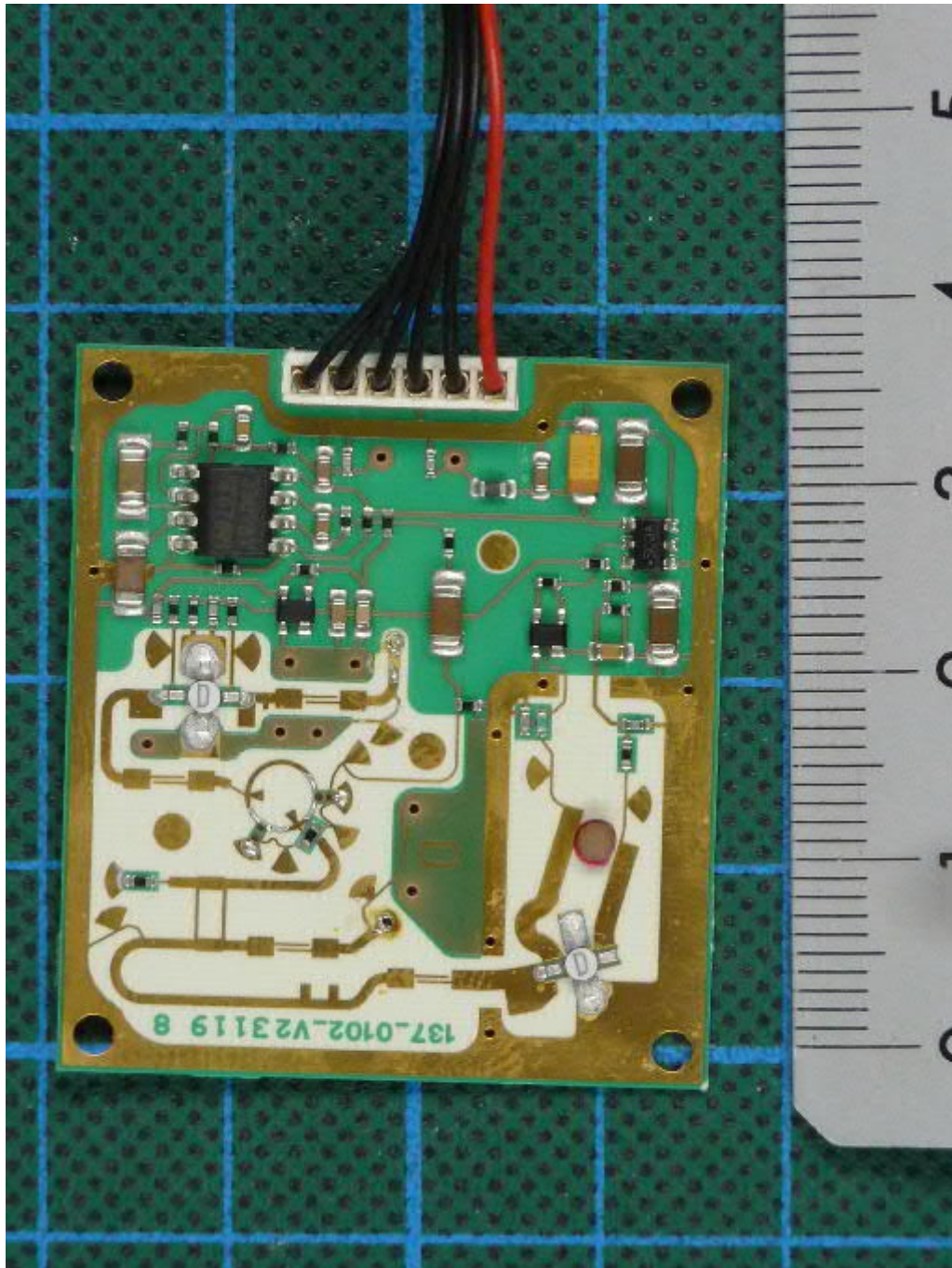
WS700-UMB, radar module, PCB, top view
