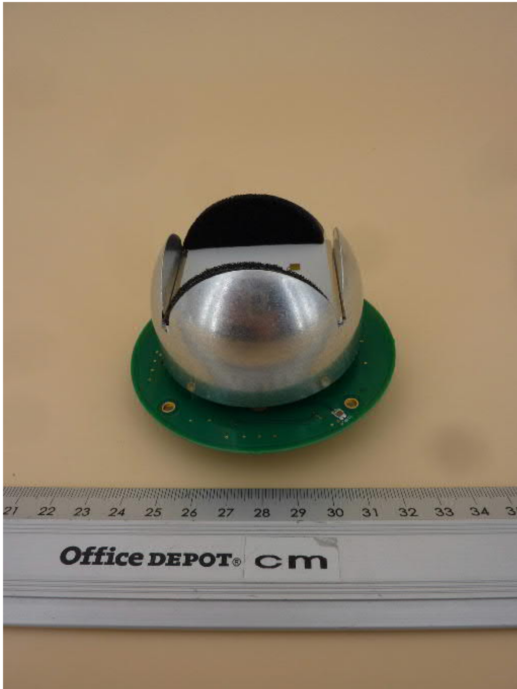
WS700-UMB, radar part, total view
