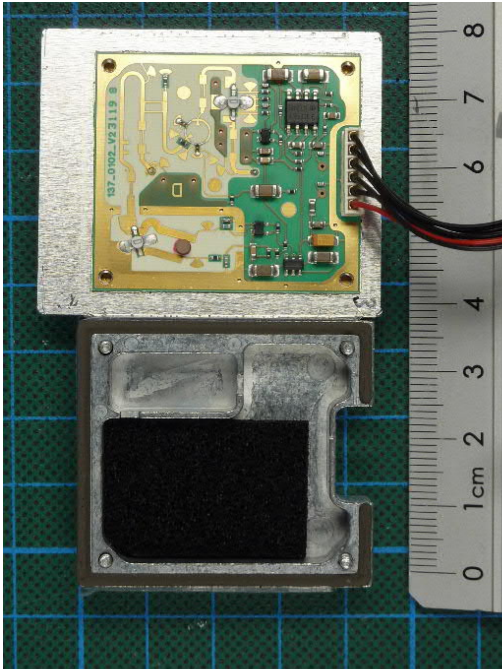
WS700-UMB, radar module, internal view
