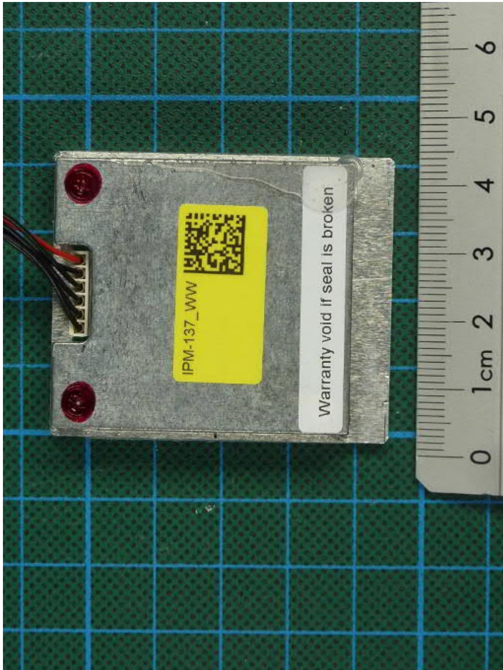
WS400-UMB, radar module, bottom view
