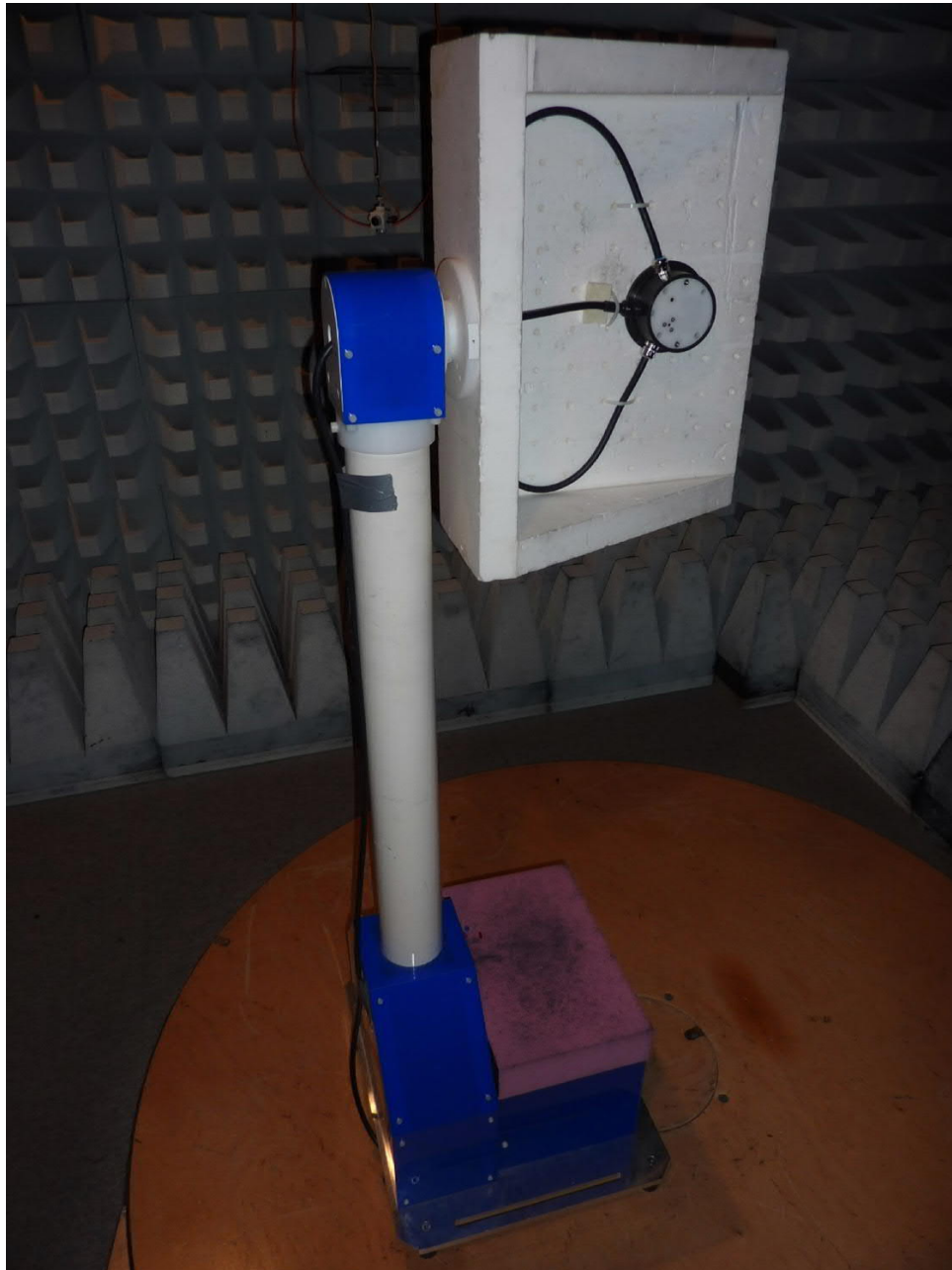
IRS31Pro-UMB, test setup fully anechoic chamber
