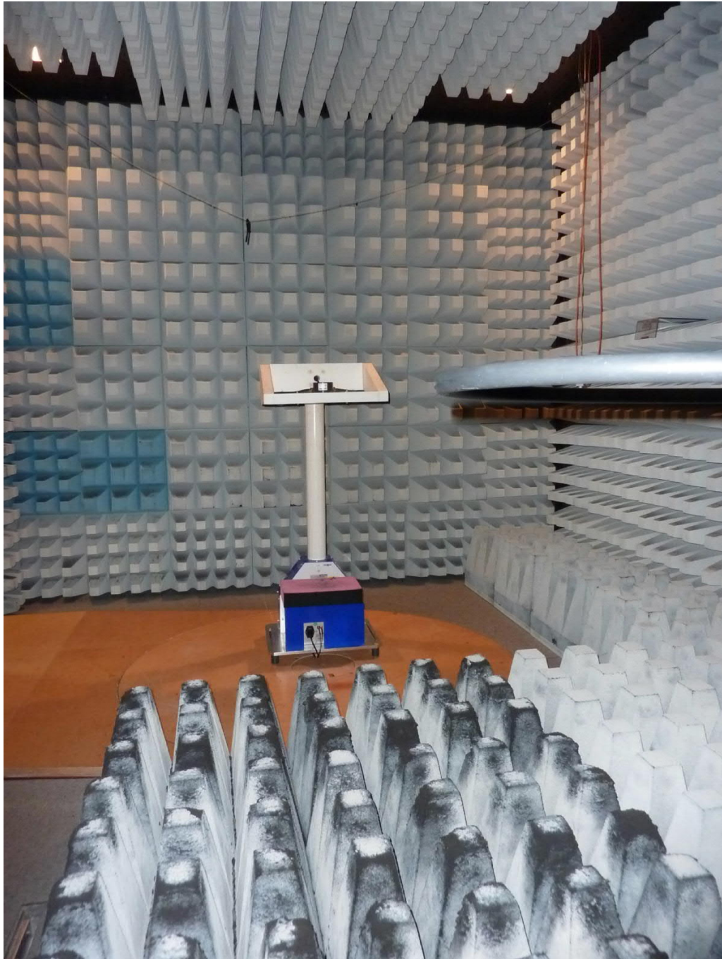
IRS31Pro-UMB, test setup fully anechoic chamber
