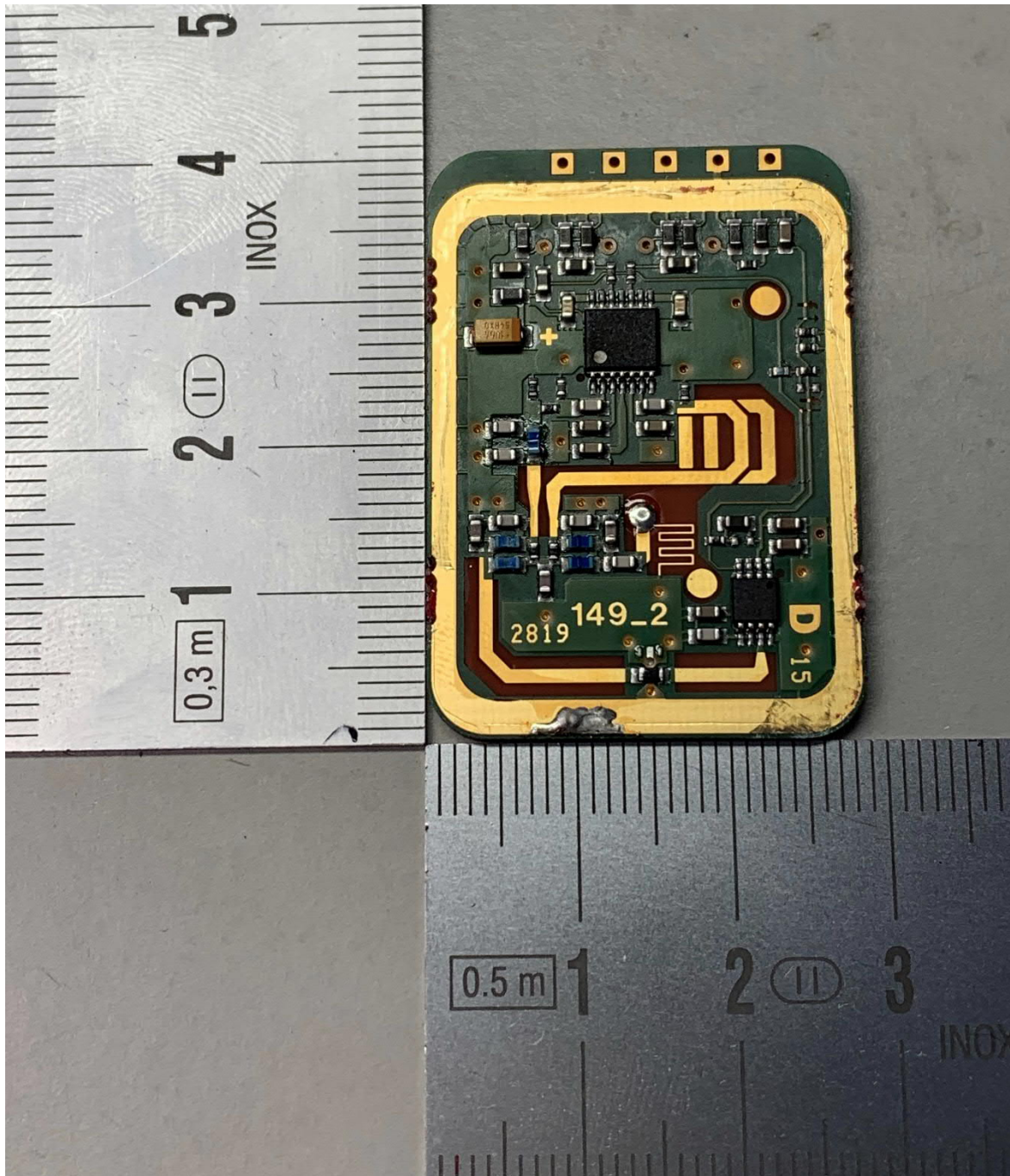
IRS31Pro-UMB, field disturbance sensor, top view (supplied by the applicant)
