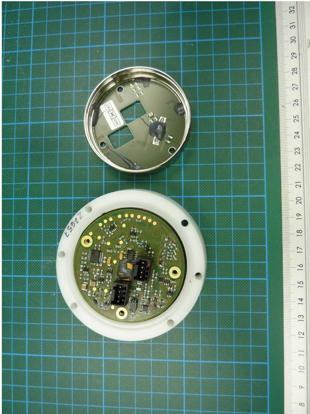
IRS31Pro-UMB, PCB, top view (shielding removed)
