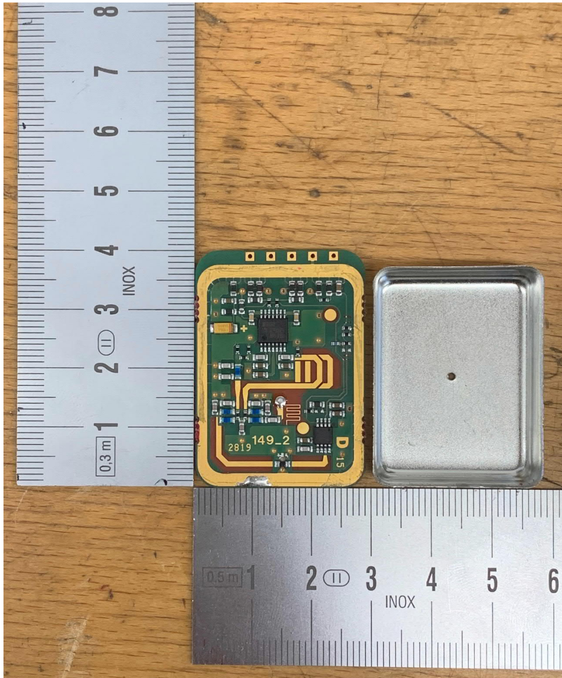
IRS31Pro-UMB, field disturbance sensor, top view, shielding removed (supplied by the applicant)
