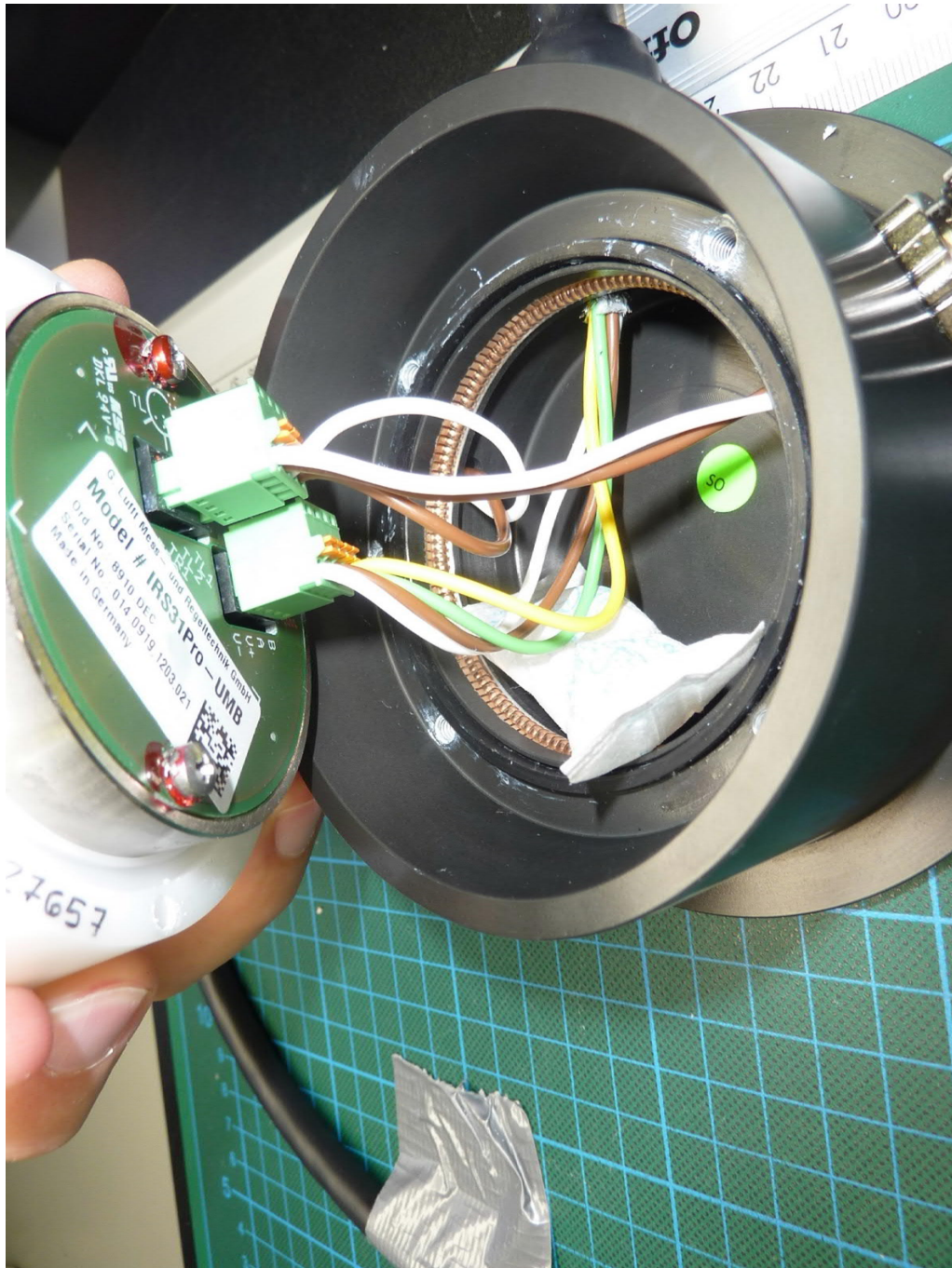
IRS31Pro-UMB, internal view, (housing opened)
