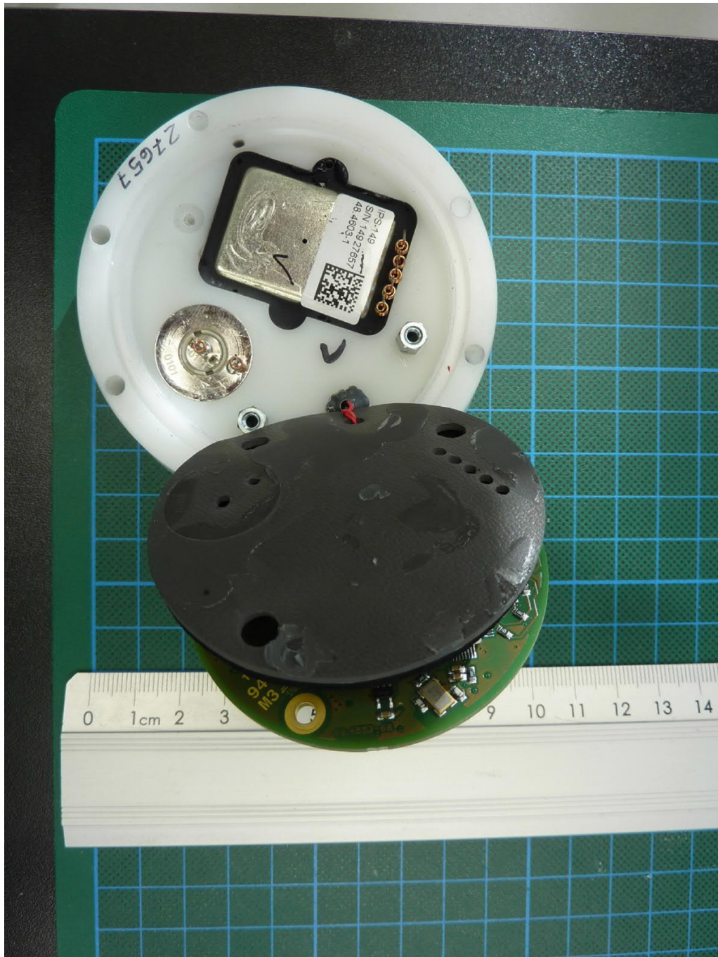
IRS31Pro-UMB, internal view, detail view to field disturbance sensor
