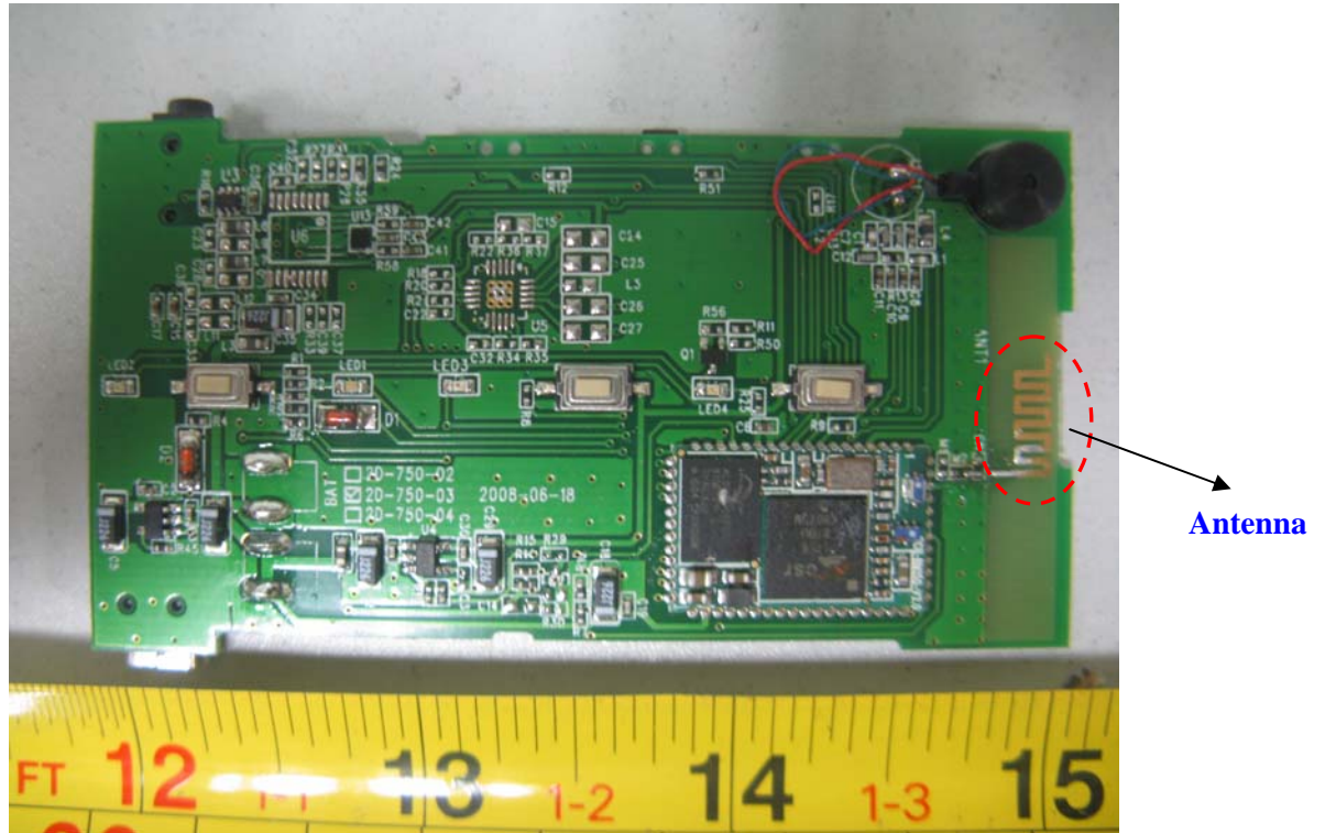
EUT- Main Board Components Bottom View
