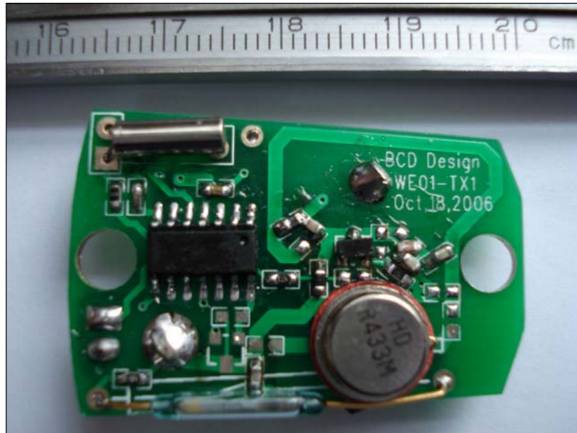
Photo 5- Main Board Front View of SENSOR(Transmitter)
