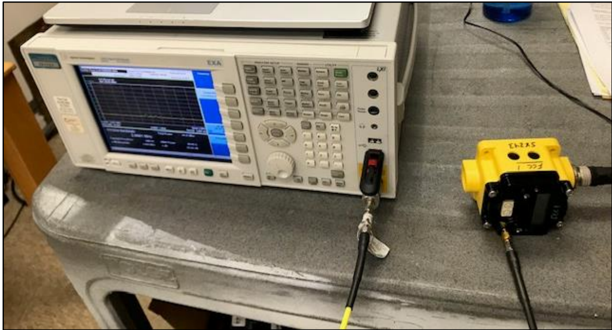
Photograph 3: Conducted Emissions Test Setup
