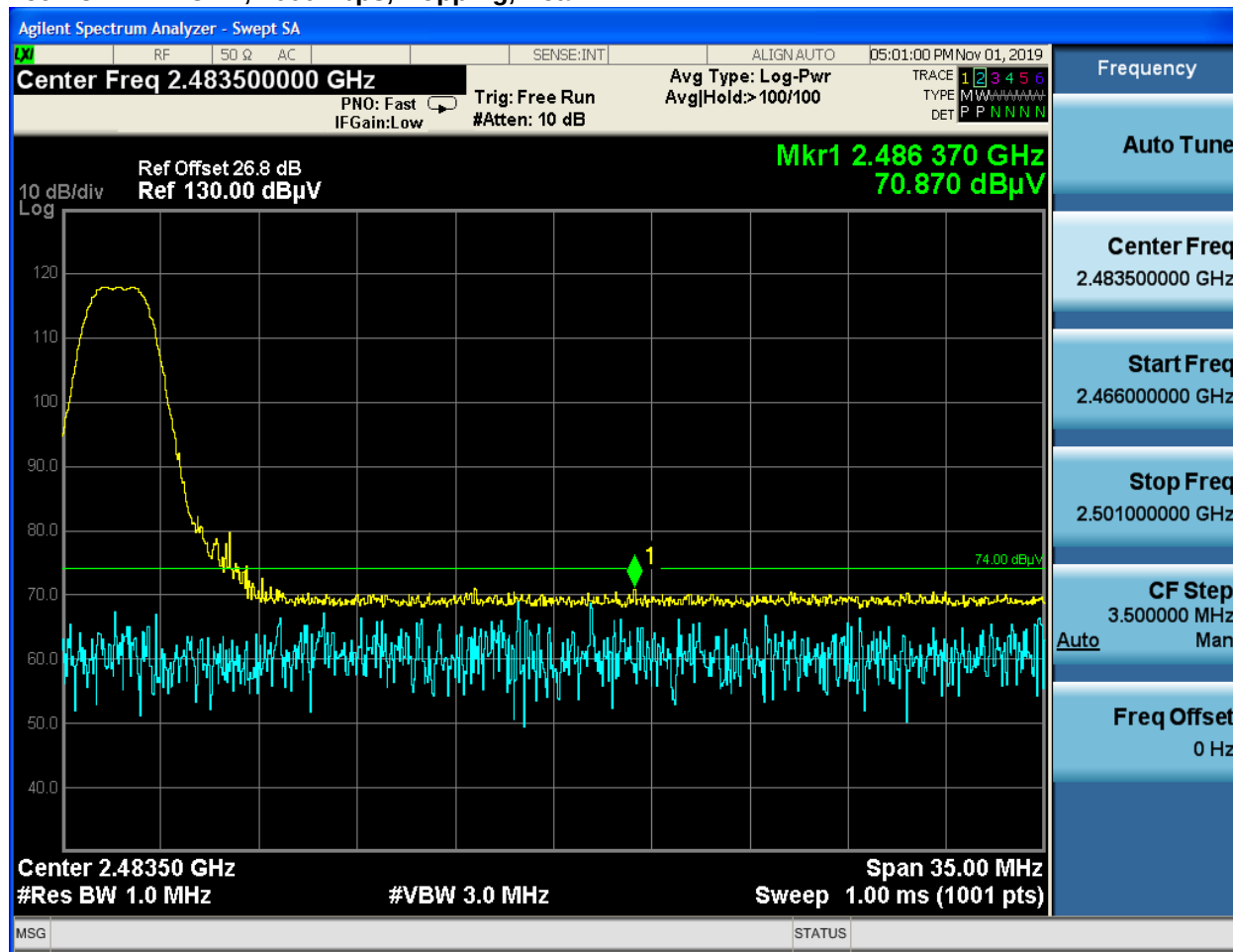
Plot 4-8: UBE, 1000 kbps, Hopping, Peak
