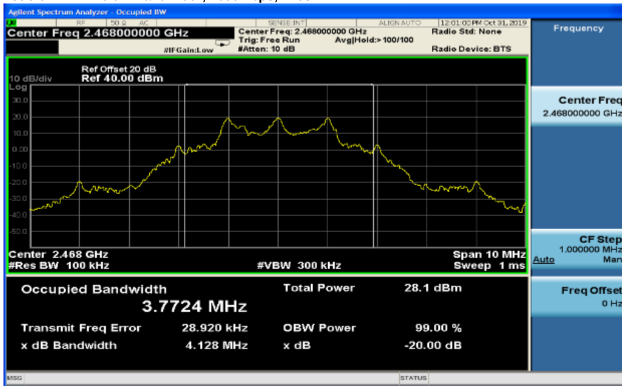
Plot 6-9: 20 dB Bandwidth, 2000 kbps, 2468 MHz
