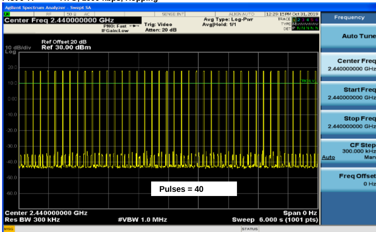
Plot 9-7: ATO, 1000 kbps, Hopping
