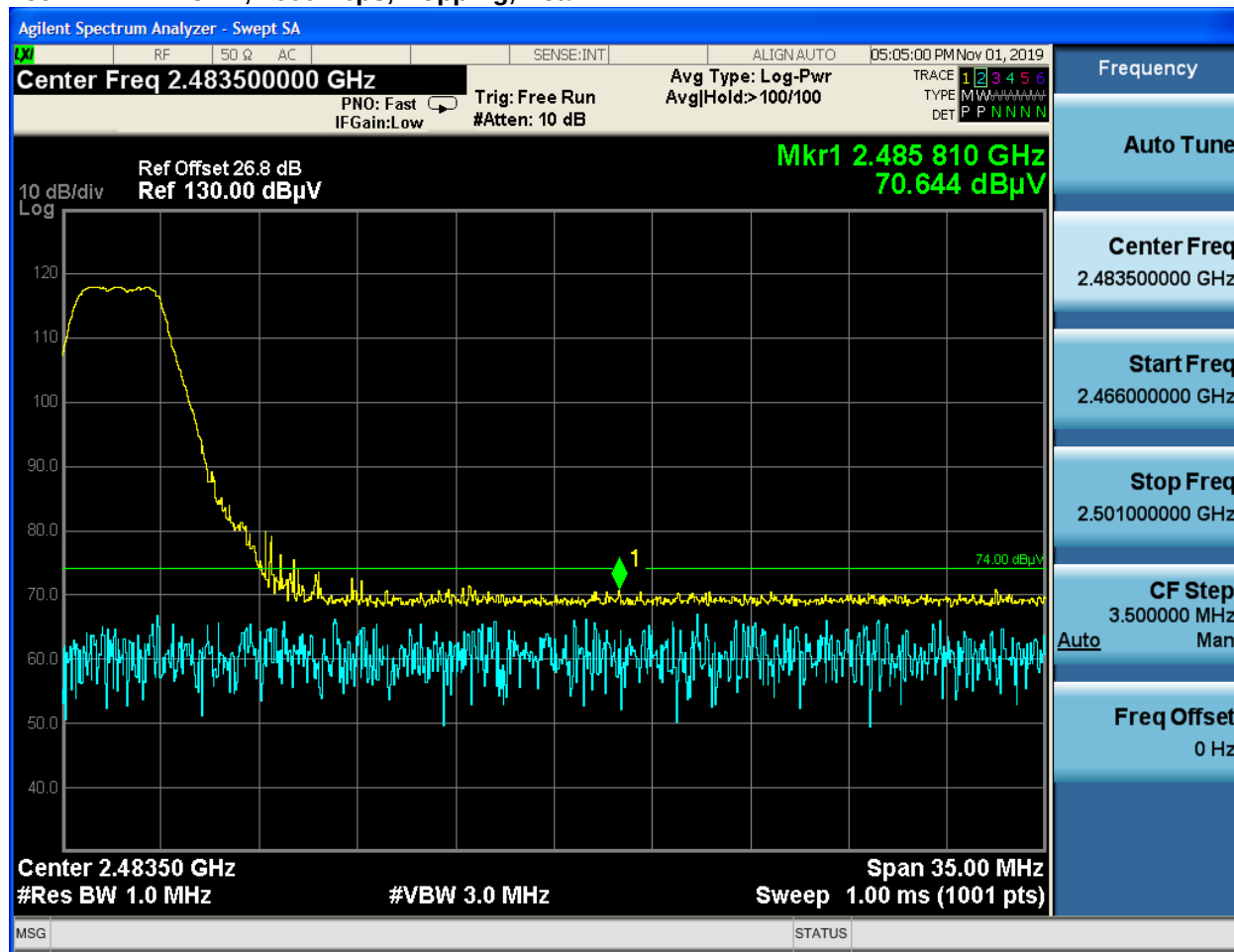
Plot 4-12: UBE, 2000 kbps, Hopping, Peak
