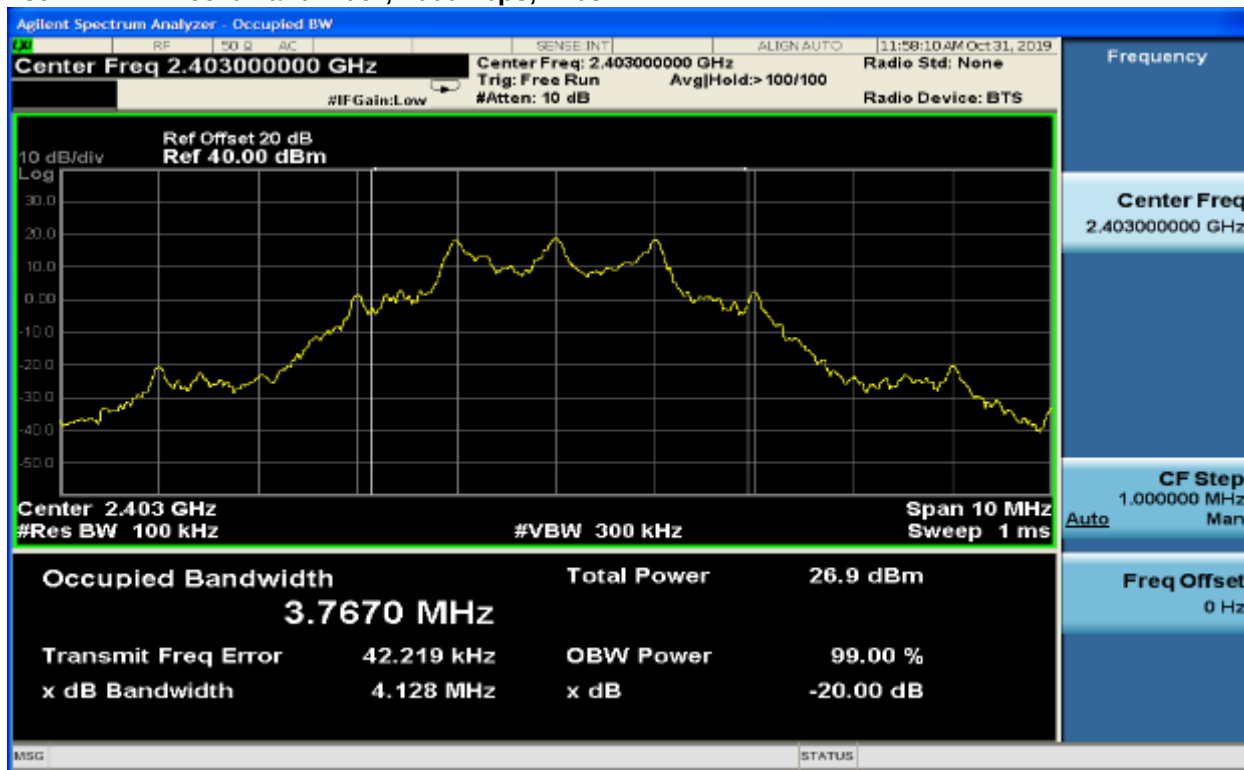
Plot 7-7: 99% Bandwidth, 2000 kbps, 2403 MHz
