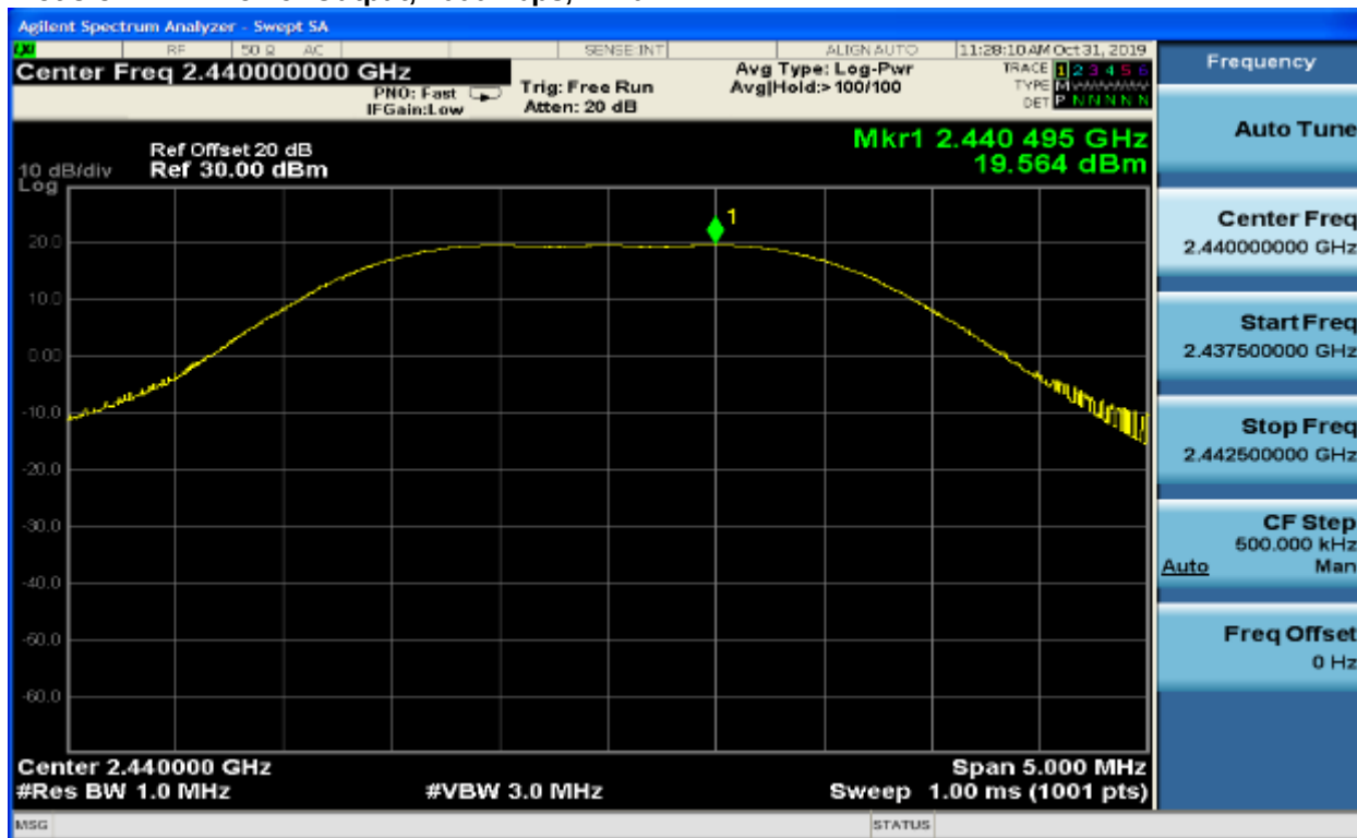
Plot 3-5: Power Output, 1000 kbps, 2440 MHz
