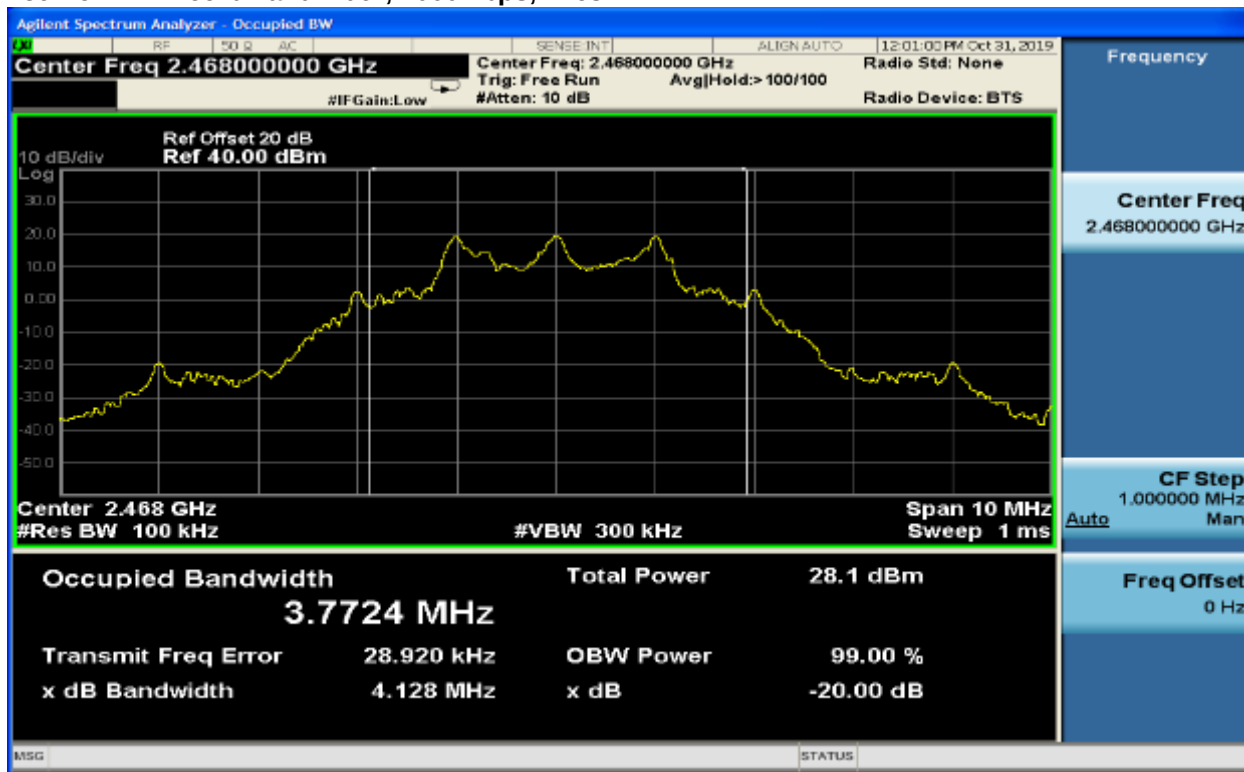
Plot 7-9: 99% Bandwidth, 2000 kbps, 2468 MHz
