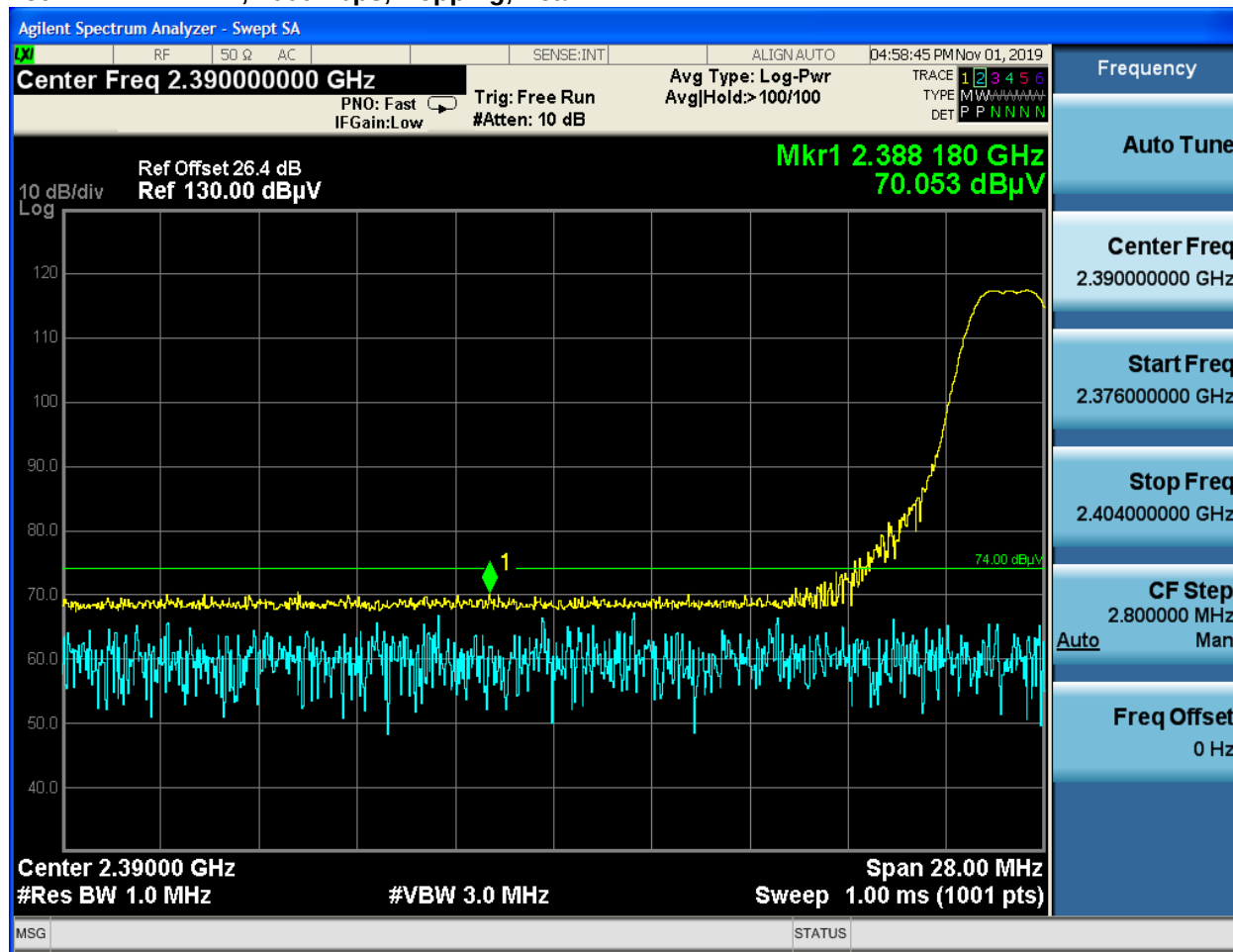
Plot 4-7: LBE, 1000 kbps, Hopping, Peak
