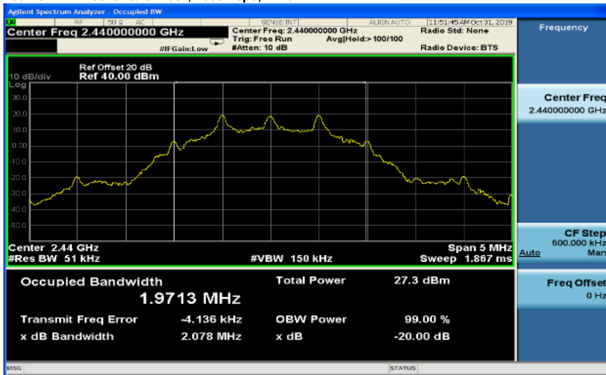
Plot 7-5: 99% Bandwidth, 1000 kbps, 2440 MHz
