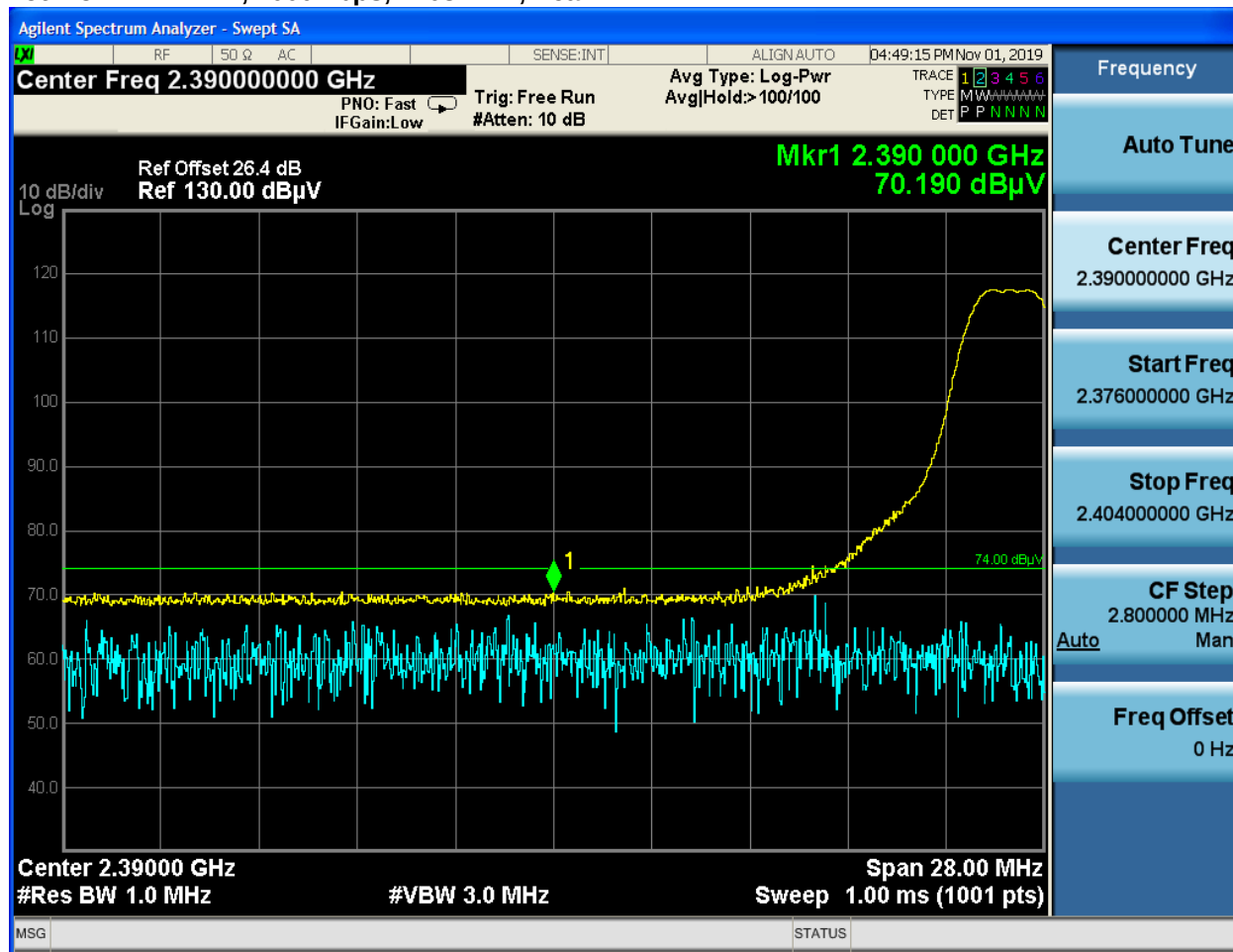
Plot 4-5: LBE, 1000 kbps, 2403 MHz, Peak
