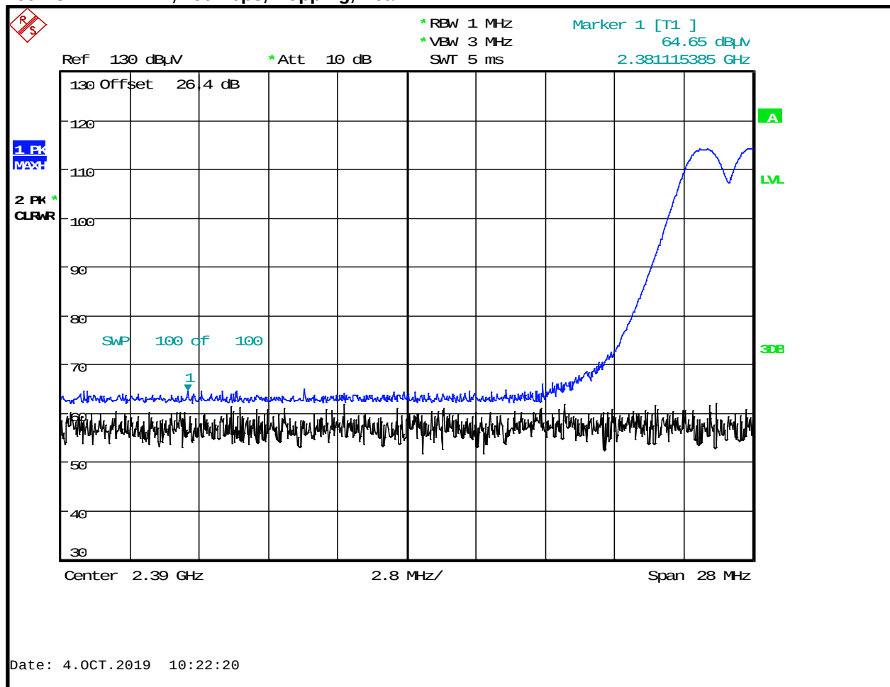
Plot 4-3: LBE, 250 kbps, Hopping, Peak
