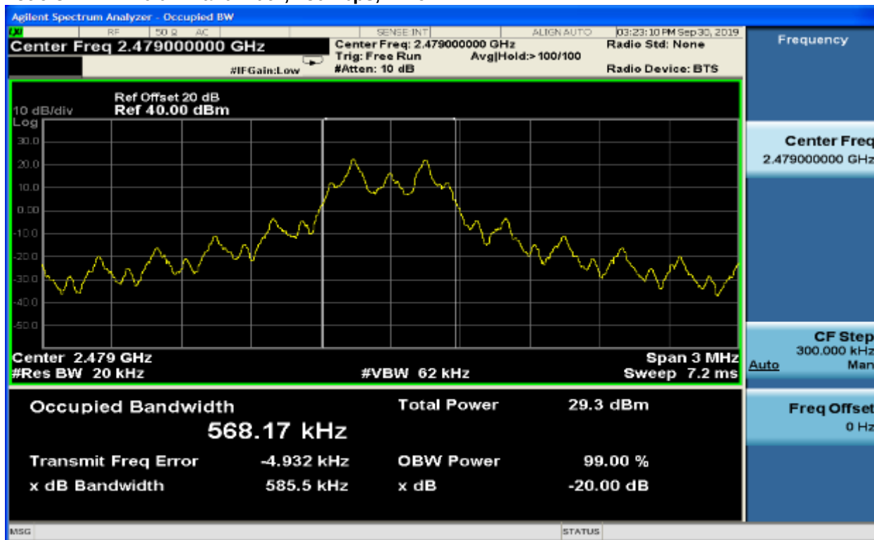
Plot 6-3: 20 dB Bandwidth, 250 kbps, 2479 MHz
