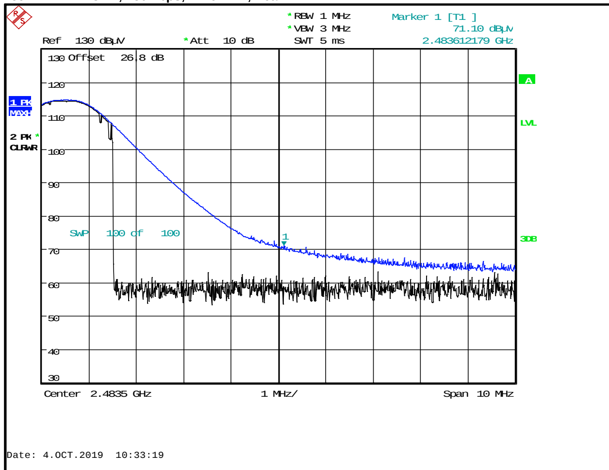
Plot 4-2: UBE, 250 kbps, 2479 MHz, Peak
