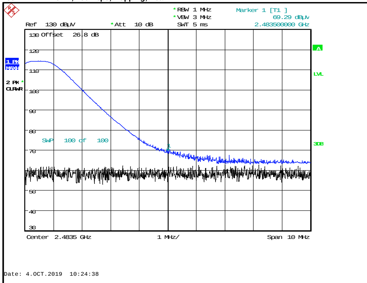
Plot 4-4: UBE, 250 kbps, Hopping, Peak
