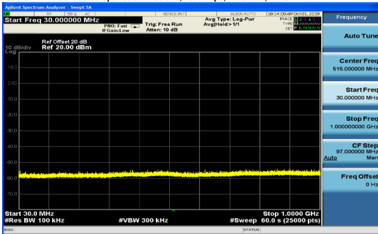
Plot 5-5: Conducted Spurious Emissions, 2000 kbps, 2440 MHz, < 1 GHz
