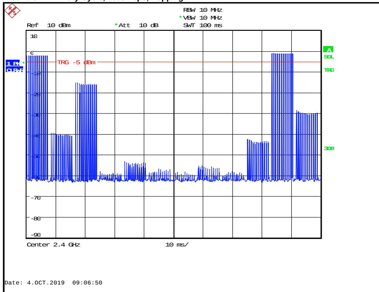
Plot 10-3: Duty Cycle, 2000 kbps, Hopping
