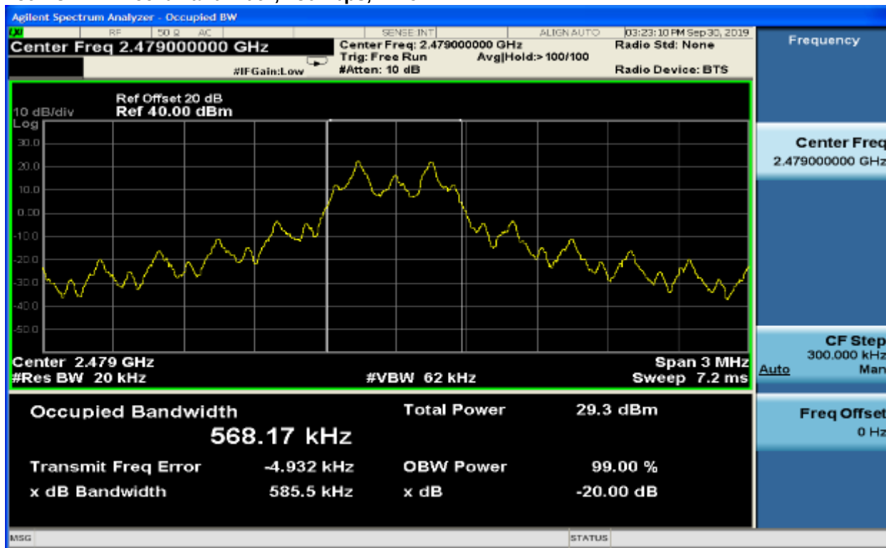
Plot 7-3: 99% Bandwidth, 250 kbps, 2479 MHz
