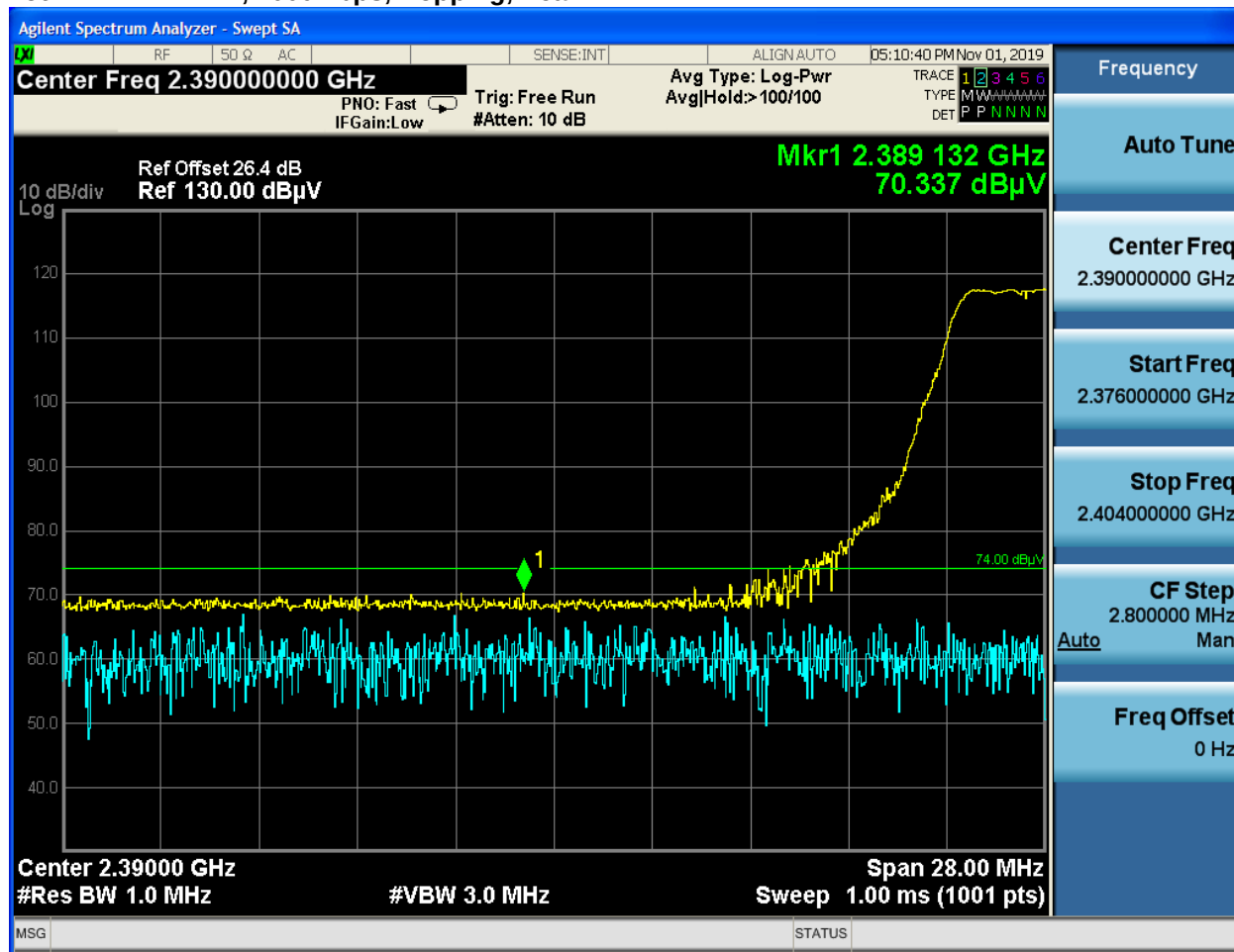
Plot 4-11: LBE, 2000 kbps, Hopping, Peak
