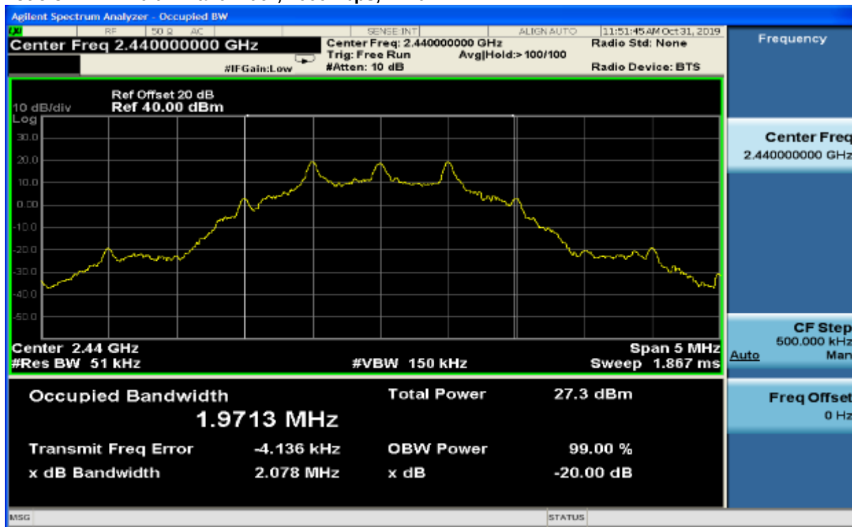
Plot 6-5: 20 dB Bandwidth, 1000 kbps, 2440 MHz
