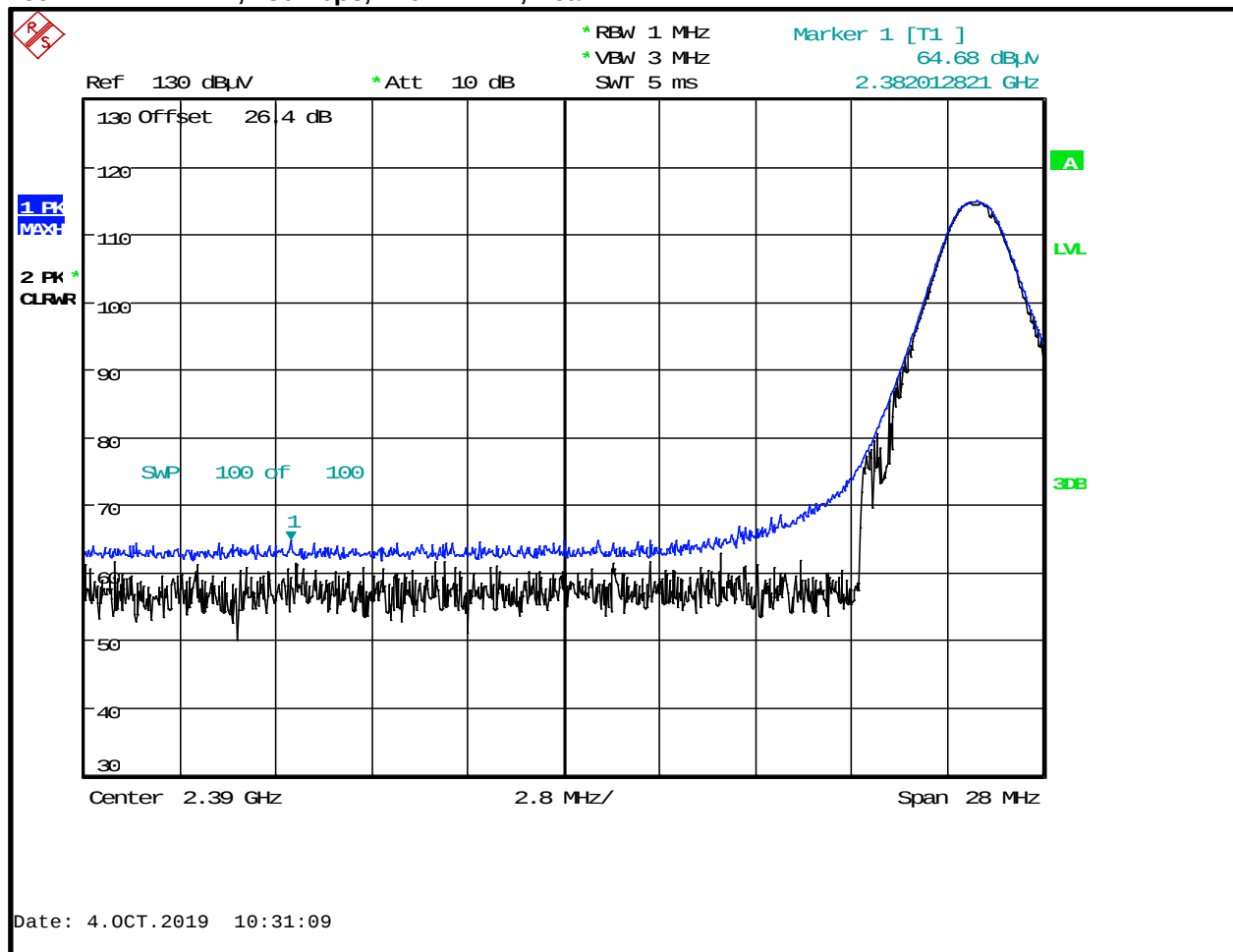
Plot 4-1: LBE, 250 kbps, 2402.2 MHz, Peak
